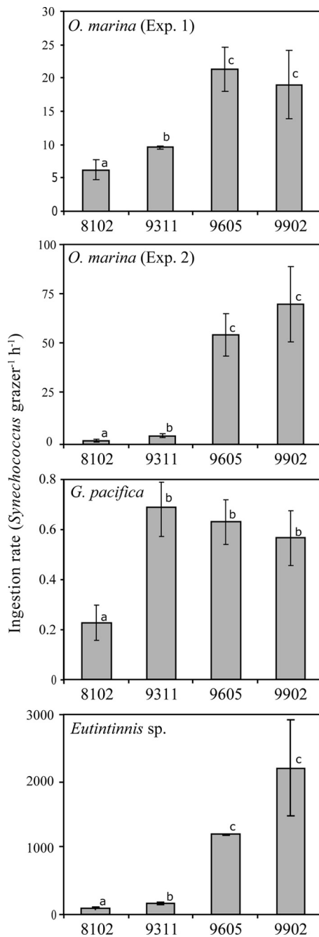
FIG. 1. Mean rates ( \pm SE) of ingestion of different Synechococcus isolates recorded for the four grazing experiments conducted with O. marina , G. pacifica , and Eutintinnis sp. Means sharing the same letter are statistically indistinguishable (Tukey-Kramer HSD, \alpha = 0.05 ).
