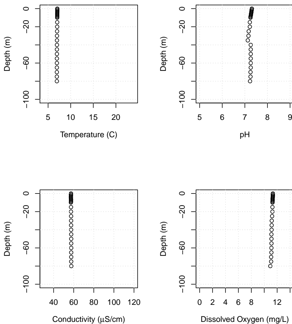
Figure B19: Lake Whatcom water column profiles showing temperature, pH, conductivity, and dissolved oxygen for Site 3, February 6, 2018.
