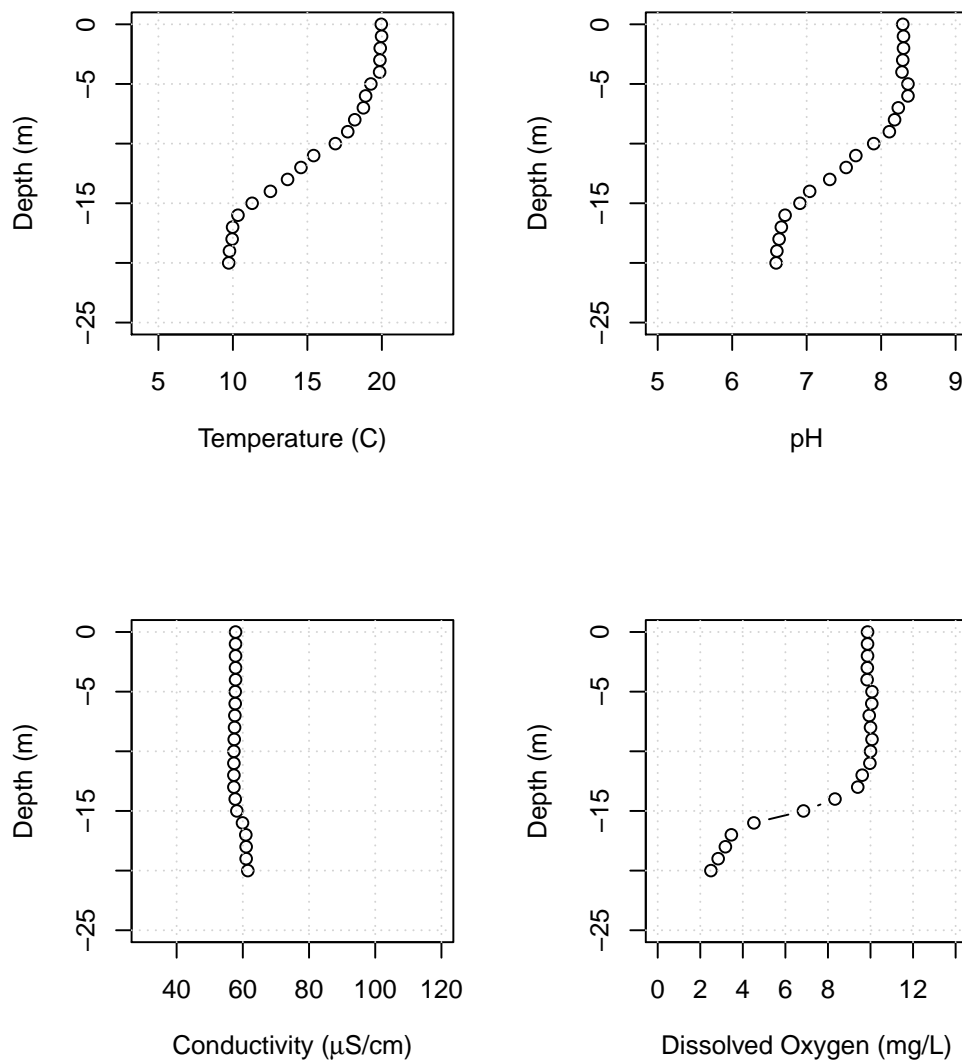
Figure B37: Lake Whatcom water column profiles showing temperature, pH, conductivity, and dissolved oxygen for Site 2, July 12, 2018.
