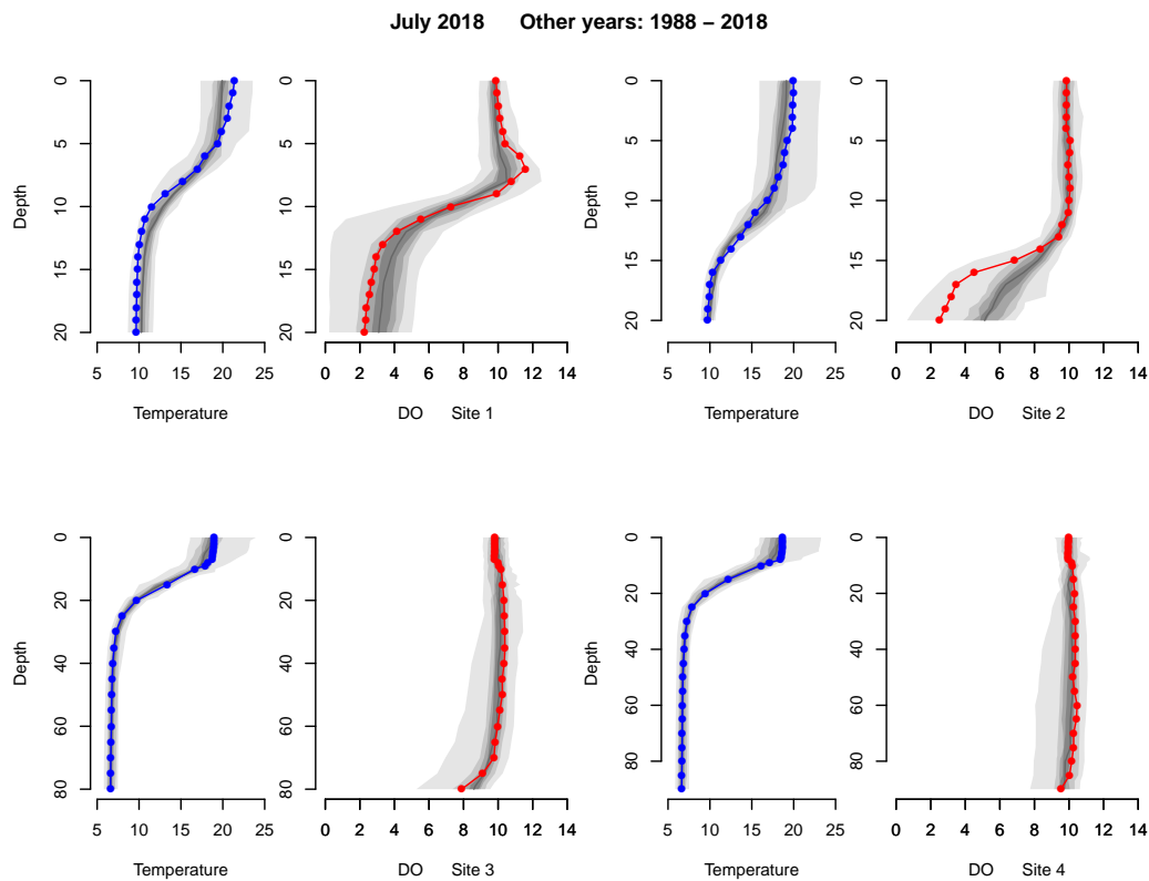
Figure 2.8: July 2018 temperature (-●-) and dissolved oxygen (-●-) profiles compared to historic ranges. The gradation in shading shows the approximate frequency of the 1988–2018 data.
