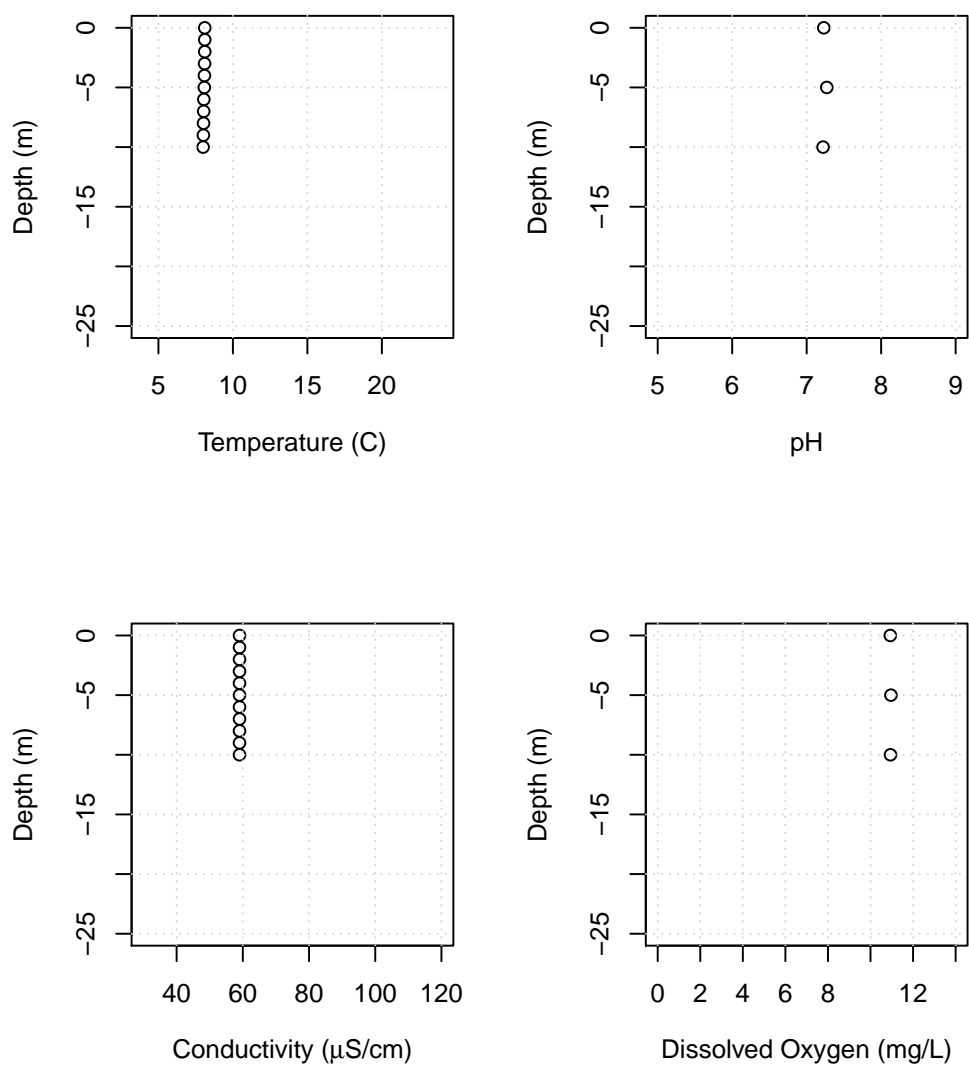
Figure B13: Lake Whatcom water column profiles showing temperature, pH, conductivity, and dissolved oxygen for the Intake, December 12, 2017. The dissolved oxygen and pH values were measured from discrete samples due to failure of the YSI oxygen and pH probes.
