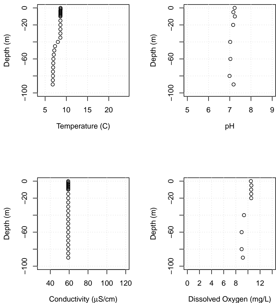
Figure B15: Lake Whatcom water column profiles showing temperature, pH, conductivity, and dissolved oxygen for Site 4, December 6, 2017. The dissolved oxygen and pH values were measured from discrete samples due to failure of the YSI oxygen and pH probes.
