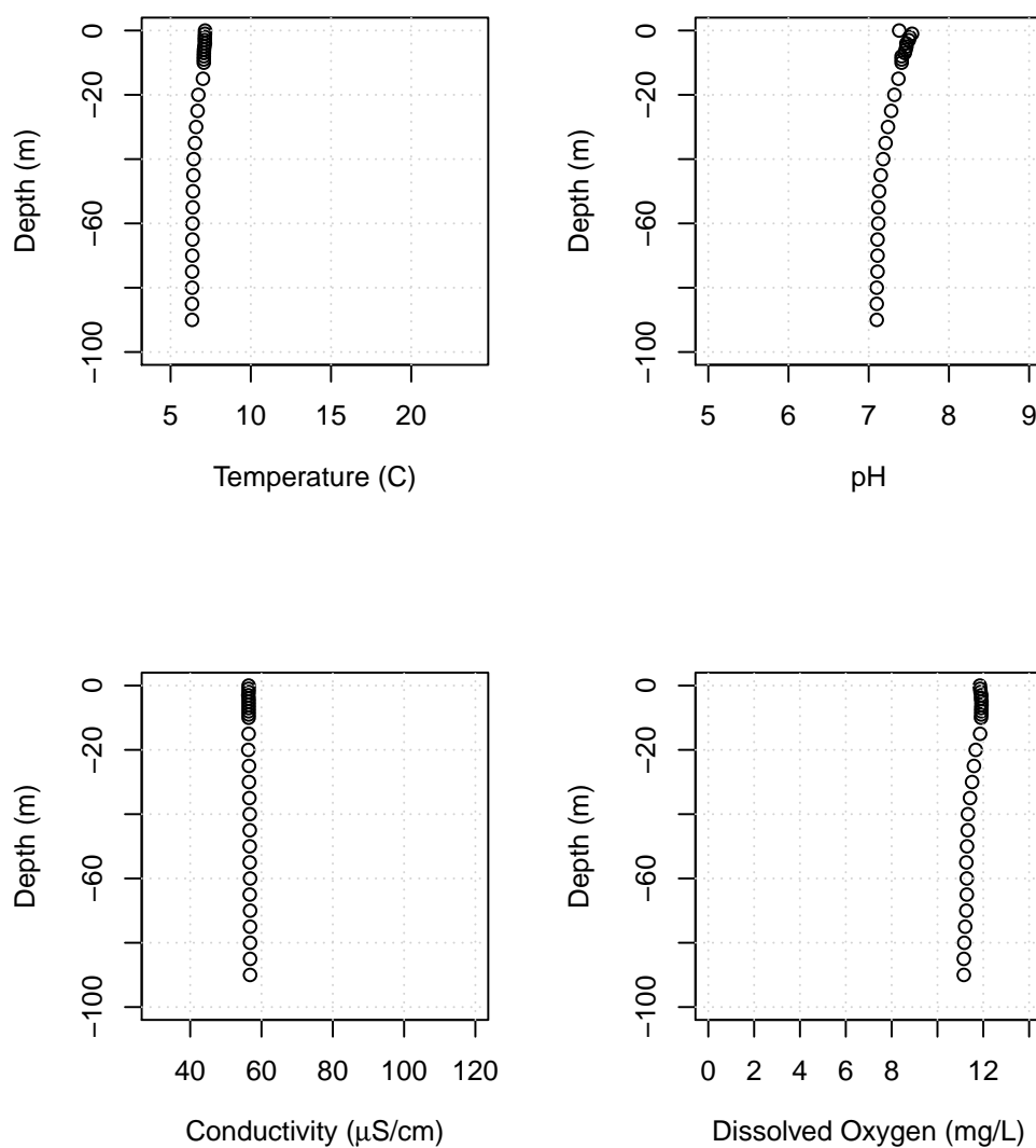
Figure B25: Lake Whatcom water column profiles showing temperature, pH, conductivity, and dissolved oxygen for Site 4, April 3, 2018.
