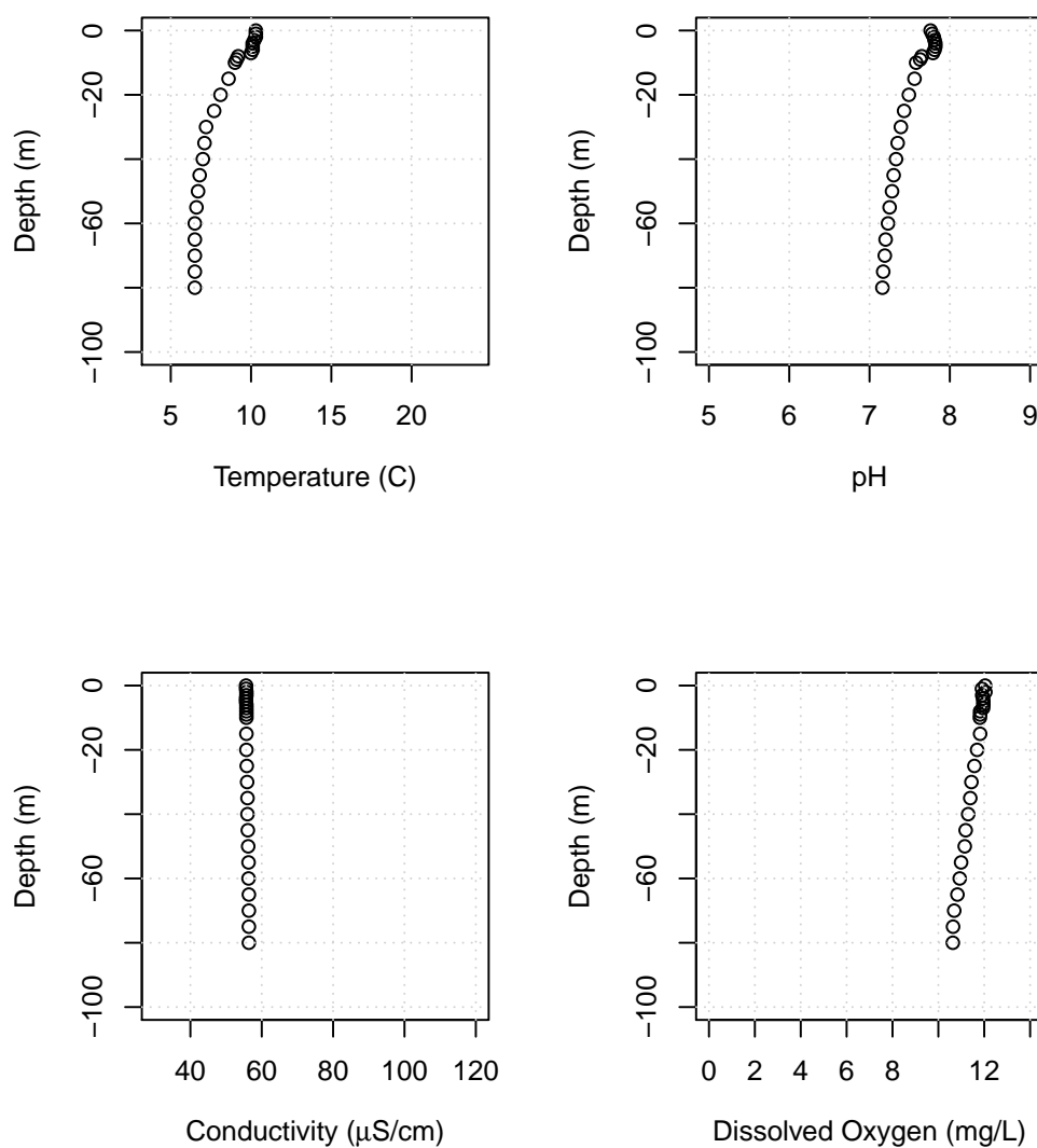
Figure B29: Lake Whatcom water column profiles showing temperature, pH, conductivity, and dissolved oxygen for Site 3, May 1, 2018.
