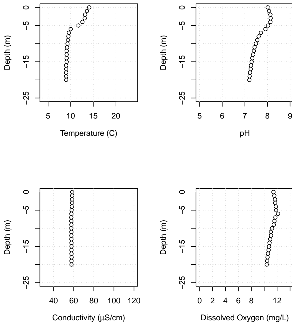
Figure B26: Lake Whatcom water column profiles showing temperature, pH, conductivity, and dissolved oxygen for Site 1, May 3, 2018.
