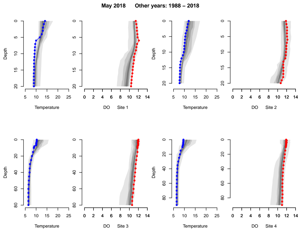
Figure 2.6: May 2018 temperature (-●-) and dissolved oxygen (-●-) profiles compared to historic ranges. The gradation in shading shows the approximate frequency of the 1988–2018 data.
