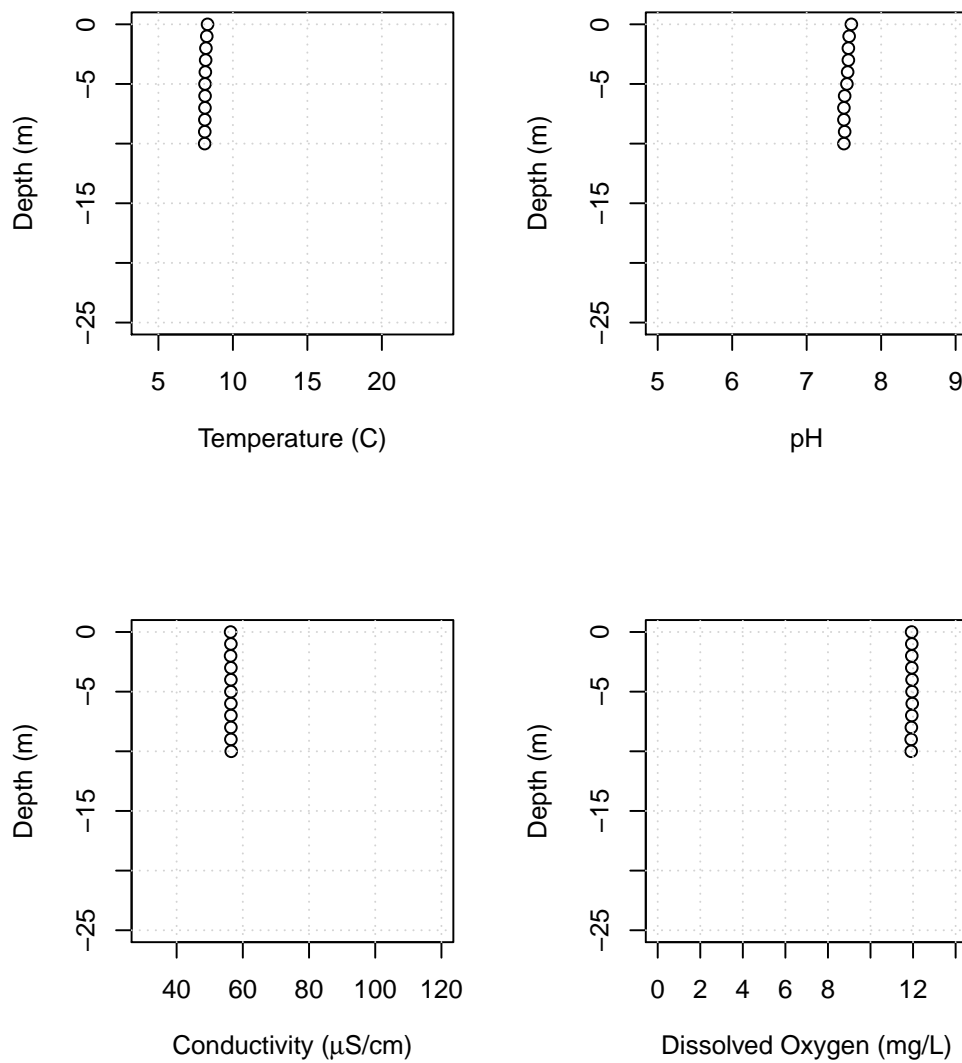
Figure B23: Lake Whatcom water column profiles showing temperature, pH, conductivity, and dissolved oxygen for the Intake, April 12, 2018.
