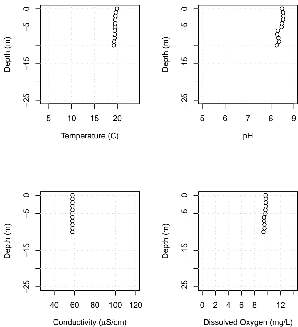
Figure B48: Lake Whatcom water column profiles showing temperature, pH, conductivity, and dissolved oxygen for the Intake, September 6, 2018.
