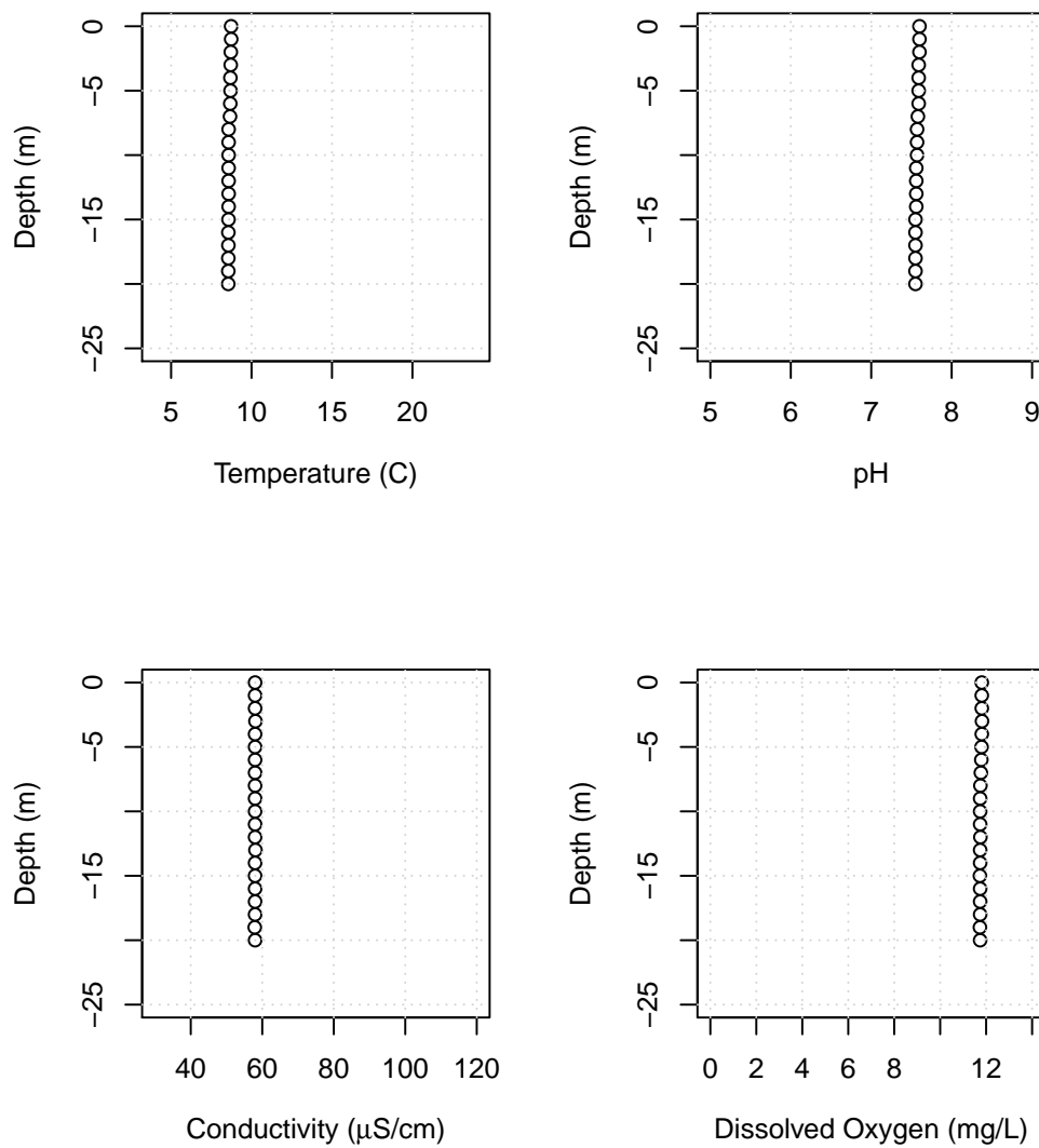
Figure B21: Lake Whatcom water column profiles showing temperature, pH, conductivity, and dissolved oxygen for Site 1, April 12, 2018.
