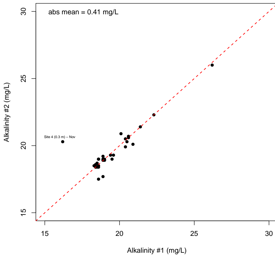
Figure C31: Alkalinity field duplicates for the 2017/2018 Lake Whatcom monitoring program (lake samples). Diagonal reference line shows 1:1 relationship.
