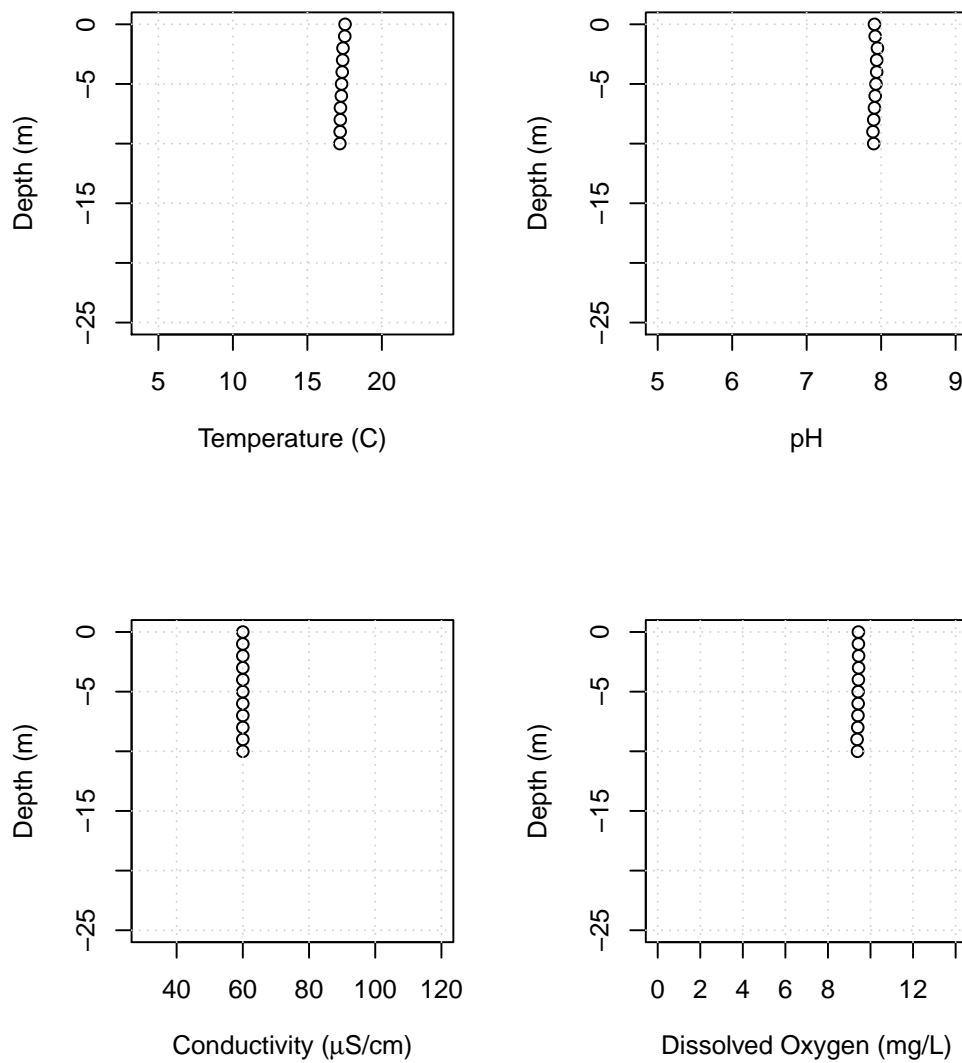
Figure B3: Lake Whatcom water column profiles showing temperature, pH, conductivity, and dissolved oxygen for the Intake, October 5, 2017.
