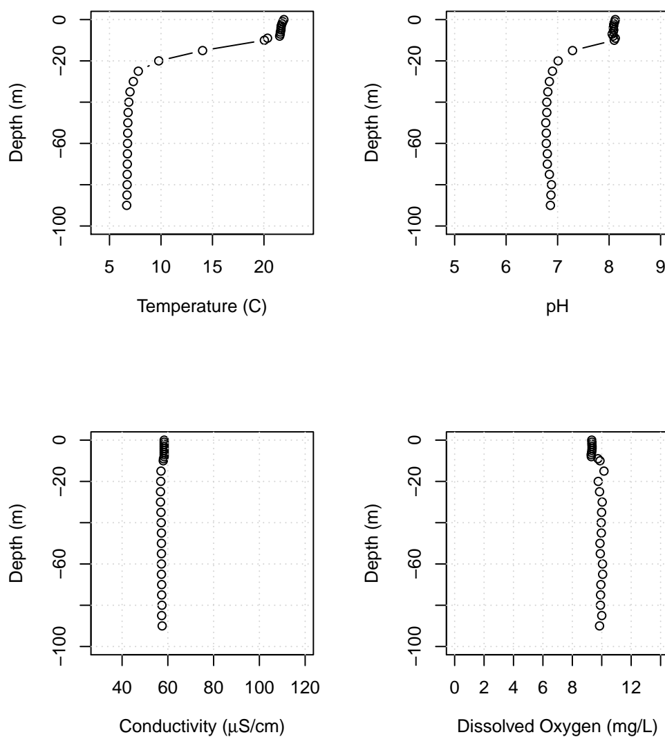
Figure B45: Lake Whatcom water column profiles showing temperature, pH, conductivity, and dissolved oxygen for Site 4, August 7, 2018.
