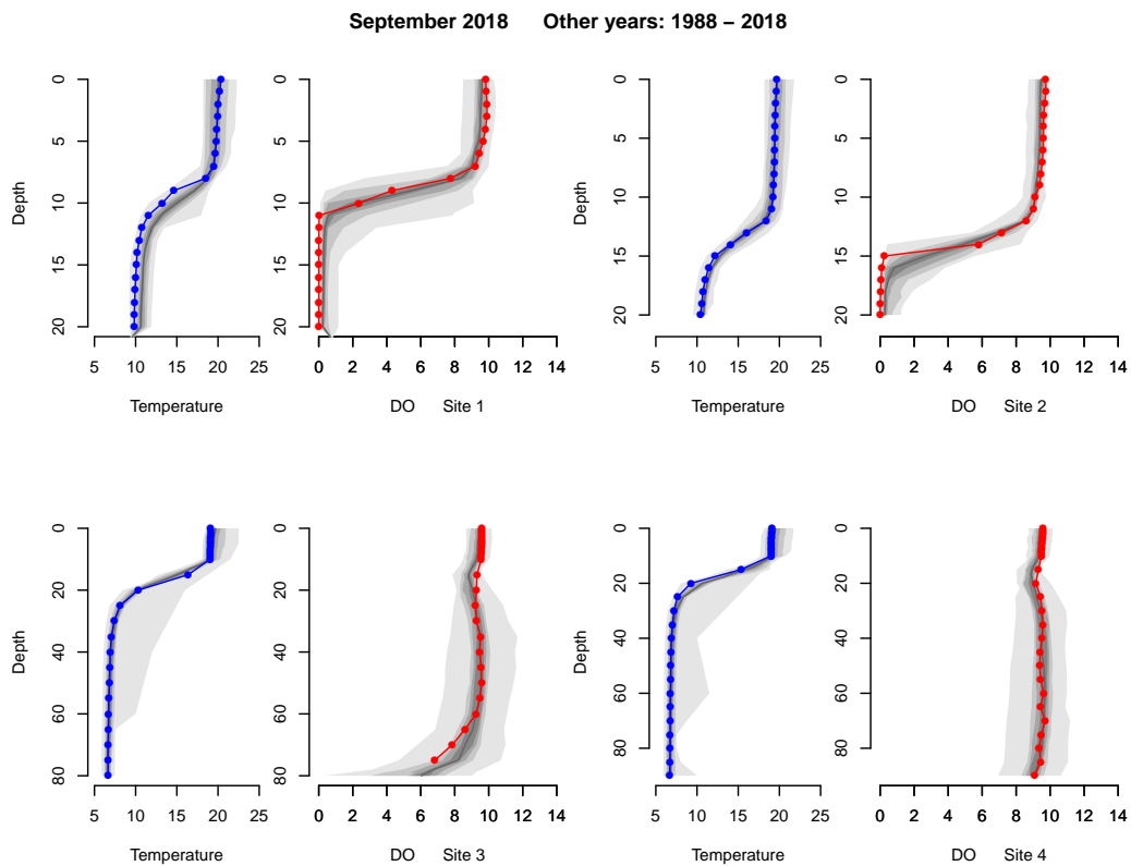
Figure 2.10: September 2018 temperature (—●—) and dissolved oxygen (—●—) profiles compared to historic ranges. The gradation in shading shows the approximate frequency of the 1988–2018 data.
