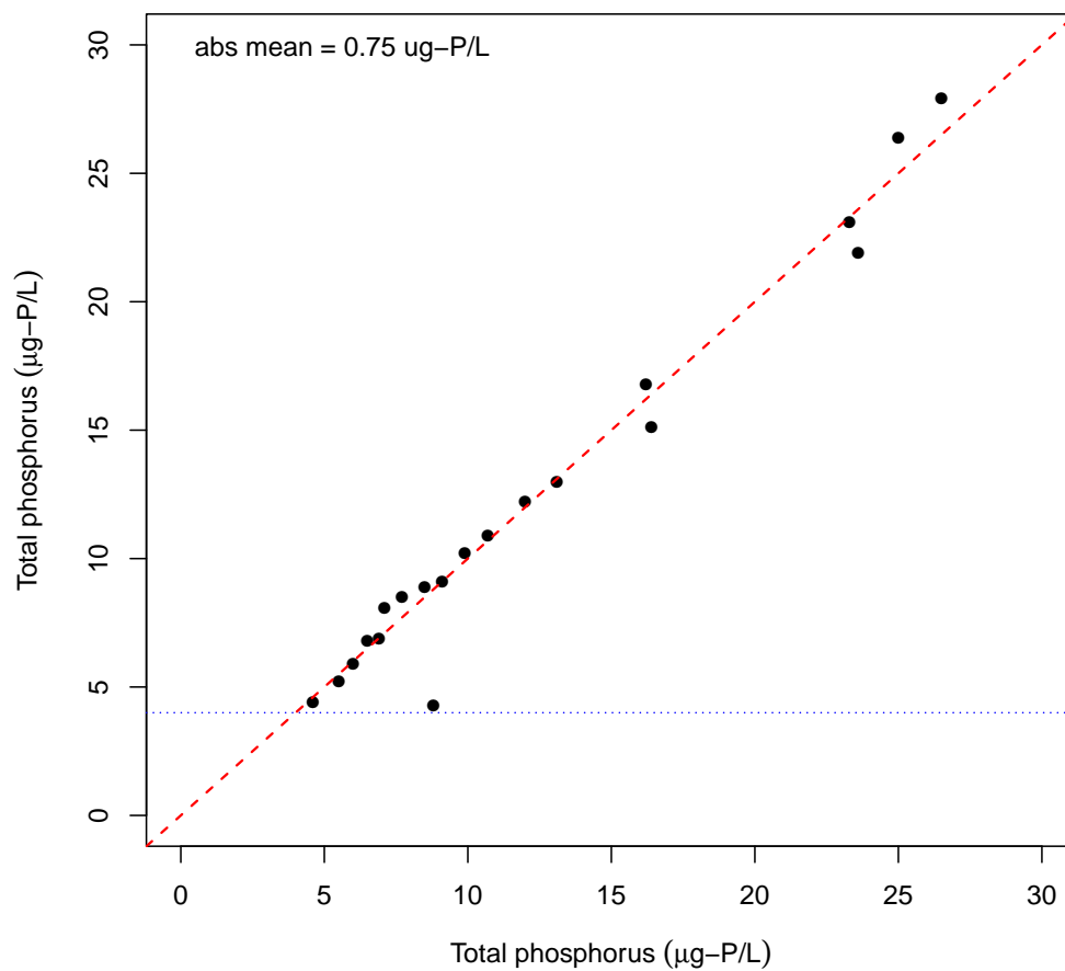
Figure C46: Phosphorus (total) field duplicates for the 2017/2018 Lake Whatcom monitoring program (tributary samples). Diagonal reference line shows 1:1 relationship; horizontal reference line shows current detection limit.
