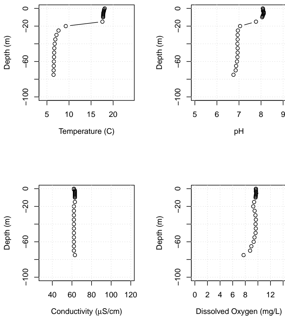
Figure B4: Lake Whatcom water column profiles showing temperature, pH, conductivity, and dissolved oxygen for Site 3, October 3, 2017.
