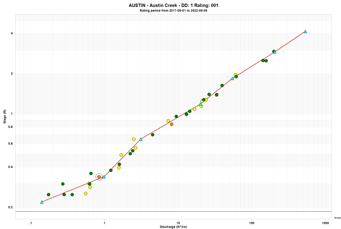
Figure 4.3: Aquarius rating curve for Austin Creek. The triangles ( \triangle ) show the fitted rating curve for WY2018. The circles show data collected in WY2018 ( \bullet ), WY2017 ( \circ ), WY2016 ( \circ ).
