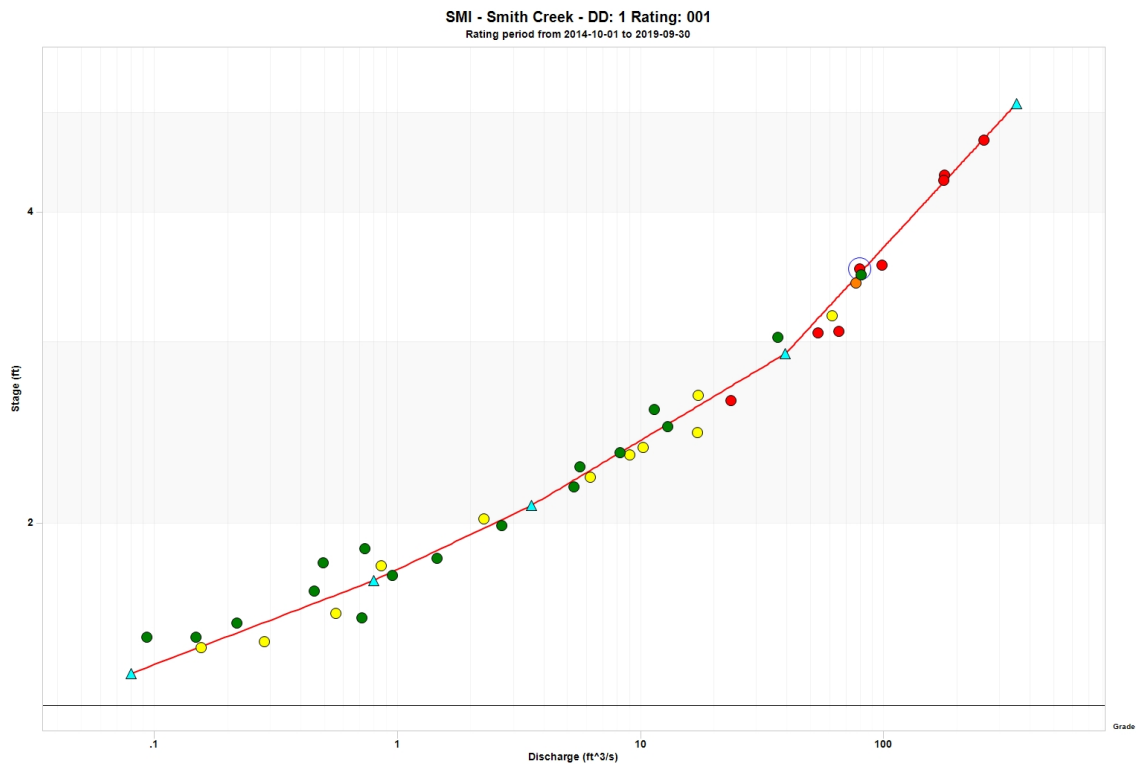
Figure 4.4: Aquarius rating curve for Smith Creek. The triangles ( \Delta ) show the fitted rating curve for WY2018. The circles show data collected in WY2018 ( \bullet ), WY2017 ( \circ ), WY2016 ( \circ ). The red circles ( \bullet ) show data collected prior to WY2016 that were used for the rating curve because they help define the high end of the rating curve.
