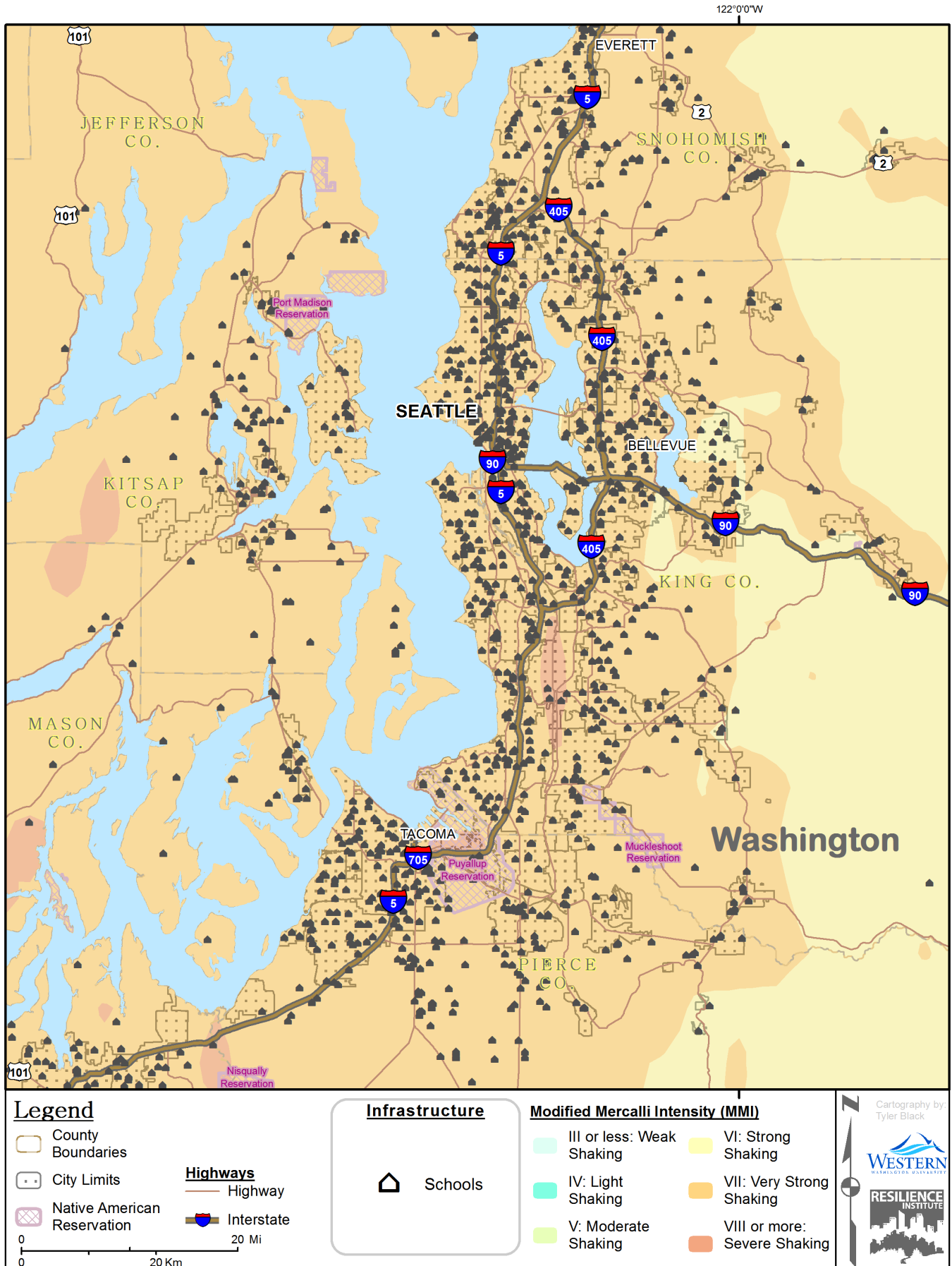
Figure 91. Seattle-Tacoma metro schools in relation to shaking intensity
