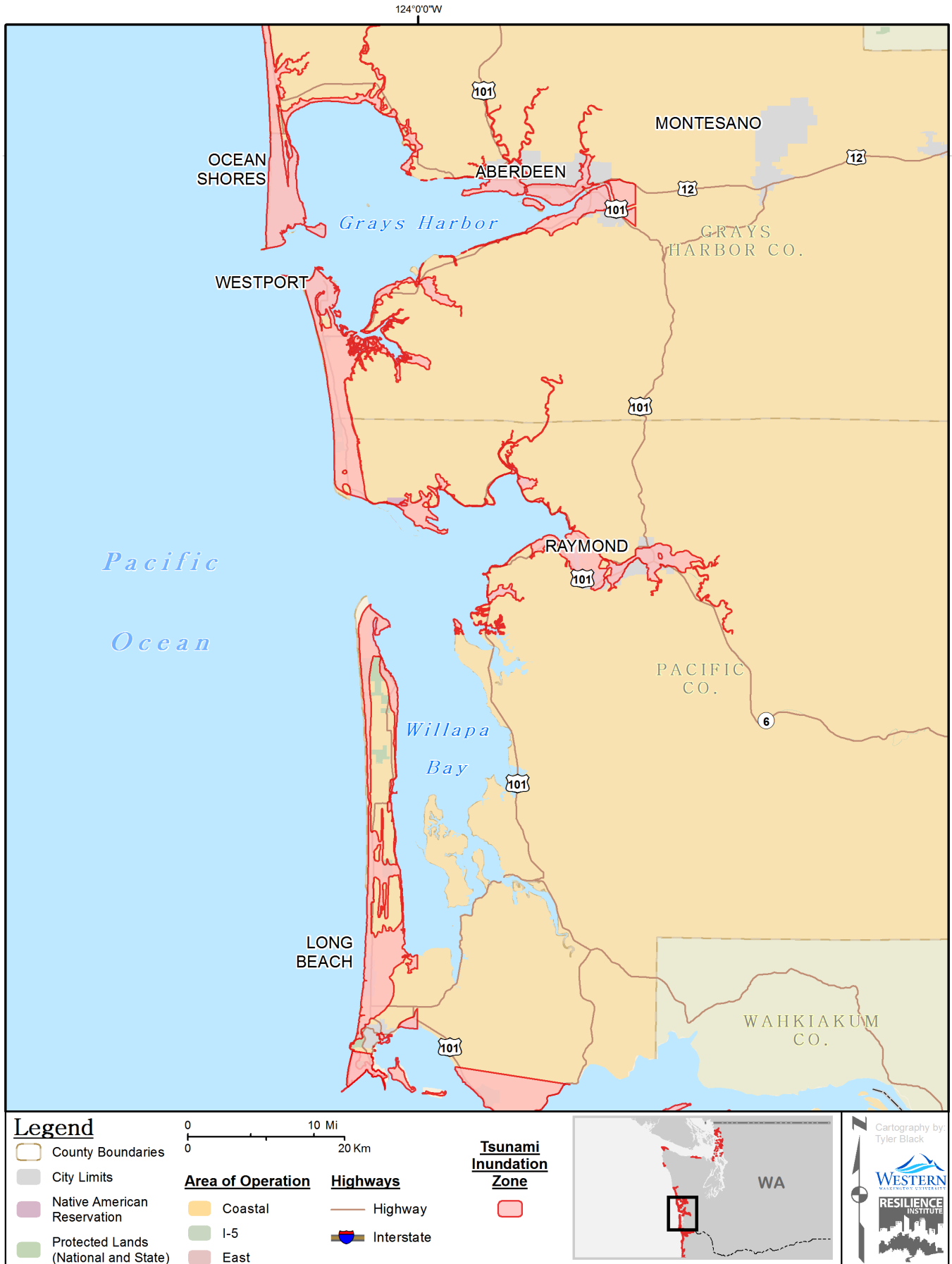
Figure 10. Tsunami inundation zone along the coast of Grays Harbor and Willapa Bay, Washington
