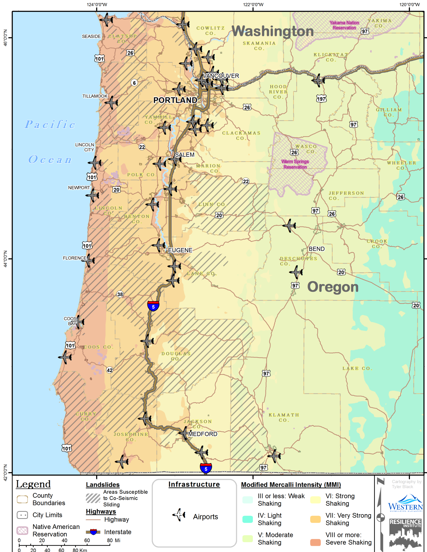
Figure 41. Oregon airports in relation to shaking intensity and landslide potential
