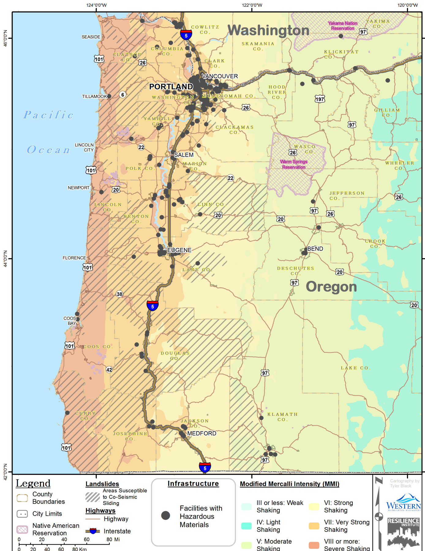
Figure 103. Oregon facilities with hazardous material in relation to shaking intensity and landslide potential
