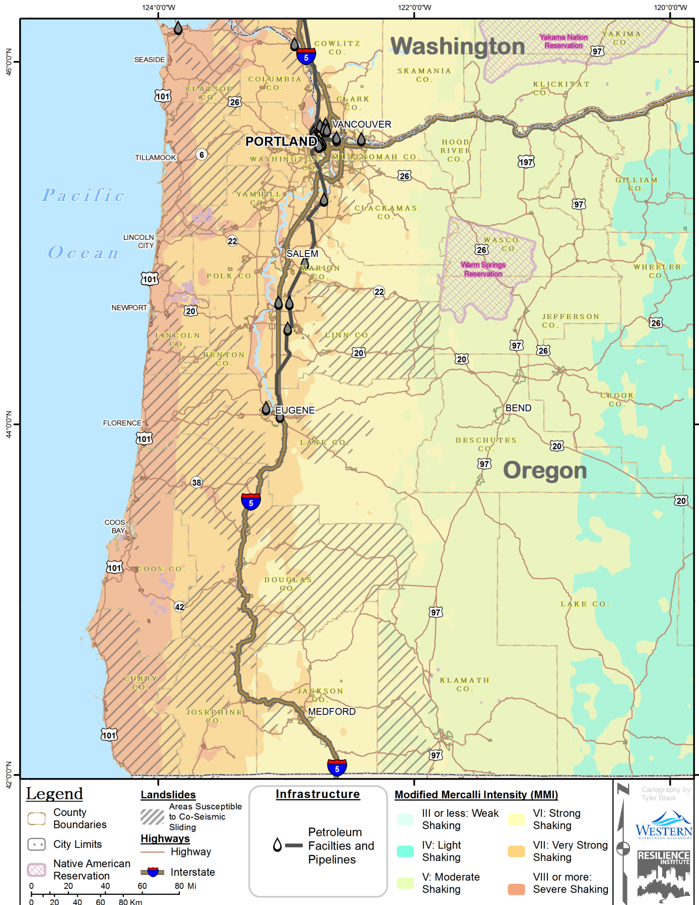
Figure 64. Oregon refined fuel facilities and pipelines in relation to shaking intensity and landslide potential
