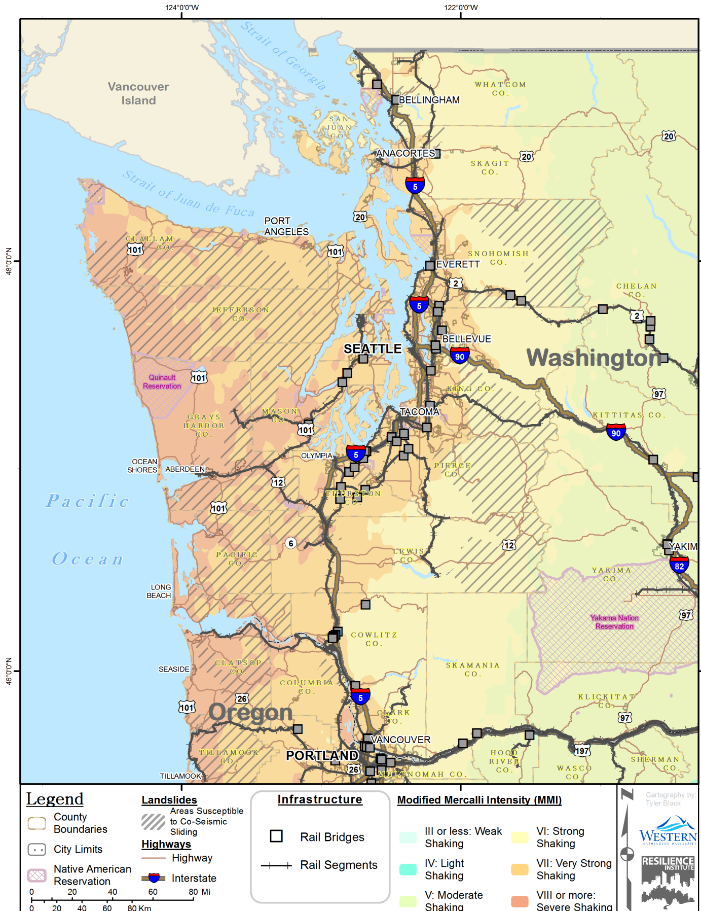
Figure 45. Washington railway track and bridges in relation to shaking intensity and landslide potential
