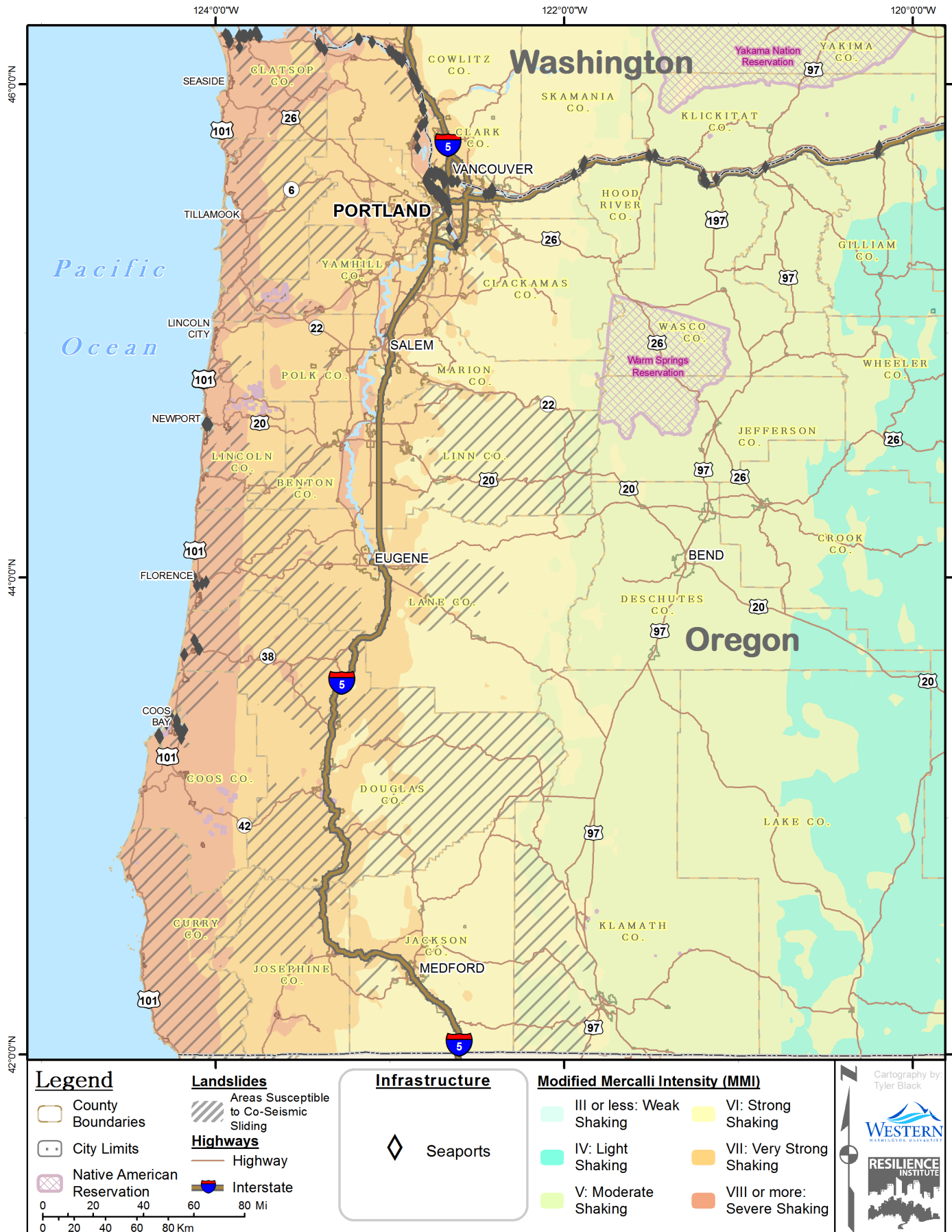
Figure 55. Oregon ports in relation to shaking intensity and landslide potential
