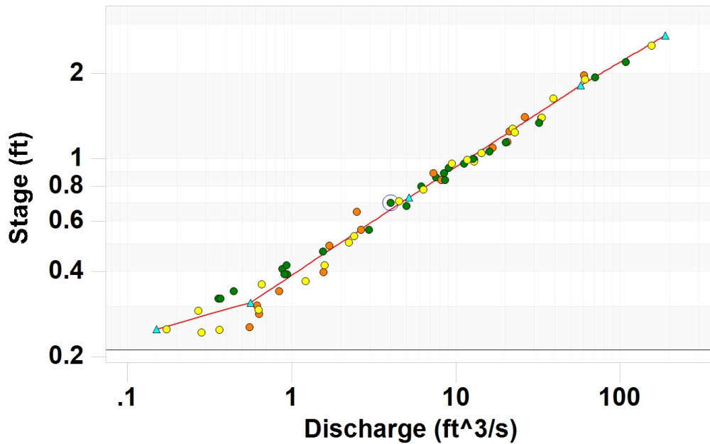
Figure 4.3: Aquarius rating curve for Austin Creek. The triangles ( \Delta ) show the fitted rating curve for WY2019. The circles show data collected in WY2019 ( \bullet ), WY2018 ( \circ ), WY2017 ( \circ ).
