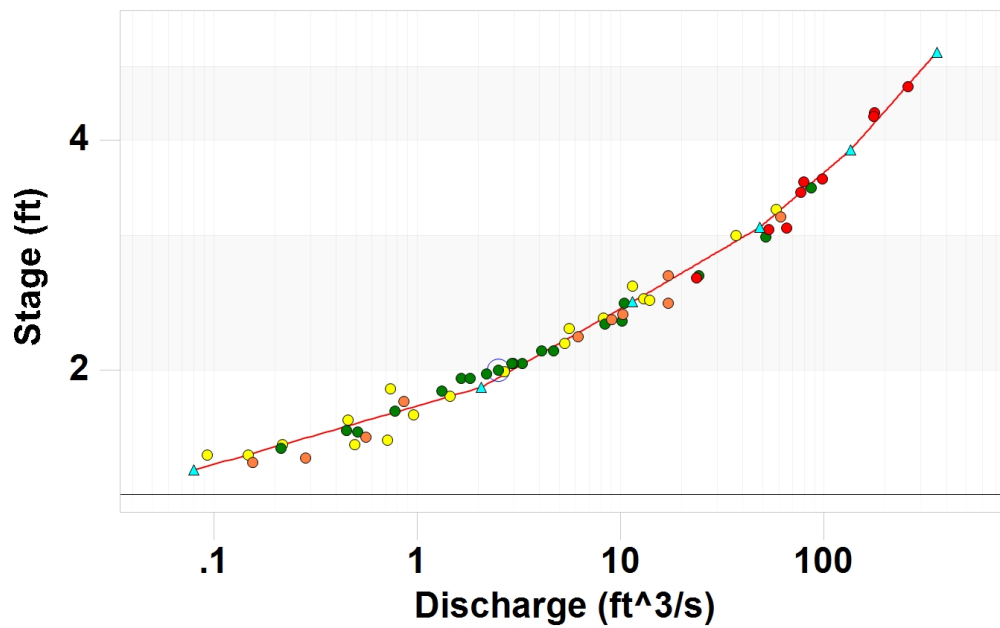
Figure 4.4: Aquarius rating curve for Smith Creek. The triangles ( \Delta ) show the fitted rating curve for WY2019. The circles show data collected in WY2019 ( \bullet ), WY2018 ( \circ ), WY2017 ( \circ ). The red circles ( \bullet ) show data collected prior to WY2017 that were used for the rating curve because they help define the high end of the rating curve.
