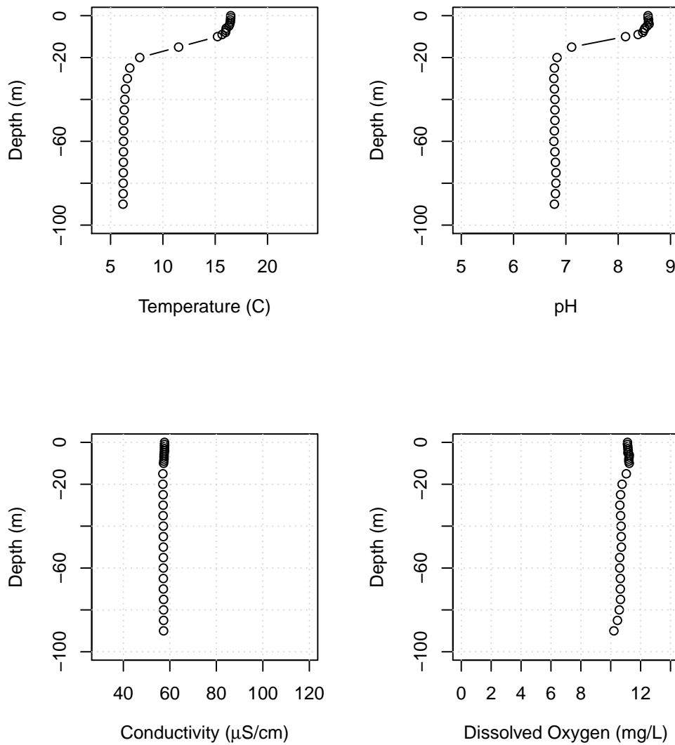
Figure B35: Lake Whatcom water column profiles showing temperature, pH, conductivity, and dissolved oxygen for Site 4, June 10, 2019.
