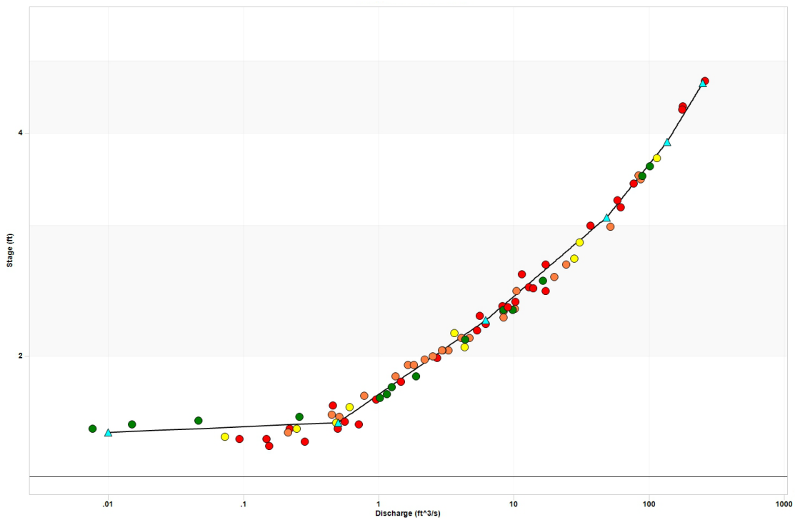
Figure 4.4: Aquarius rating curve for Smith Creek. The triangles (▲) show the fitted rating curve for WY2021. The circles show data collected in WY2021 (●), WY2020 (●), WY2019 (●). The red circles (●) show data collected prior to WY2019 that were used for the rating curve because they help define the high end of the rating curve.
