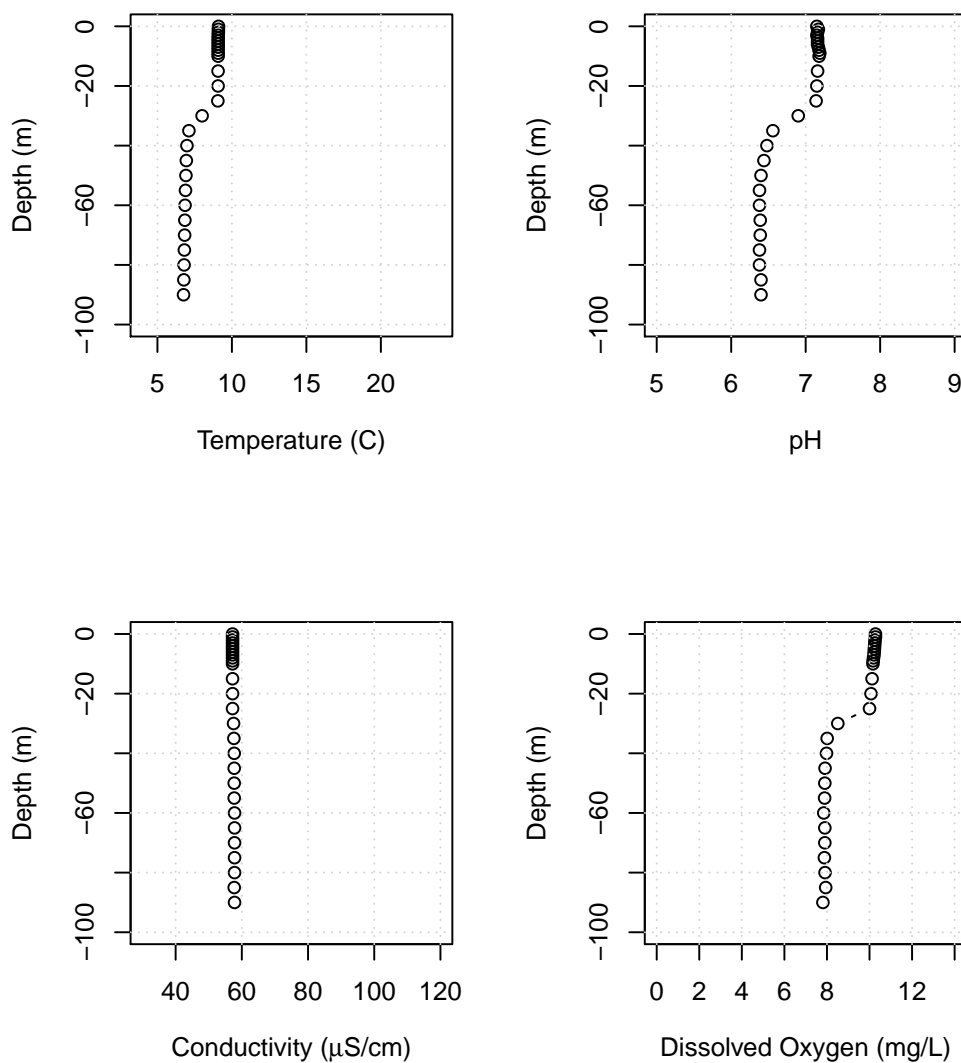
Figure B15: Lake Whatcom water column profiles showing temperature, pH, conductivity, and dissolved oxygen for Site 4, December 2, 2020.
