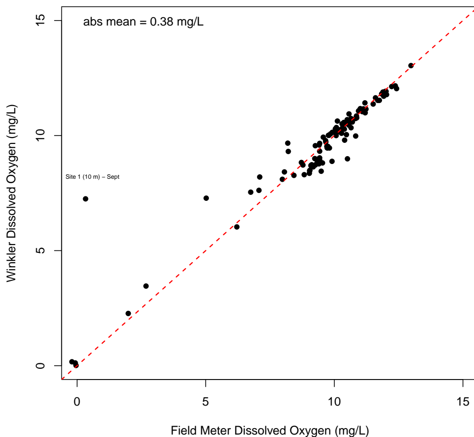
Figure C35: Dissolved oxygen field duplicates for the 2020/2021 Lake Whatcom monitoring program (lake samples). Diagonal reference line shows 1:1 relationship. The labeled outlier was collected when extreme gradients were present. Field meter samples were collected at true depth; Winkler samples were measured in the laboratory from samples collected using a marked line, which will be slightly shallower than true depth. There was a systematic bias between the Winkler and field meter results, with the Winkler results \sim 0.5 mg/L lower than the field meter. This is within typical ranges for Winkler vs. field meter comparisons (Johengen, et al., 2016).
