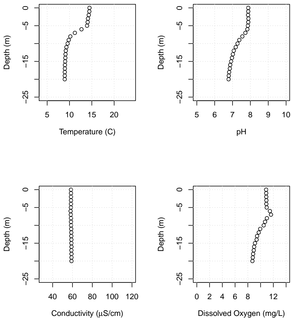
Figure B26: Lake Whatcom water column profiles showing temperature, pH, conductivity, and dissolved oxygen for Site 1, May 10, 2021.
