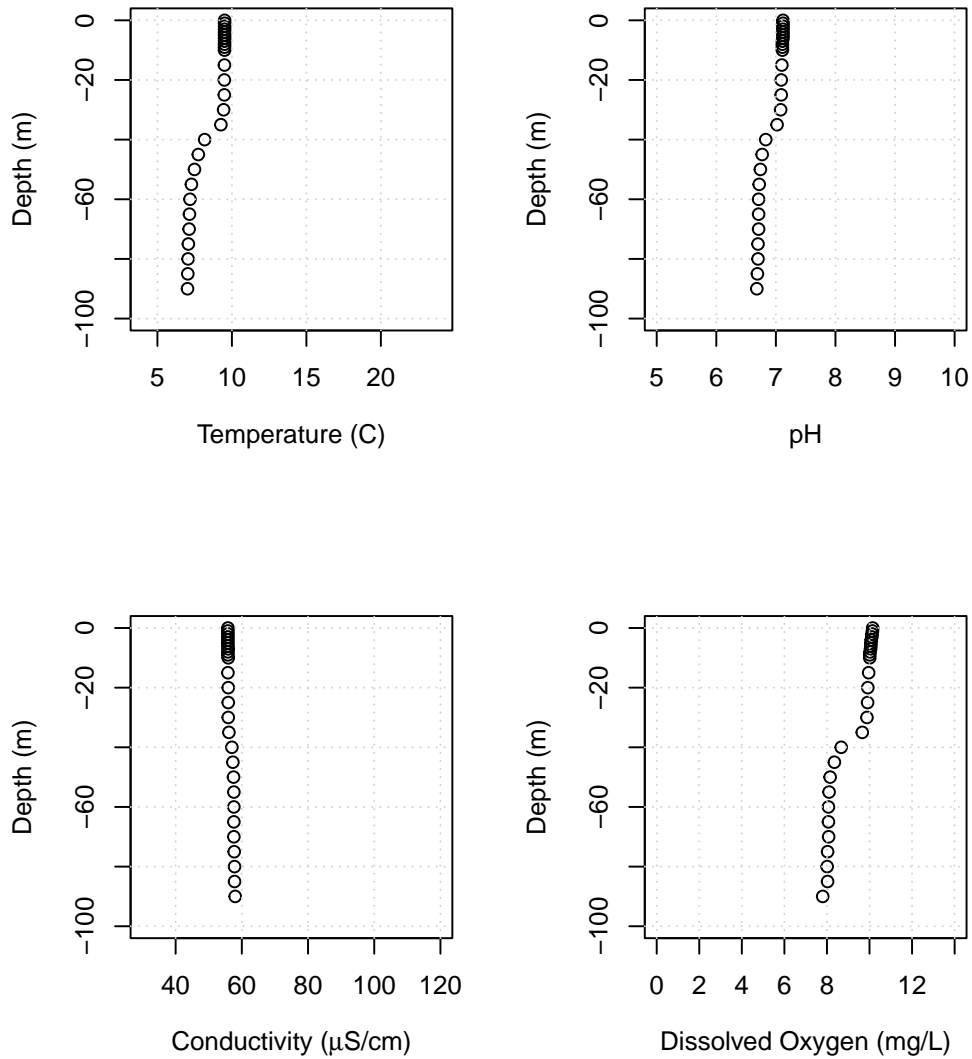
Figure B65: Lake Whatcom water column profiles showing temperature, pH, conductivity, and dissolved oxygen for Site 4, December 2, 2021.
