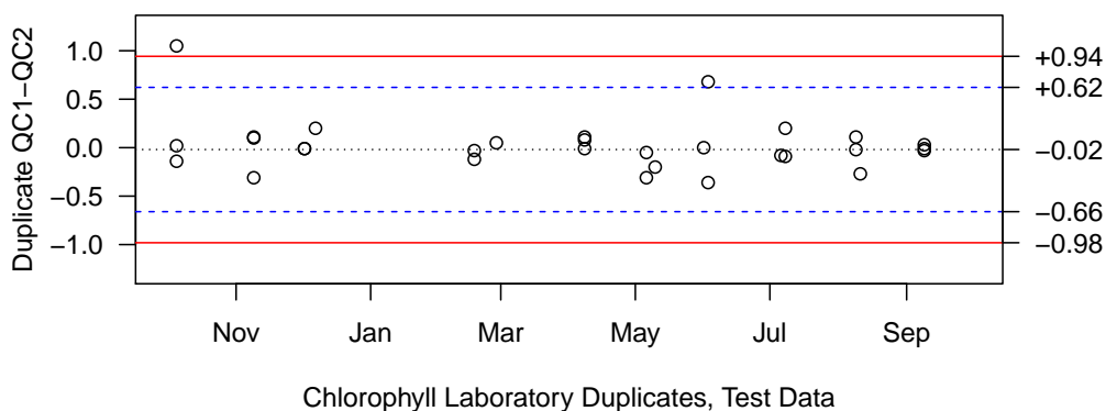
Figure C4: Chlorophyll laboratory duplicates for the Lake Whatcom monitoring program. Upper/lower acceptance limits ( \pm 2 std. dev. from mean pair difference) and upper/lower warning limits ( \pm 3 std. dev. from mean pair difference) were calculated based on the preceding two years of lab duplicate data.
