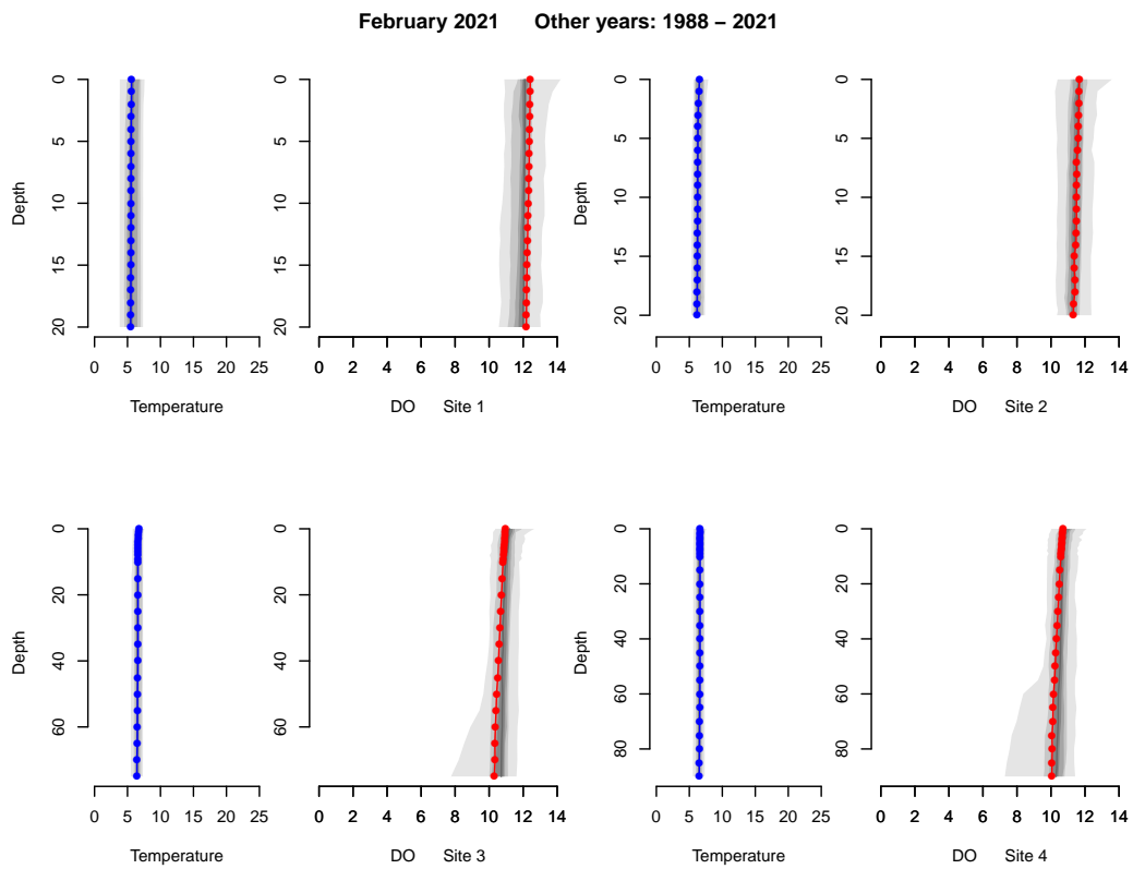
Figure 2.4: February 2021 temperature (-●-) and dissolved oxygen (-●-) profiles compared to historic ranges. The gradation in shading shows the approximate frequency of the 1988–2021 data.
