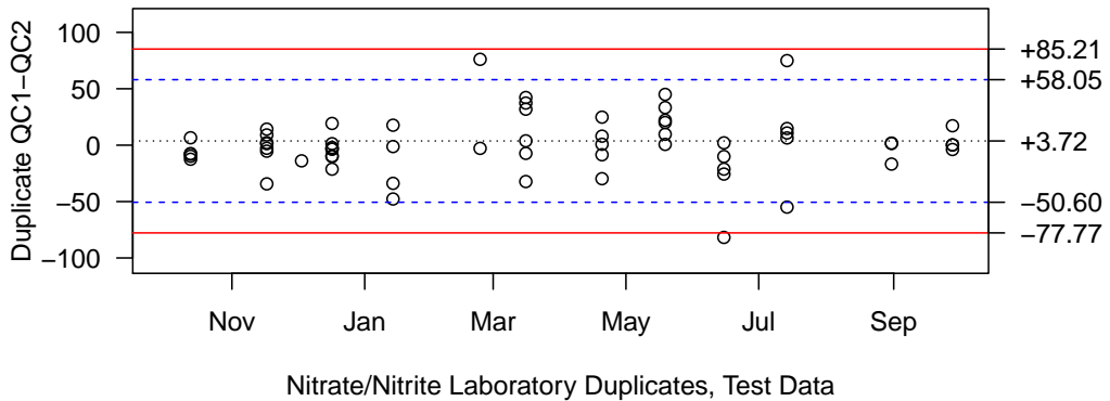
Figure C11: Nitrogen (nitrate/nitrite) laboratory duplicates for the Lake Whatcom monitoring program. Upper/lower acceptance limits ( \pm 2 std. dev. from mean pair difference) and upper/lower warning limits ( \pm 3 std. dev. from mean pair difference) were calculated based on the preceding two years of lab duplicate data.
