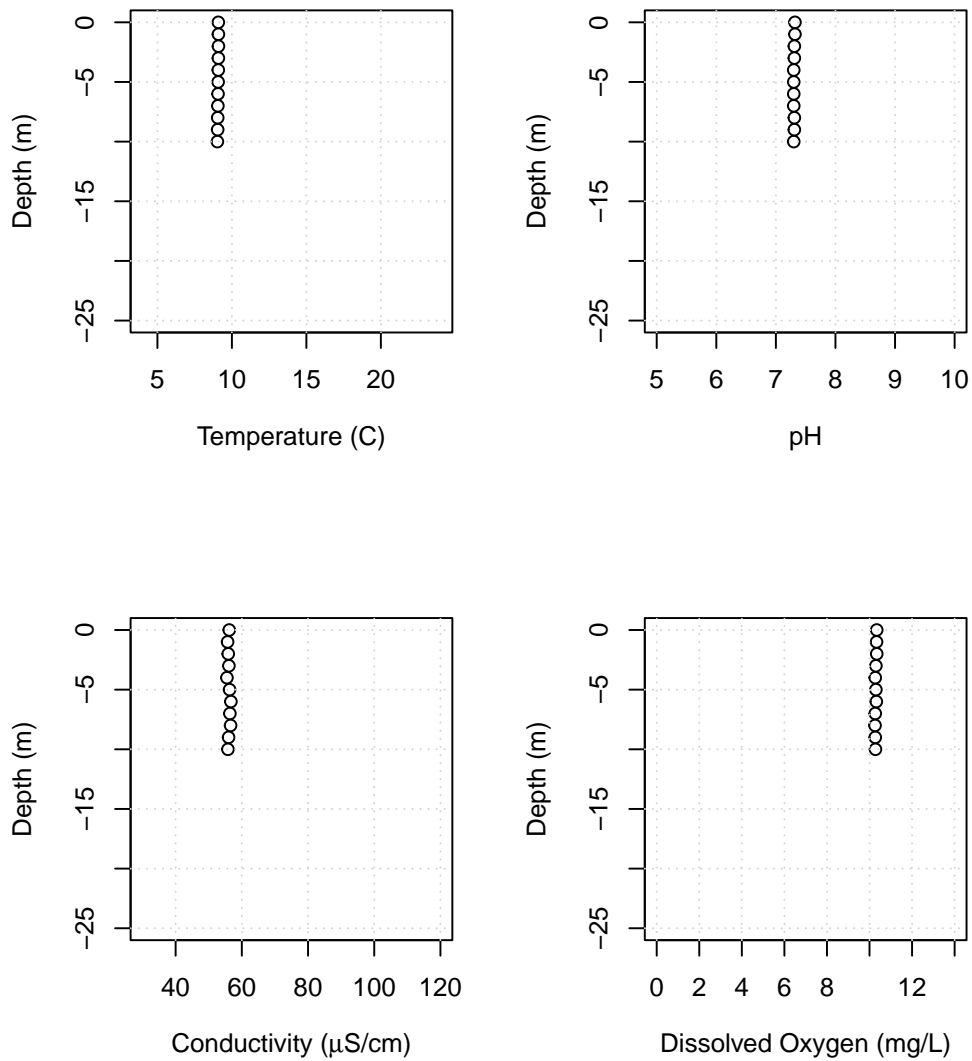
Figure B63: Lake Whatcom water column profiles showing temperature, pH, conductivity, and dissolved oxygen for the Intake, December 9, 2021.
