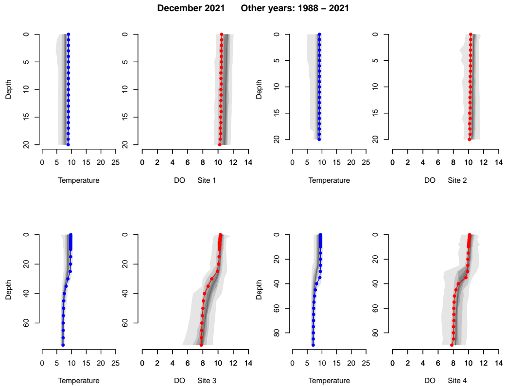
Figure 2.13: December 2021 temperature (-●-) and dissolved oxygen (-●-) profiles compared to historic ranges. The gradation in shading shows the approximate frequency of the 1988–2021 data. December 2021 is not part of the 2020/2021 sampling period, but were included to to provide information on the timing of destratification.
