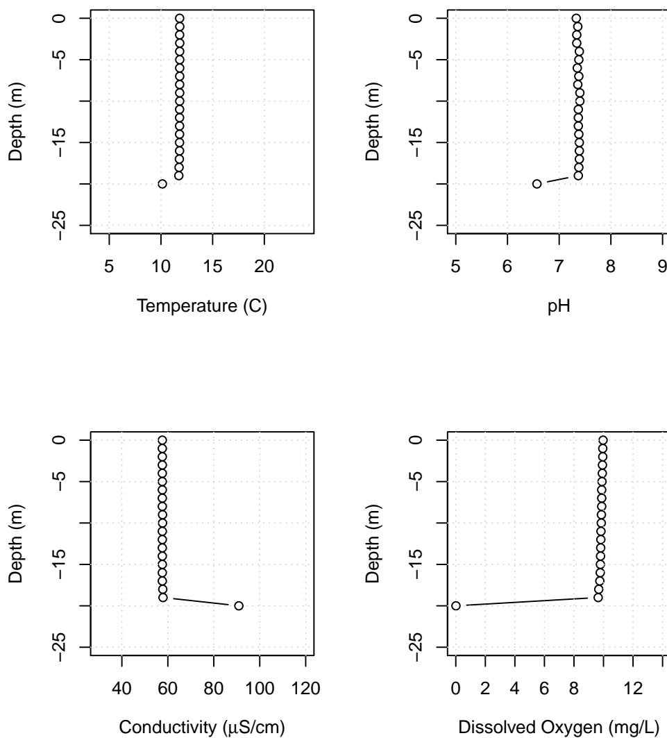
Figure B7: Lake Whatcom water column profiles showing temperature, pH, conductivity, and dissolved oxygen for Site 2, November 9, 2020.
