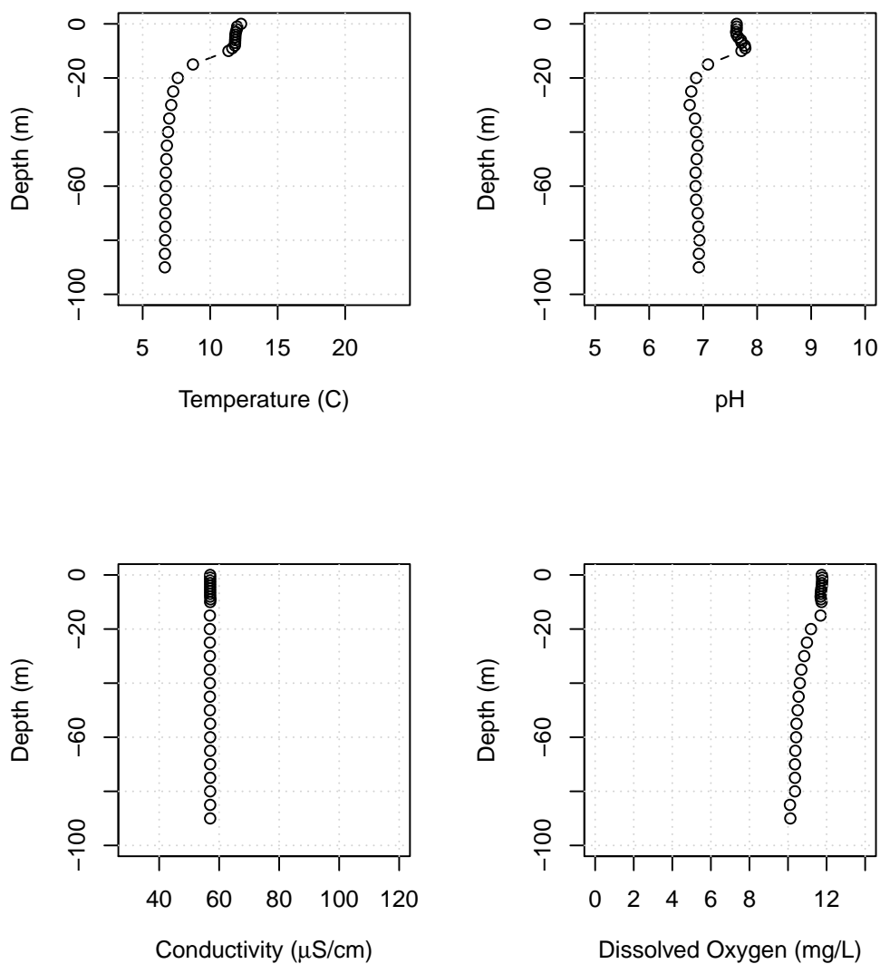
Figure B30: Lake Whatcom water column profiles showing temperature, pH, conductivity, and dissolved oxygen for Site 4, May 4, 2021.
