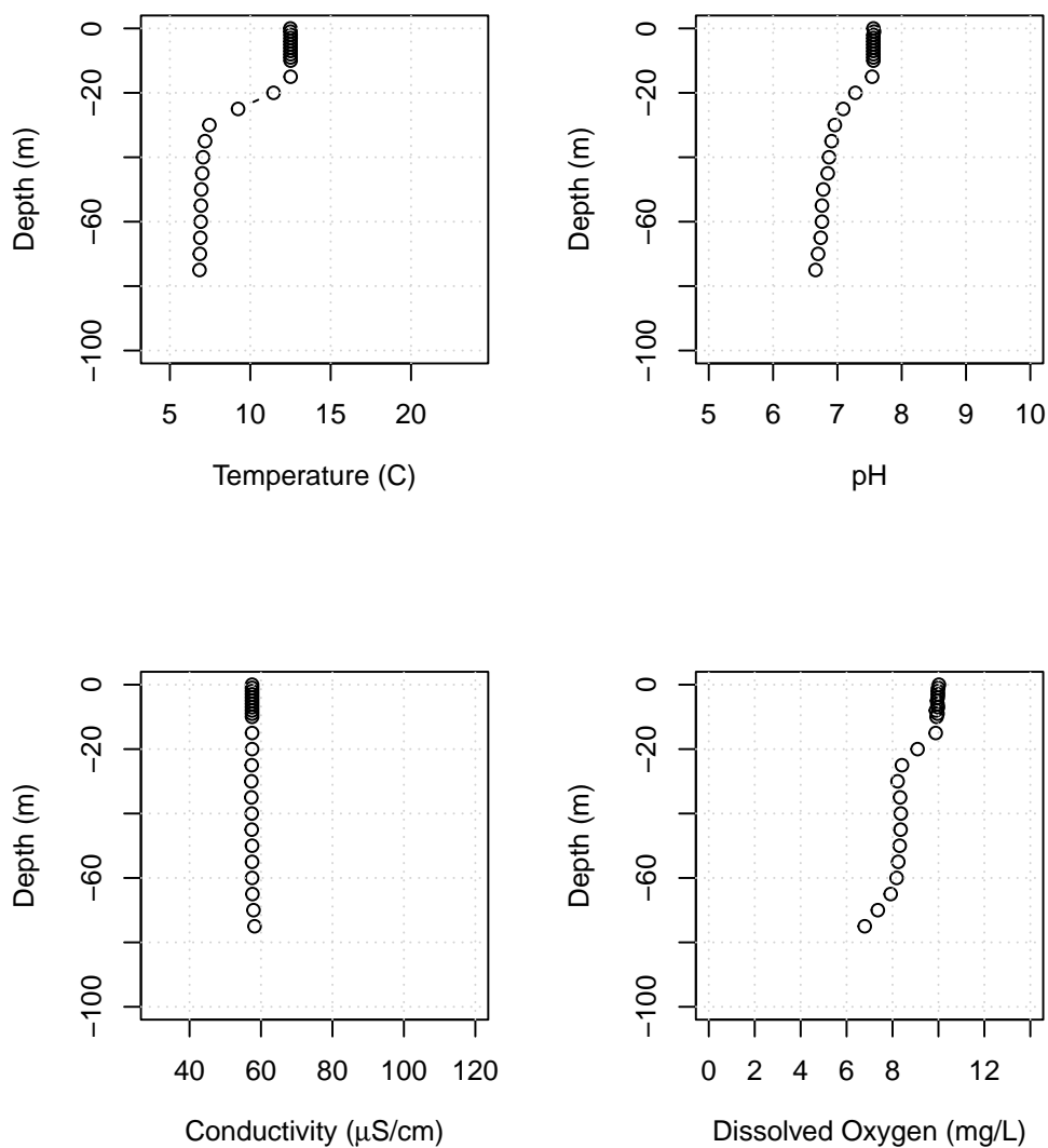
Figure B59: Lake Whatcom water column profiles showing temperature, pH, conductivity, and dissolved oxygen for Site 3, November 2, 2021.
