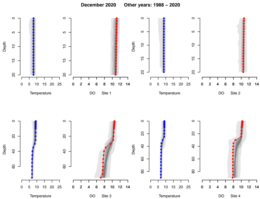
Figure 2.3: December 2020 temperature (-●-) and dissolved oxygen (-●-) profiles compared to historic ranges. The gradation in shading shows the approximate frequency of the 1988–2020 data.
