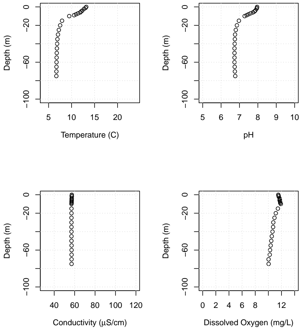
Figure B29: Lake Whatcom water column profiles showing temperature, pH, conductivity, and dissolved oxygen for Site 3, May 4, 2021.
