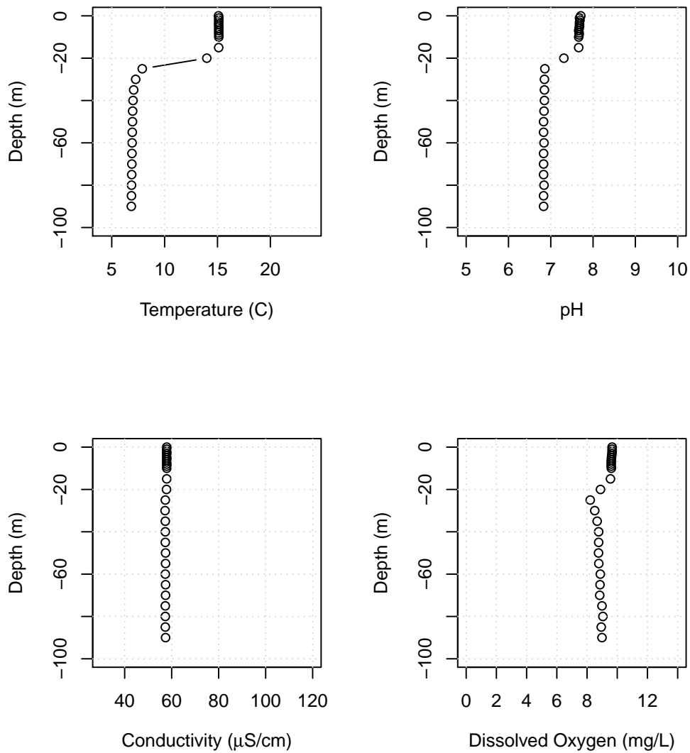
Figure B55: Lake Whatcom water column profiles showing temperature, pH, conductivity, and dissolved oxygen for Site 4, October 12, 2021.
