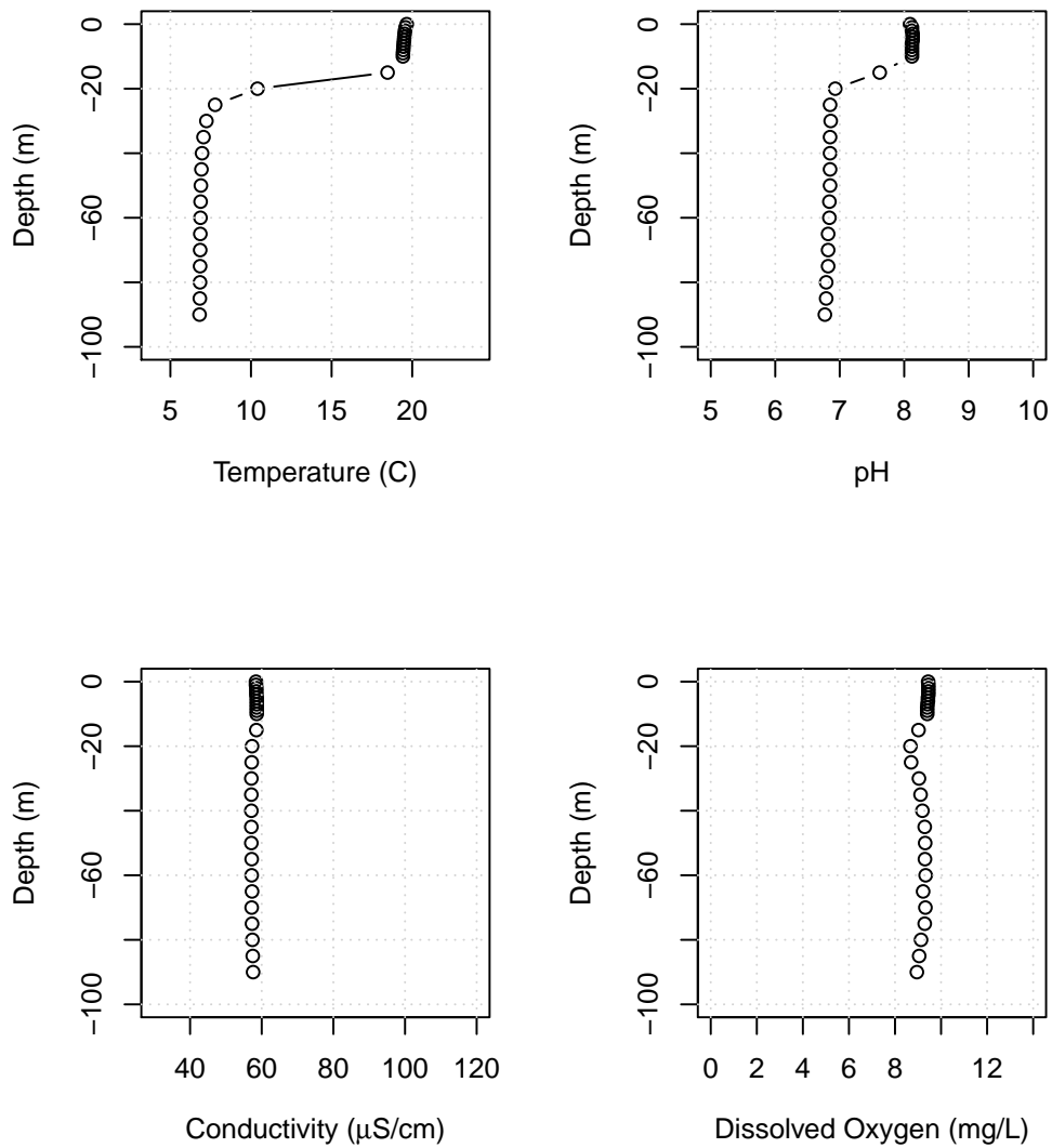
Figure B50: Lake Whatcom water column profiles showing temperature, pH, conductivity, and dissolved oxygen for Site 4, September 7, 2021.
