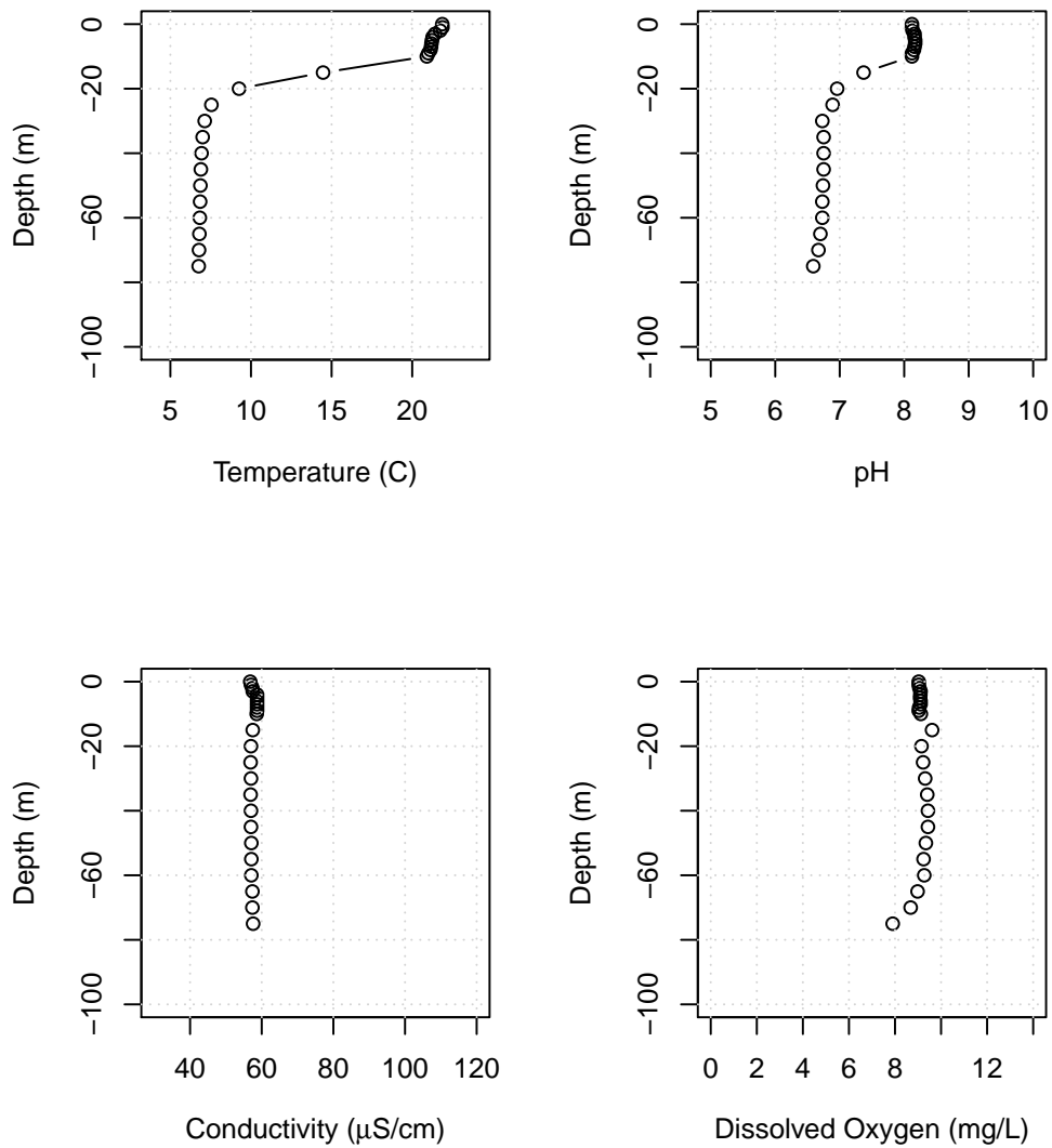
Figure B44: Lake Whatcom water column profiles showing temperature, pH, conductivity, and dissolved oxygen for Site 3, August 11, 2021.
