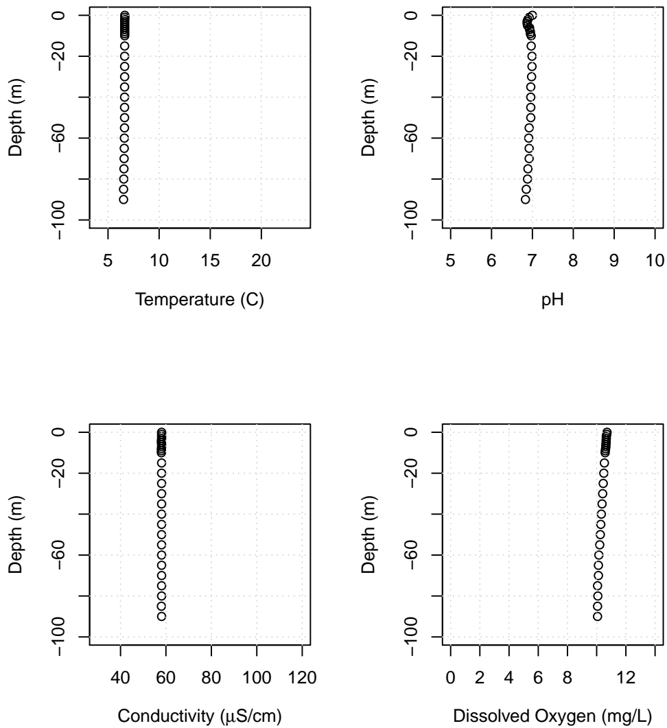
Figure B20: Lake Whatcom water column profiles showing temperature, pH, conductivity, and dissolved oxygen for Site 4, February 17, 2021.
