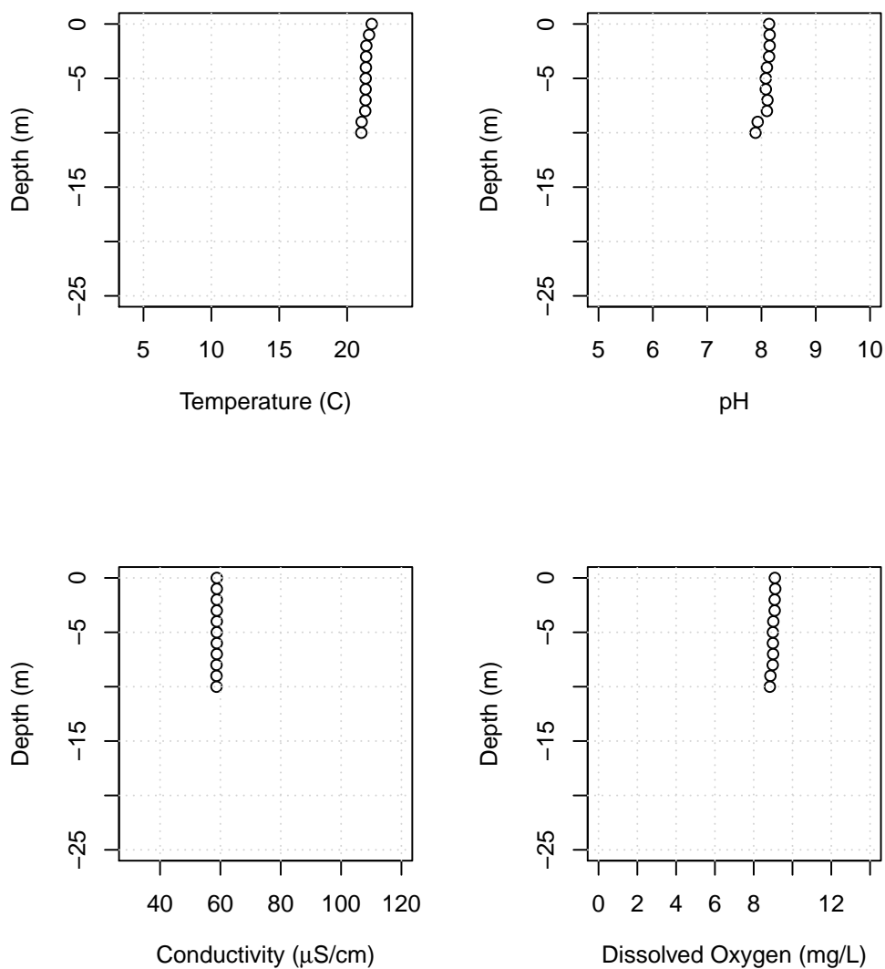
Figure B43: Lake Whatcom water column profiles showing temperature, pH, conductivity, and dissolved oxygen for the Intake, August 9, 2021.
