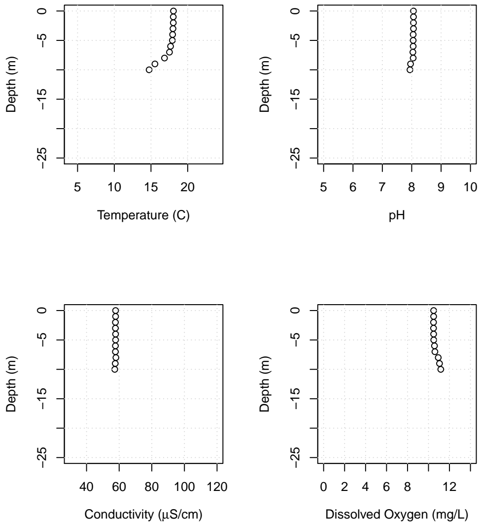
Figure B33: Lake Whatcom water column profiles showing temperature, pH, conductivity, and dissolved oxygen for the Intake, June 3, 2021.
