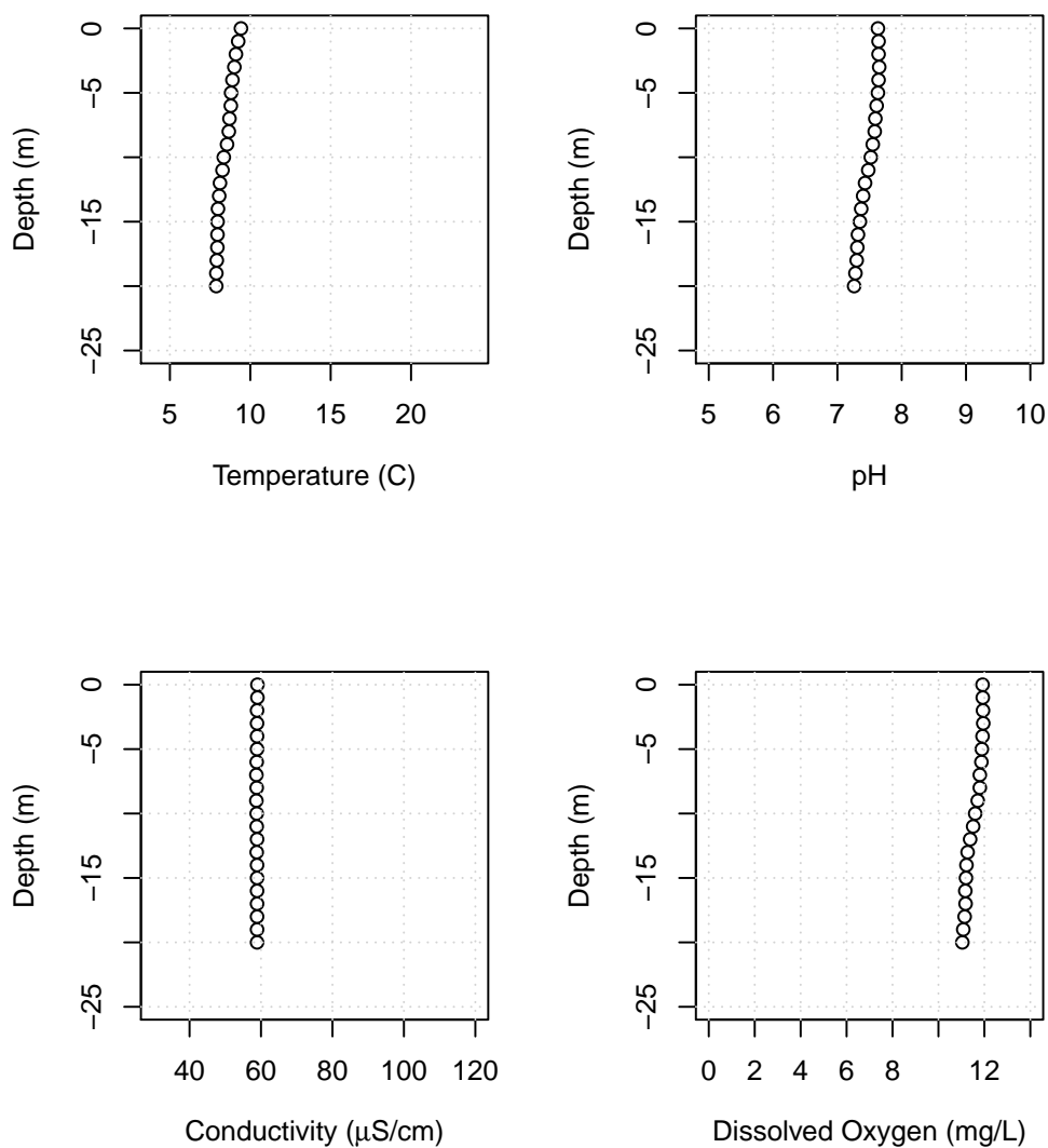
Figure B21: Lake Whatcom water column profiles showing temperature, pH, conductivity, and dissolved oxygen for Site 1, April 8, 2021.
