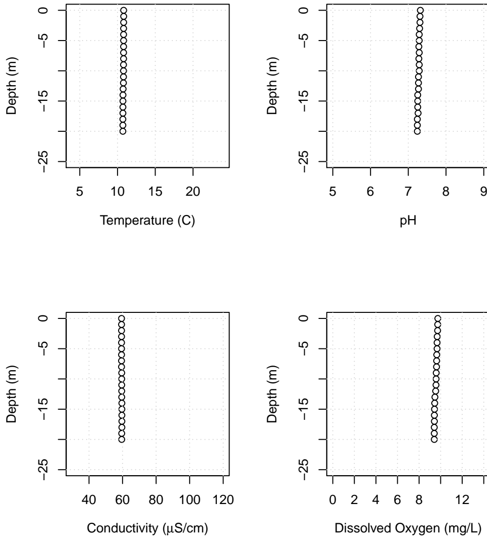
Figure B6: Lake Whatcom water column profiles showing temperature, pH, conductivity, and dissolved oxygen for Site 1, November 9, 2020.
