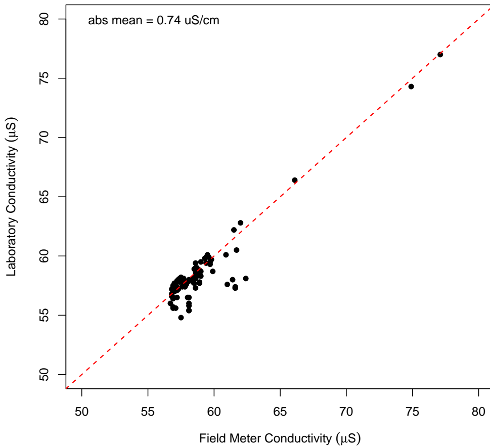
Figure C34: Conductivity field duplicates for the 2020/2021 Lake Whatcom monitoring program (lake samples). Diagonal reference line shows 1:1 relationship.
