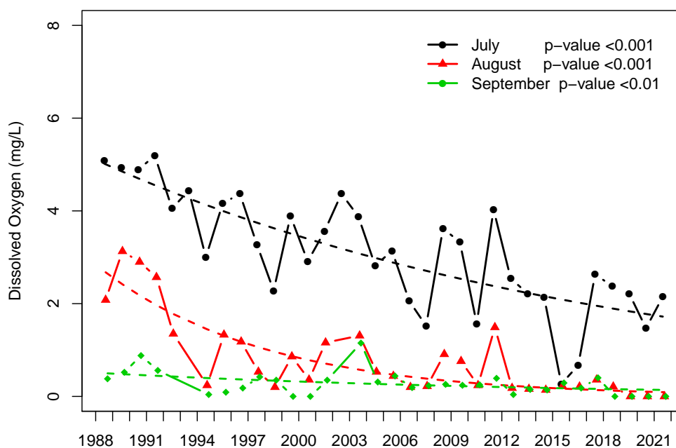
Site 1 Dissolved Oxygen by Year at Depth 18
