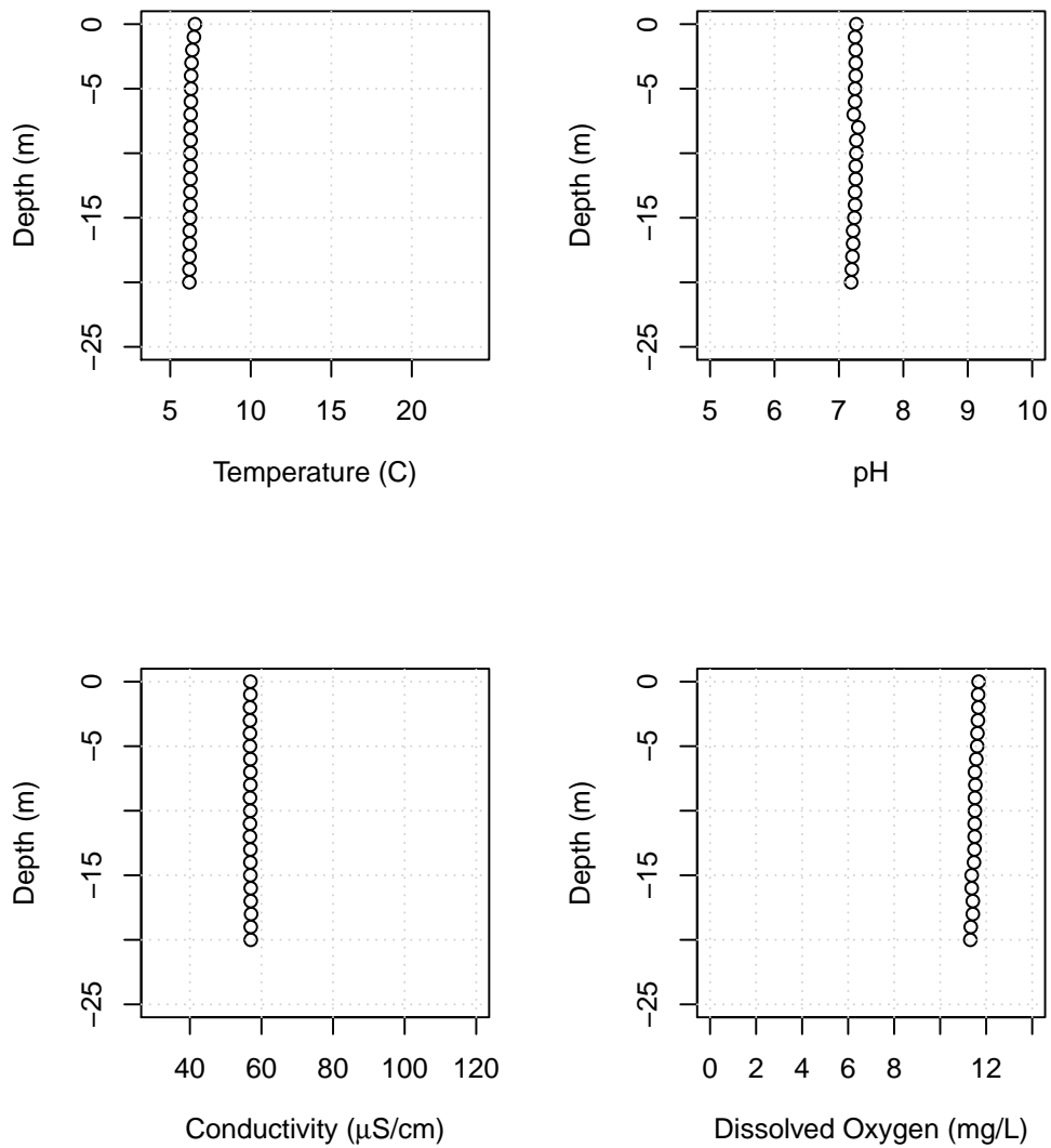
Figure B17: Lake Whatcom water column profiles showing temperature, pH, conductivity, and dissolved oxygen for Site 2, February 24, 2021.
