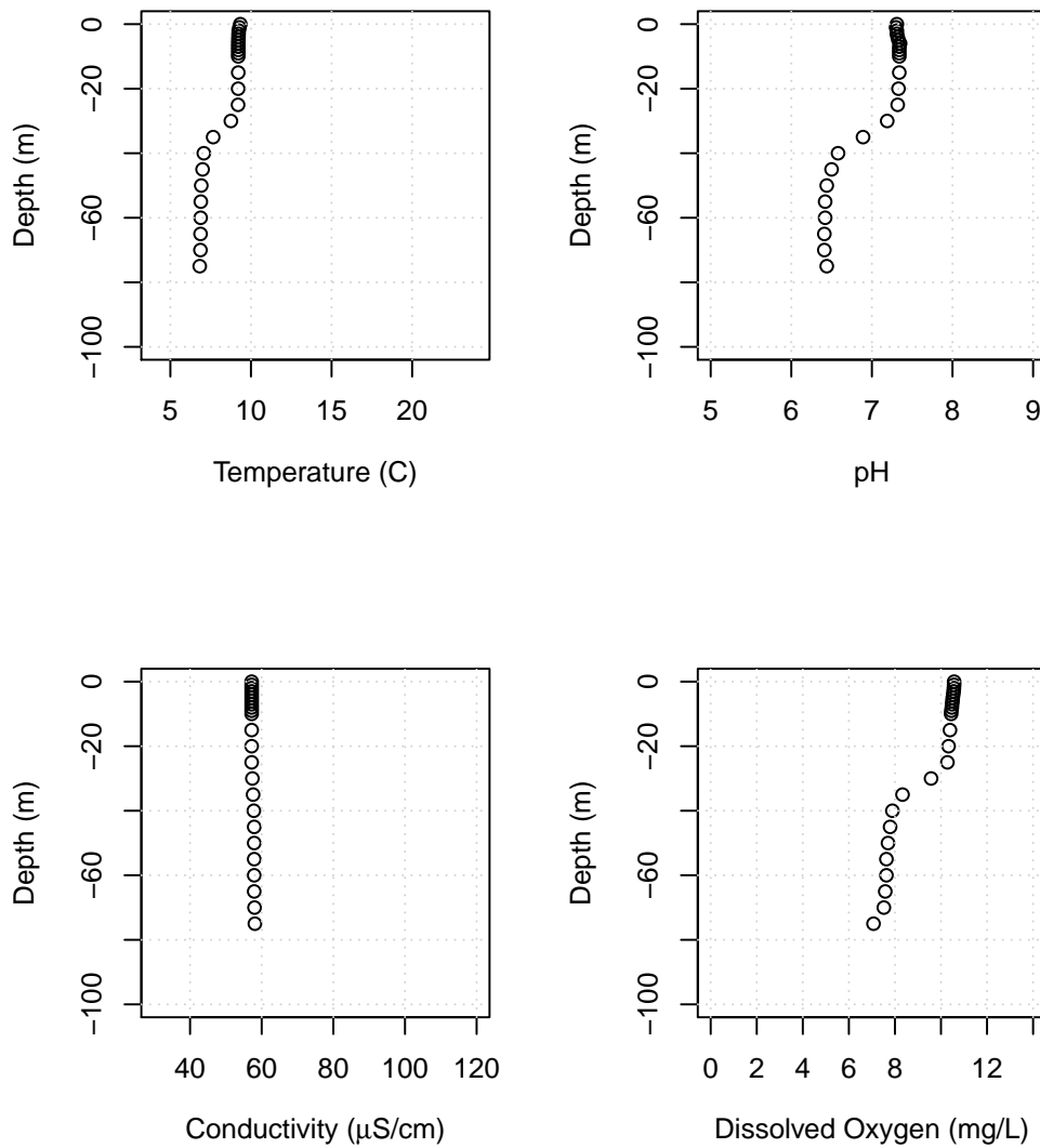
Figure B14: Lake Whatcom water column profiles showing temperature, pH, conductivity, and dissolved oxygen for Site 3, December 2, 2020.
