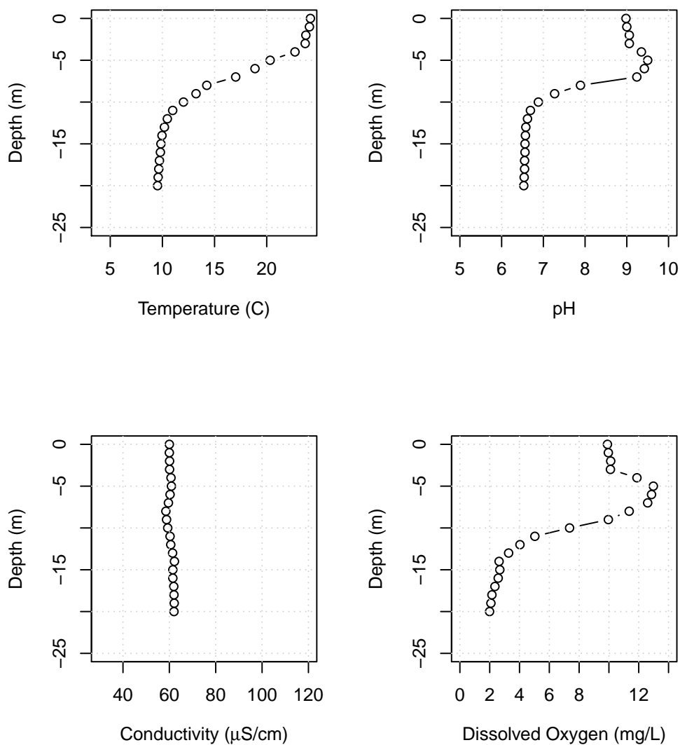
Figure B36: Lake Whatcom water column profiles showing temperature, pH, conductivity, and dissolved oxygen for Site 1, July 6, 2021.
