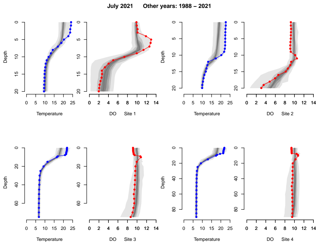
Figure 2.8: July 2021 temperature (-●-) and dissolved oxygen (-●-) profiles compared to historic ranges. The gradation in shading shows the approximate frequency of the 1988–2021 data.
