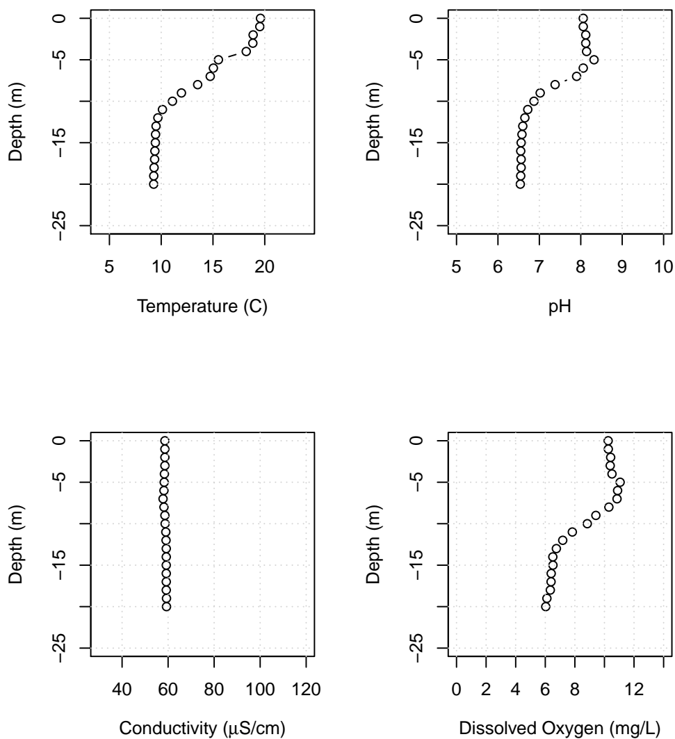
Figure B31: Lake Whatcom water column profiles showing temperature, pH, conductivity, and dissolved oxygen for Site 1, June 3, 2021.
