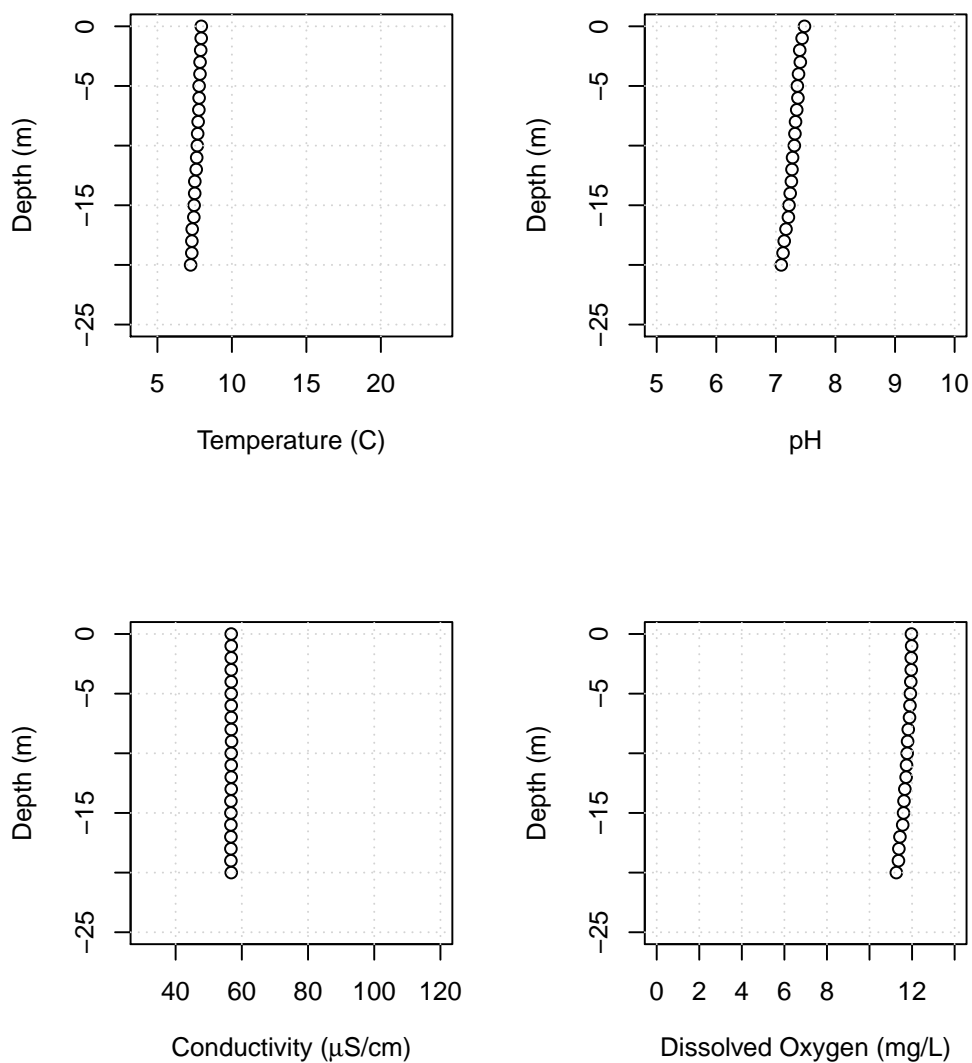
Figure B22: Lake Whatcom water column profiles showing temperature, pH, conductivity, and dissolved oxygen for Site 2, April 8, 2021.
