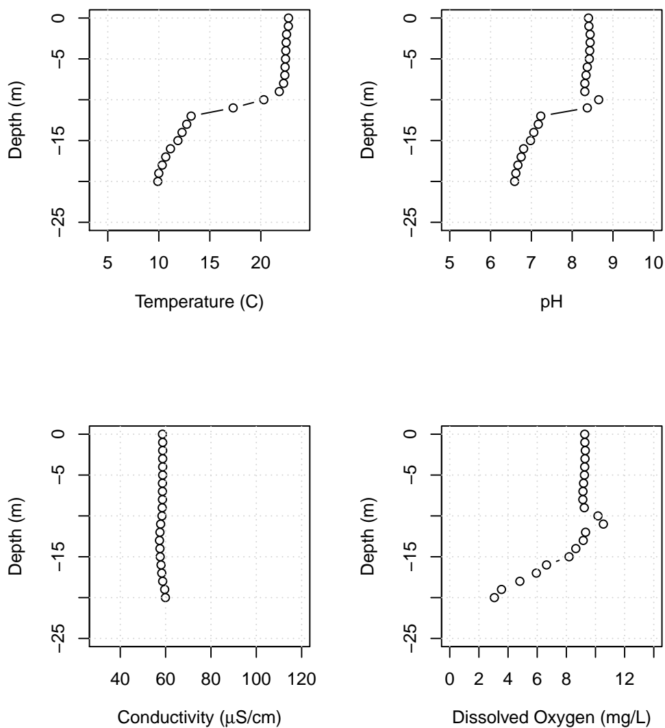
Figure B37: Lake Whatcom water column profiles showing temperature, pH, conductivity, and dissolved oxygen for Site 2, July 8, 2021.
