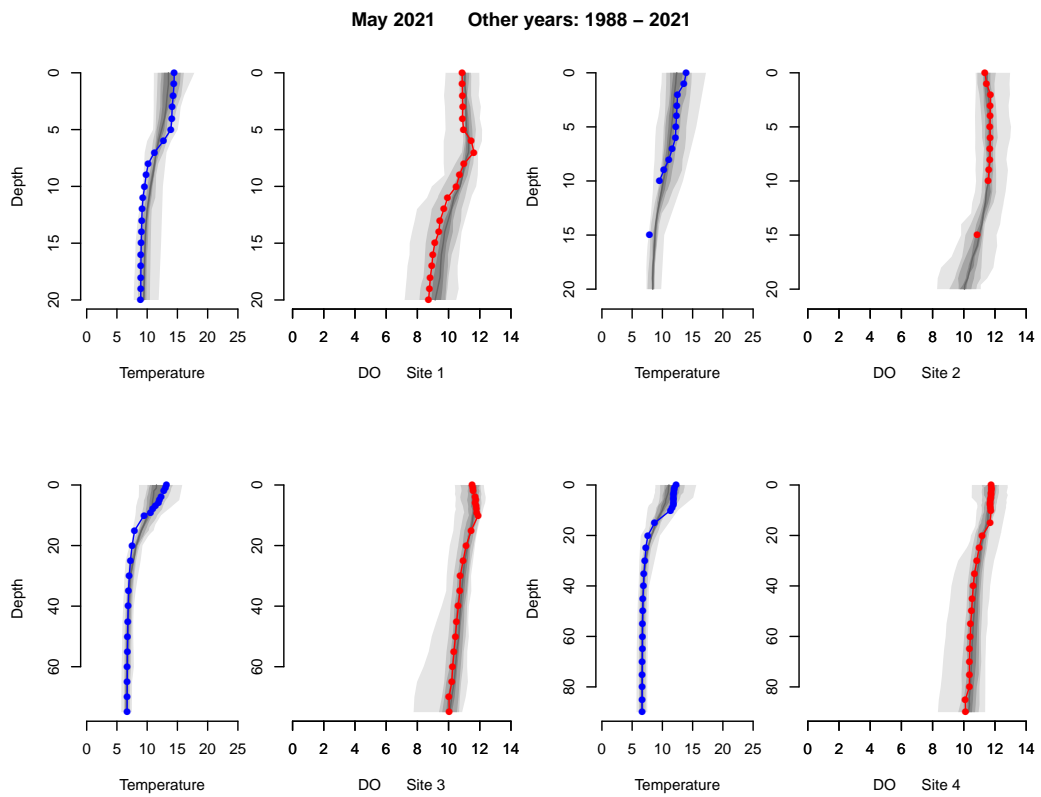
Figure 2.6: May 2021 temperature (-●-) and dissolved oxygen (-●-) profiles compared to historic ranges. The gradation in shading shows the approximate frequency of the 1988–2021 data.
