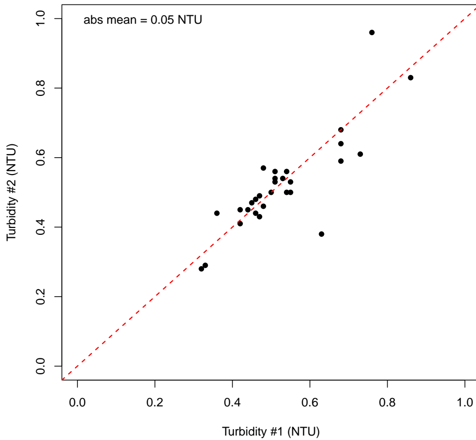
Figure C48: Turbidity field duplicates for the 2020/2021 Lake Whatcom monitoring program (lake samples). Diagonal reference line shows 1:1 relationship.
