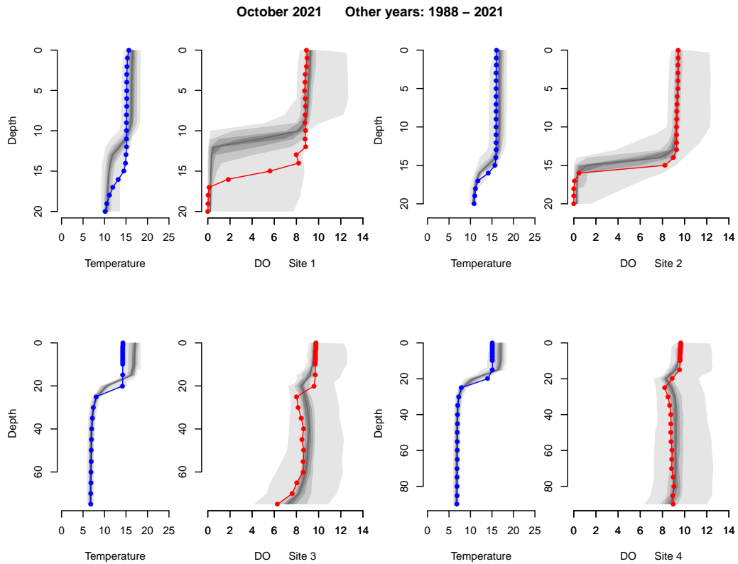
Figure 2.11: October 2021 temperature (-●-) and dissolved oxygen (-●-) profiles compared to historic ranges. The gradation in shading shows the approximate frequency of the 1988–2021 data. October 2021 is not part of the 2020/2021 sampling period, but were included to to provide information on the timing of destratification.
