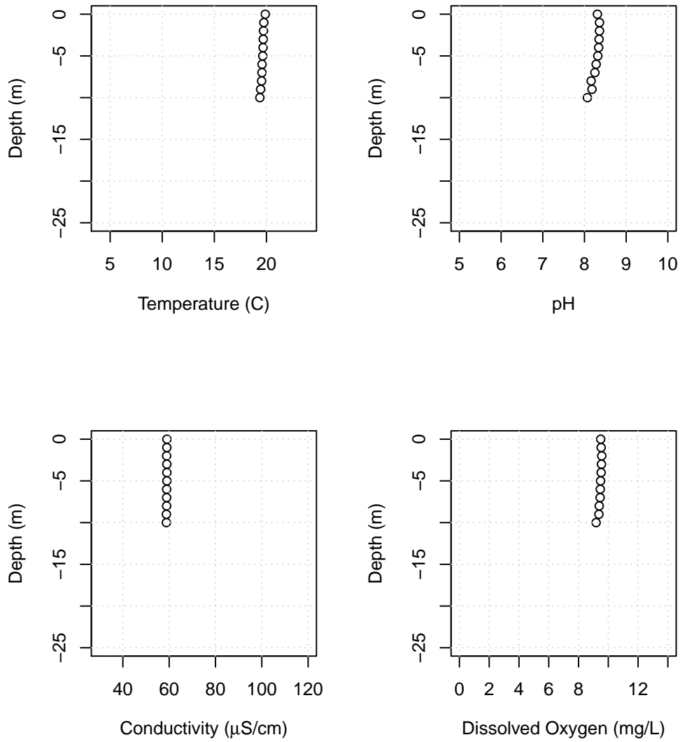
Figure B48: Lake Whatcom water column profiles showing temperature, pH, conductivity, and dissolved oxygen for the Intake, September 9, 2021.
