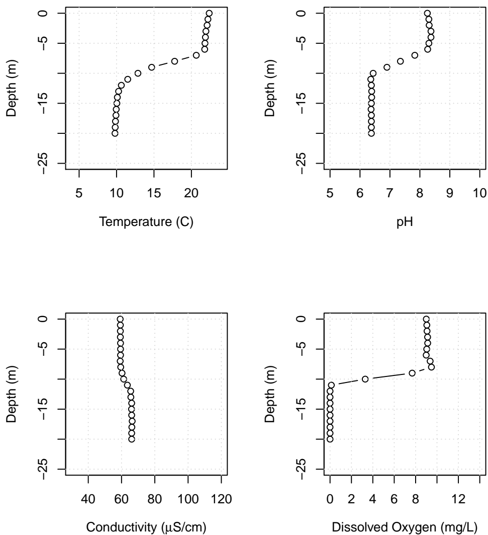
Figure B41: Lake Whatcom water column profiles showing temperature, pH, conductivity, and dissolved oxygen for Site 1, August 9, 2021.
