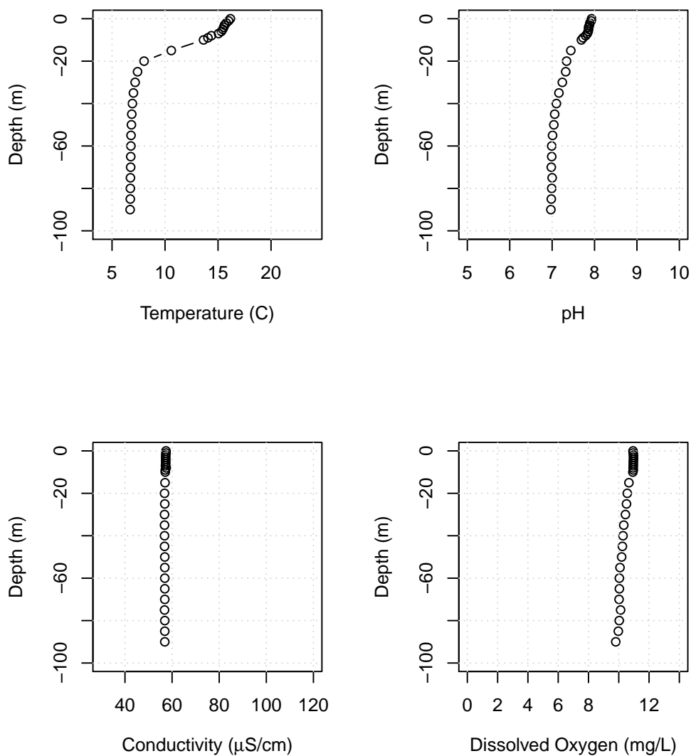
Figure B35: Lake Whatcom water column profiles showing temperature, pH, conductivity, and dissolved oxygen for Site 4, June 1, 2021.
