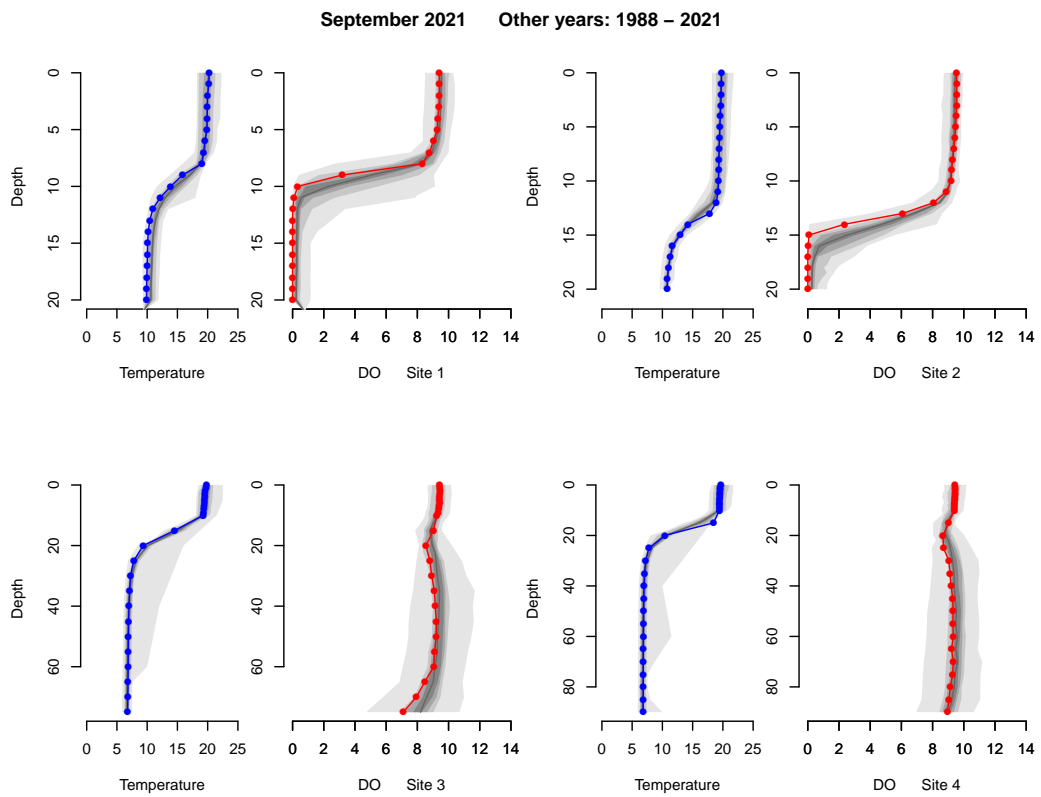
Figure 2.10: September 2021 temperature (---●---) and dissolved oxygen (---●---) profiles compared to historic ranges. The gradation in shading shows the approximate frequency of the 1988–2021 data.
