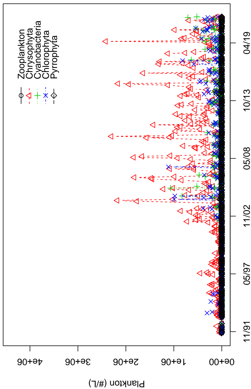
Figure B137: Lake Whatcom plankton data for Site 2.
