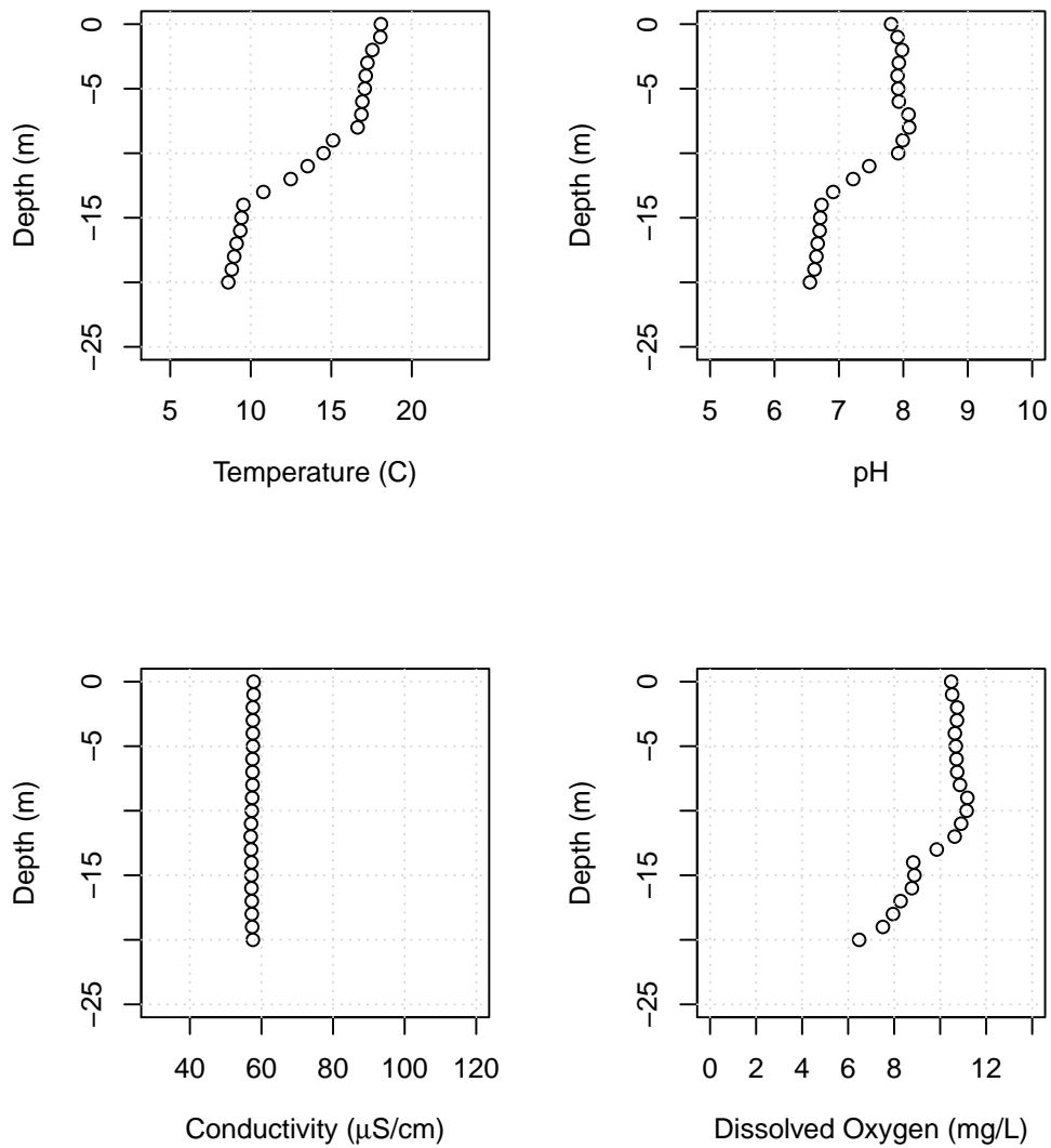
Figure B32: Lake Whatcom water column profiles showing temperature, pH, conductivity, and dissolved oxygen for Site 2, June 3, 2021.
