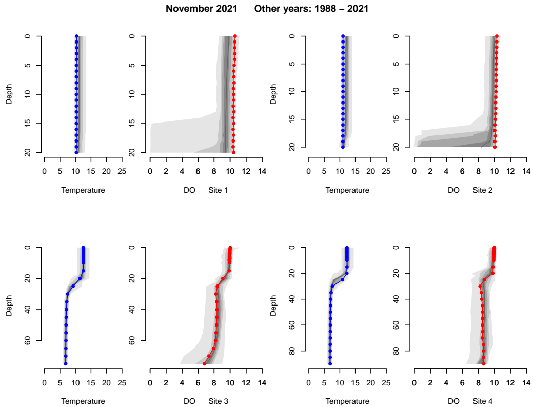
Figure 2.12: November 2021 temperature (-●-) and dissolved oxygen (-●-) profiles compared to historic ranges. The gradation in shading shows the approximate frequency of the 1988–2021 data. November 2021 is not part of the 2020/2021 sampling period, but were included to to provide information on the timing of destratification.
