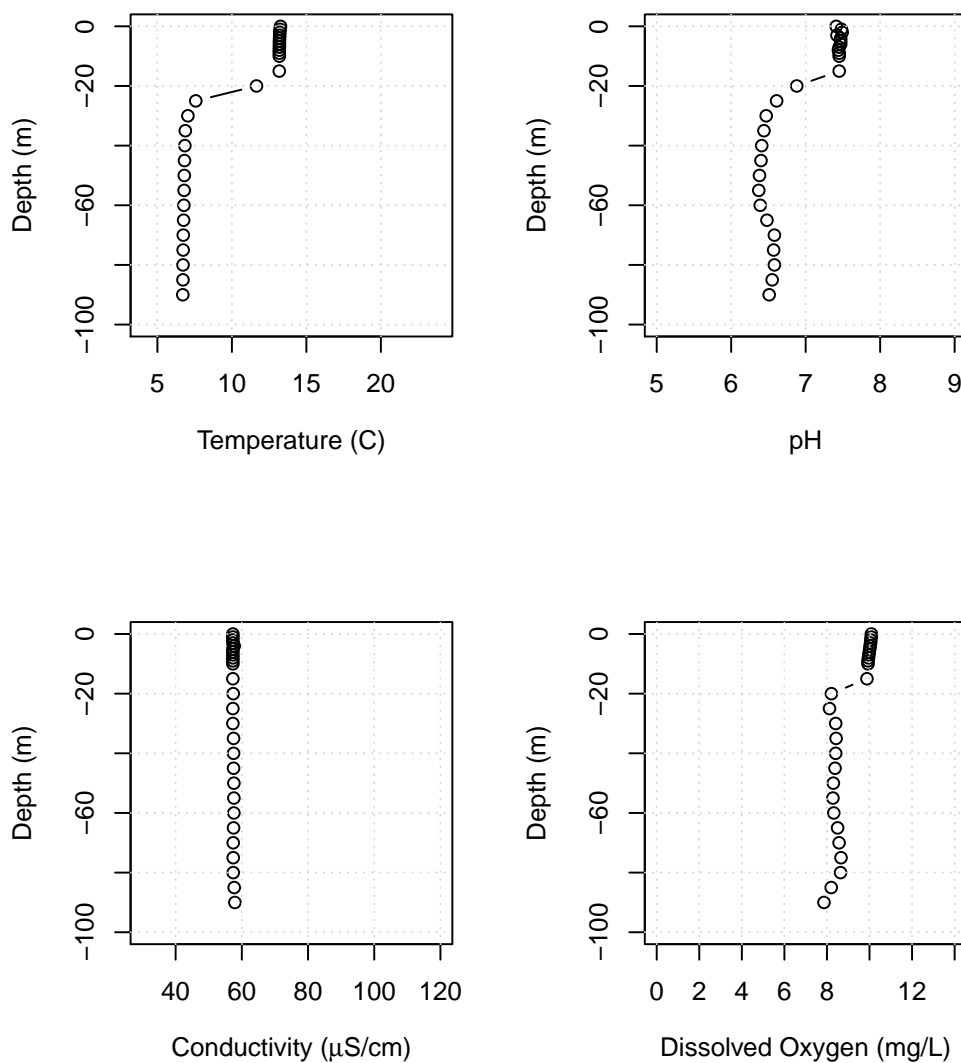
Figure B10: Lake Whatcom water column profiles showing temperature, pH, conductivity, and dissolved oxygen for Site 4, November 2, 2020.
