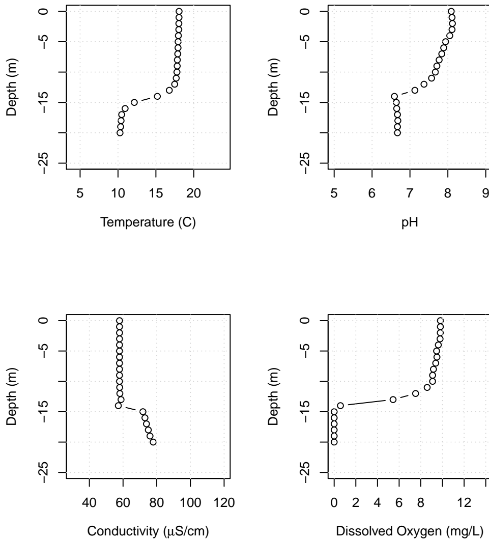
Figure B2: Lake Whatcom water column profiles showing temperature, pH, conductivity, and dissolved oxygen for Site 2, October 7, 2020.
