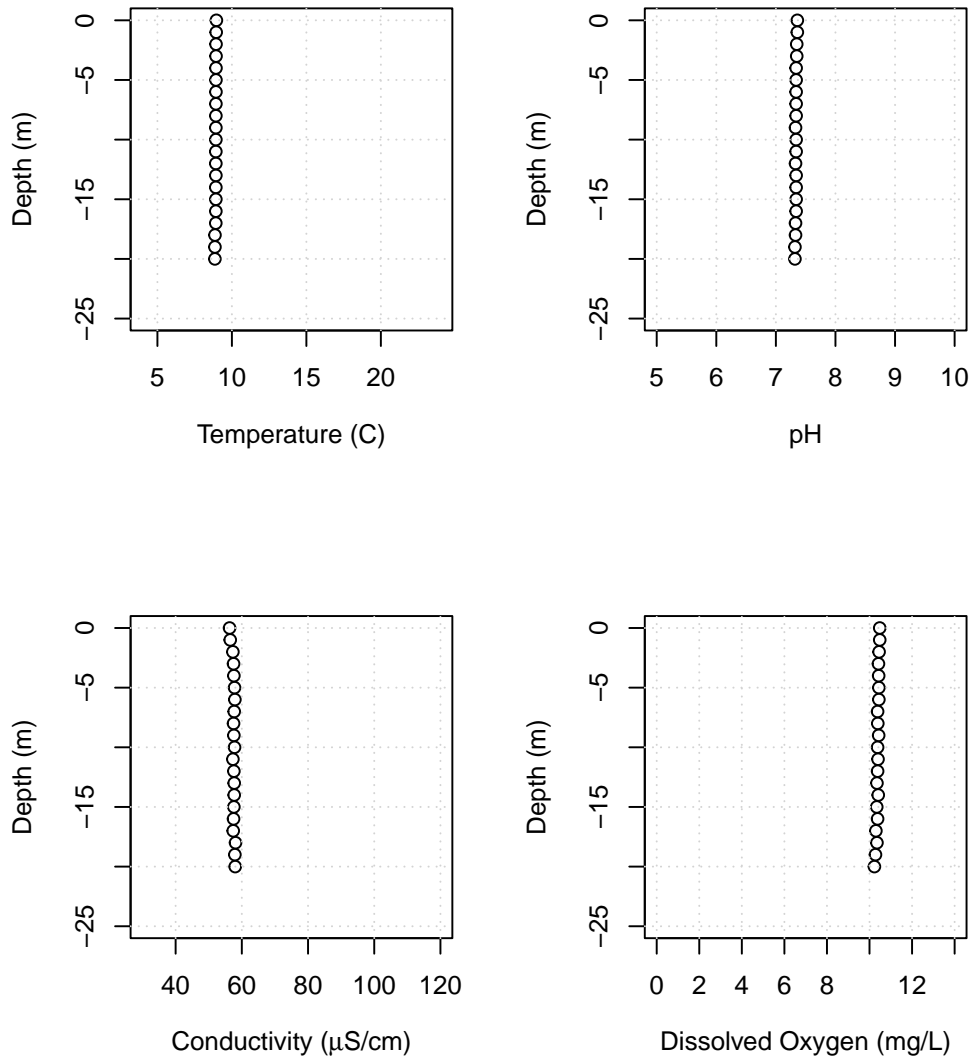
Figure B61: Lake Whatcom water column profiles showing temperature, pH, conductivity, and dissolved oxygen for Site 1, December 9, 2021.
