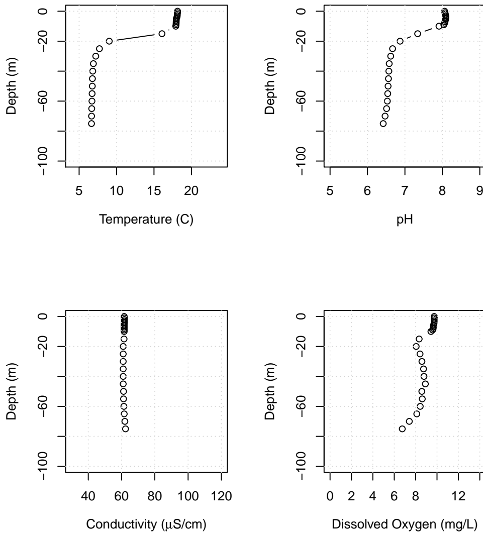
Figure B4: Lake Whatcom water column profiles showing temperature, pH, conductivity, and dissolved oxygen for Site 3, October 5, 2020.
