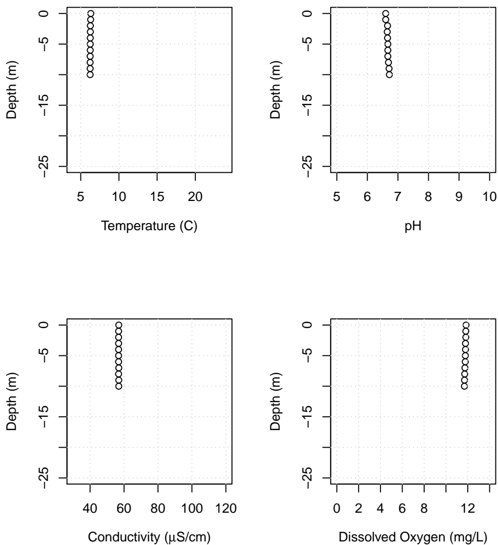
Figure B18: Lake Whatcom water column profiles showing temperature, pH, conductivity, and dissolved oxygen for the Intake, February 27, 2021.
