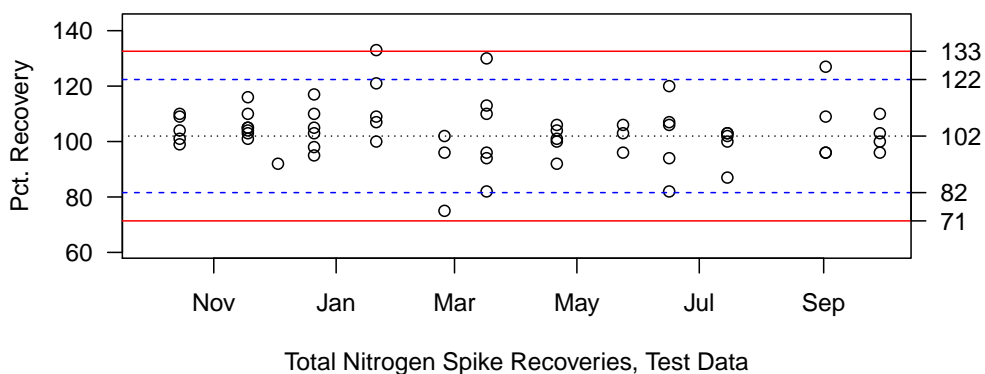
Figure C16: Nitrogen (total) spike recoveries for the Lake Whatcom monitoring program. Upper/lower acceptance limits ( \pm 2 std. dev. from mean pair difference) and upper/lower warning limits ( \pm 3 std. dev. from mean pair difference) were calculated based on the preceding two years of spike data.
