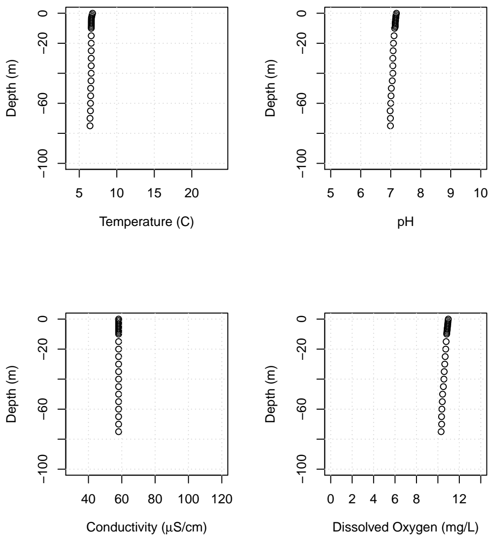
Figure B19: Lake Whatcom water column profiles showing temperature, pH, conductivity, and dissolved oxygen for Site 3, February 17, 2021.
