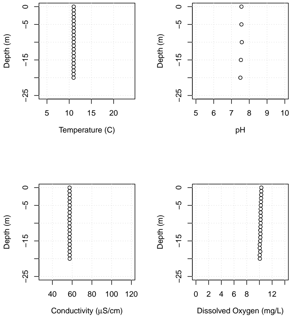
Figure B57: Lake Whatcom water column profiles showing temperature, pH, conductivity, and dissolved oxygen for Site 2, November 9, 2021.
