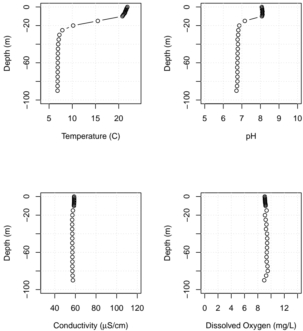
Figure B45: Lake Whatcom water column profiles showing temperature, pH, conductivity, and dissolved oxygen for Site 4, August 11, 2021.
