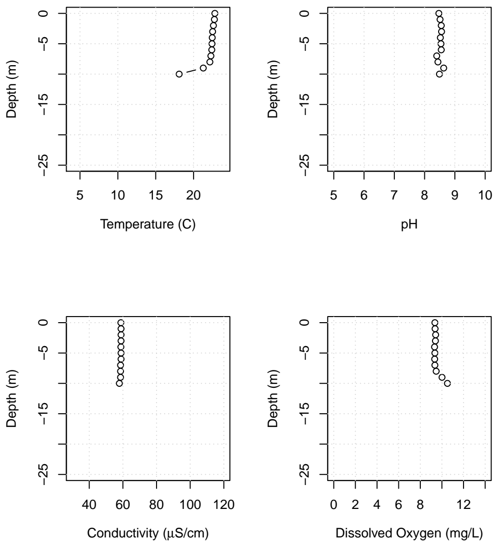
Figure B38: Lake Whatcom water column profiles showing temperature, pH, conductivity, and dissolved oxygen for the Intake, July 8, 2021.
