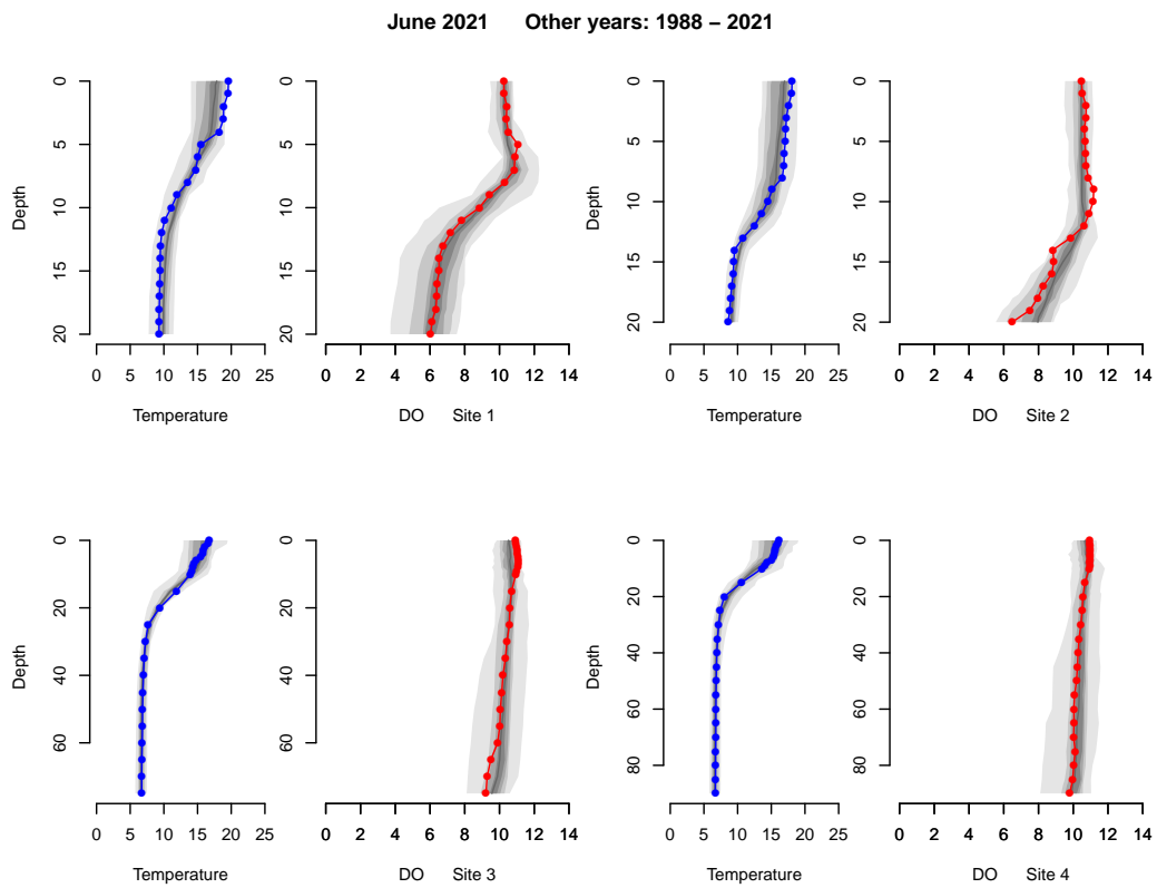
Figure 2.7: June 2021 temperature (-●-) and dissolved oxygen (-●-) profiles compared to historic ranges. The gradation in shading shows the approximate frequency of the 1988–2021 data.
