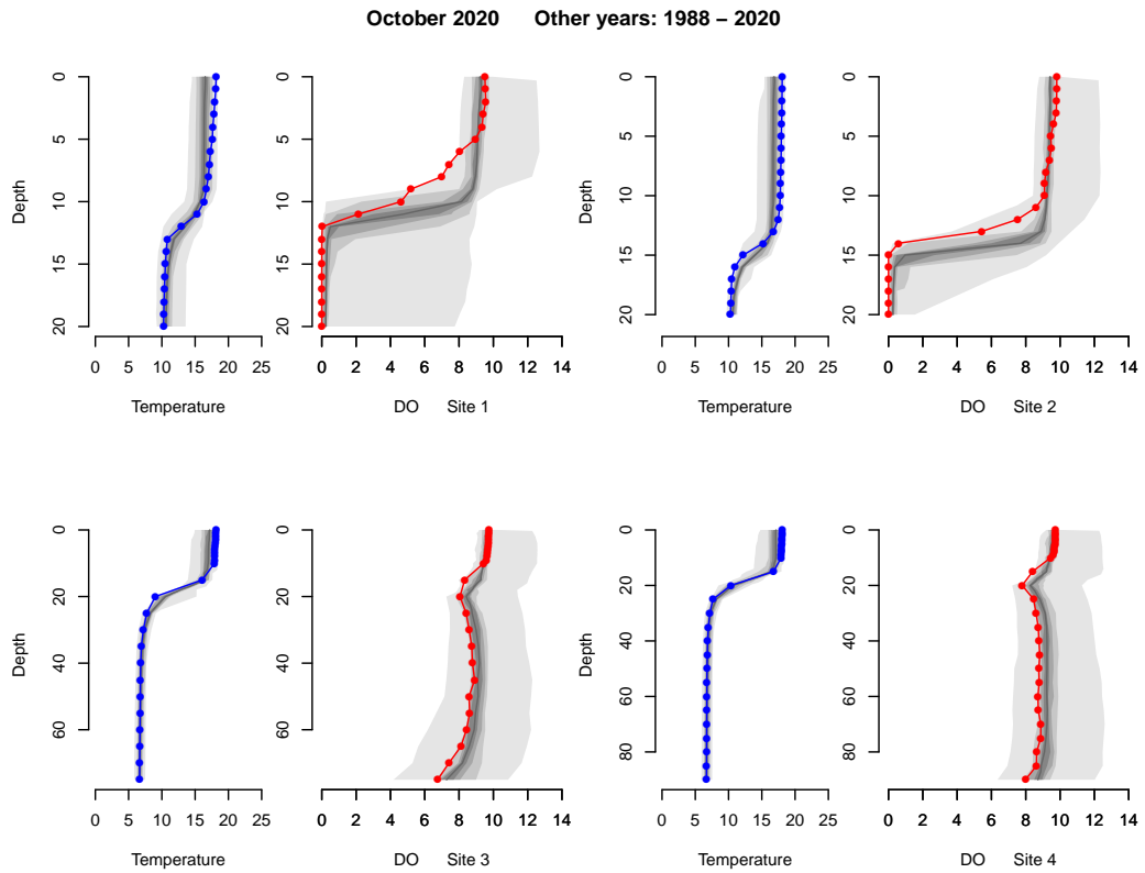
Figure 2.1: October 2020 temperature (-●-) and dissolved oxygen (-●-) profiles compared to historic ranges. The gradation in shading shows the approximate frequency of the 1988–2020 data.
