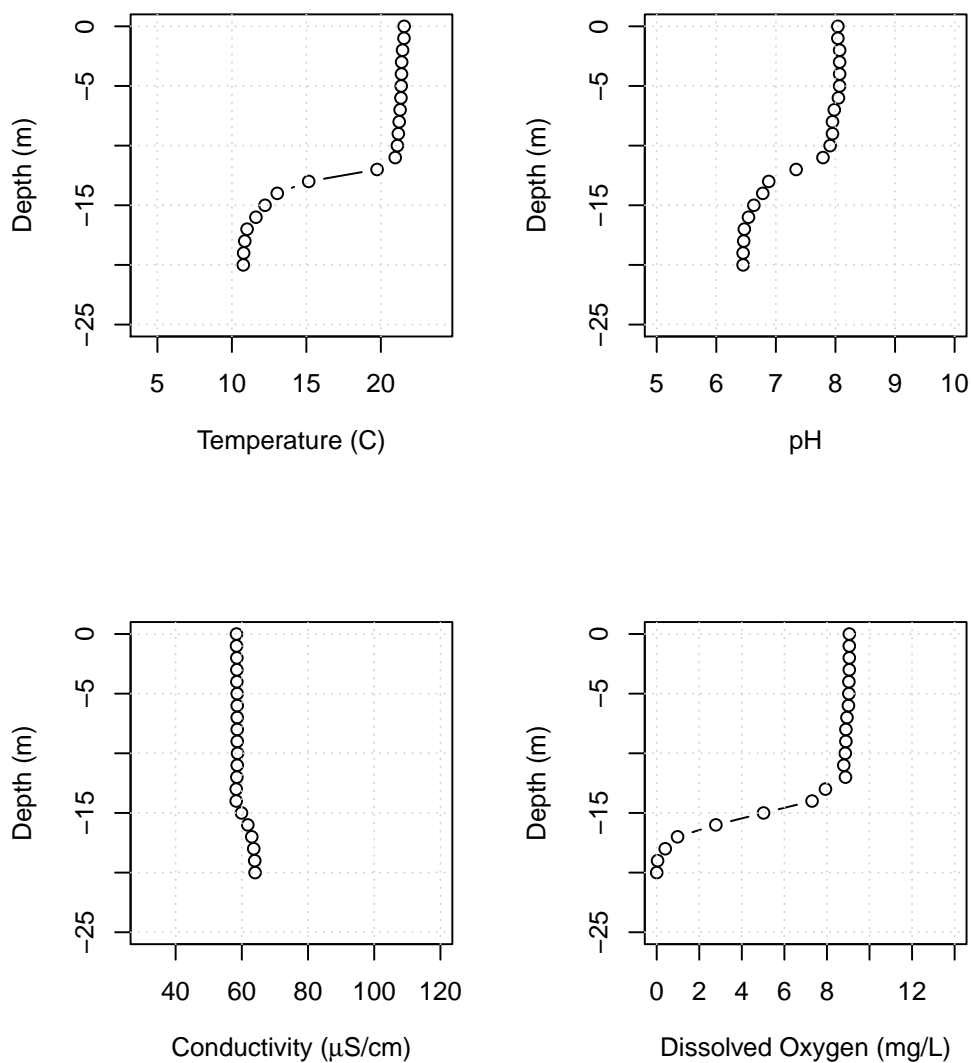
Figure B42: Lake Whatcom water column profiles showing temperature, pH, conductivity, and dissolved oxygen for Site 2, August 9, 2021.
