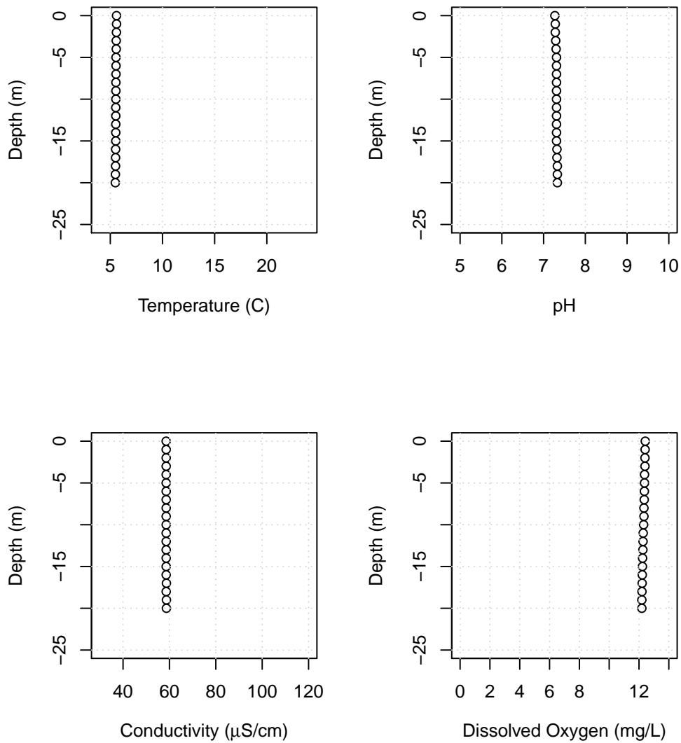
Figure B16: Lake Whatcom water column profiles showing temperature, pH, conductivity, and dissolved oxygen for Site 1, February 27, 2021.
