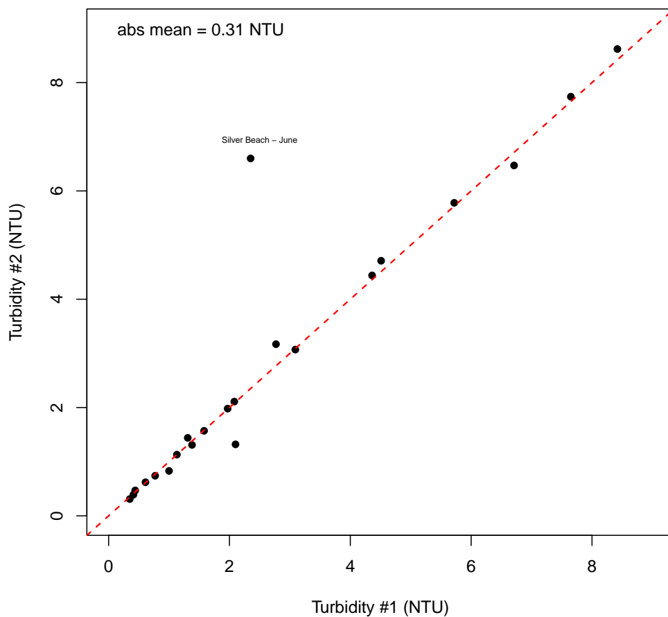
Figure C49: Turbidity field duplicates for the 2020/2021 Lake Whatcom monitoring program (tributary samples). Diagonal reference line shows 1:1 relationship. The outlier identified likely represents sediment contamination of the duplicate sample.
