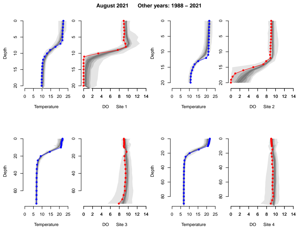
Figure 2.9: August 2021 temperature (-●-) and dissolved oxygen (-●-) profiles compared to historic ranges. The gradation in shading shows the approximate frequency of the 1988–2021 data.
