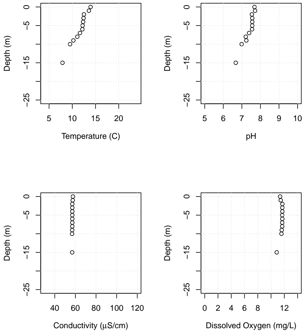
Figure B27: Lake Whatcom water column profiles showing temperature, pH, conductivity, and dissolved oxygen for Site 2, May 6, 2021.
