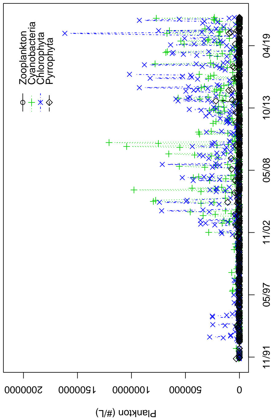
Figure B141: Lake Whatcom plankton data for Site 1, with Chrysophyta omitted to show remaining plankton groups.
