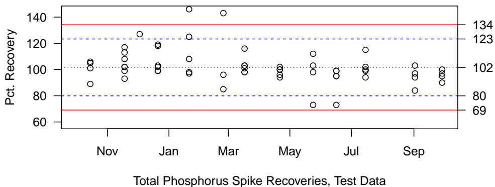
Figure C25: Phosphorus (total) spike recoveries for the Lake Whatcom monitoring program. Upper/lower acceptance limits ( \pm 2 std. dev. from mean pair difference) and upper/lower warning limits ( \pm 3 std. dev. from mean pair difference) were calculated based on the preceding two years of spike data.
