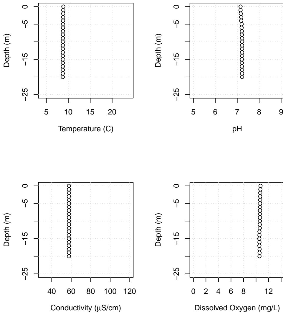
Figure B12: Lake Whatcom water column profiles showing temperature, pH, conductivity, and dissolved oxygen for Site 2, December 9, 2020.
