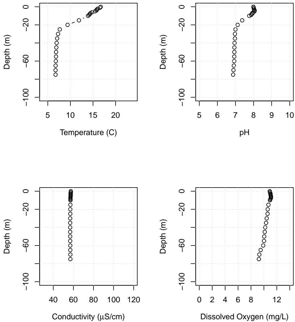
Figure B34: Lake Whatcom water column profiles showing temperature, pH, conductivity, and dissolved oxygen for Site 3, June 1, 2021.
