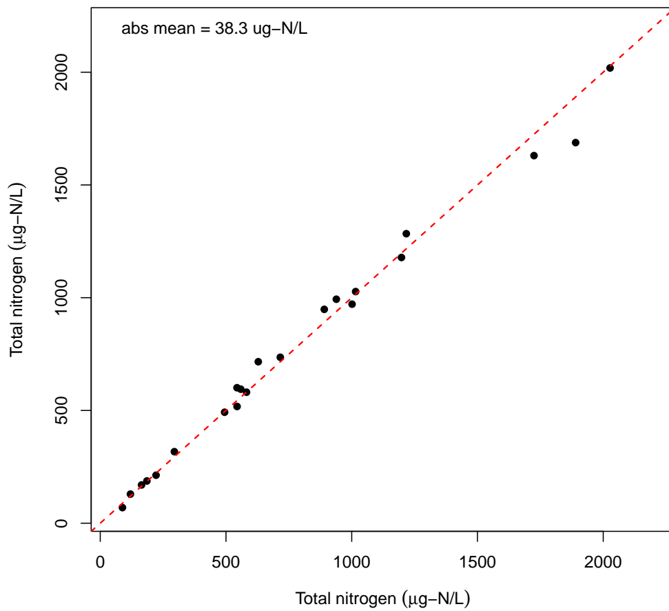
Figure C42: Nitrogen (total) field duplicates for the 2020/2021 Lake Whatcom monitoring program (tributary samples). Diagonal reference line shows 1:1 relationship.
