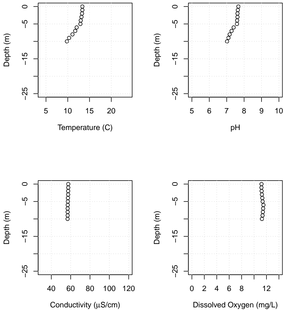
Figure B28: Lake Whatcom water column profiles showing temperature, pH, conductivity, and dissolved oxygen for the Intake, May 10, 2021.
