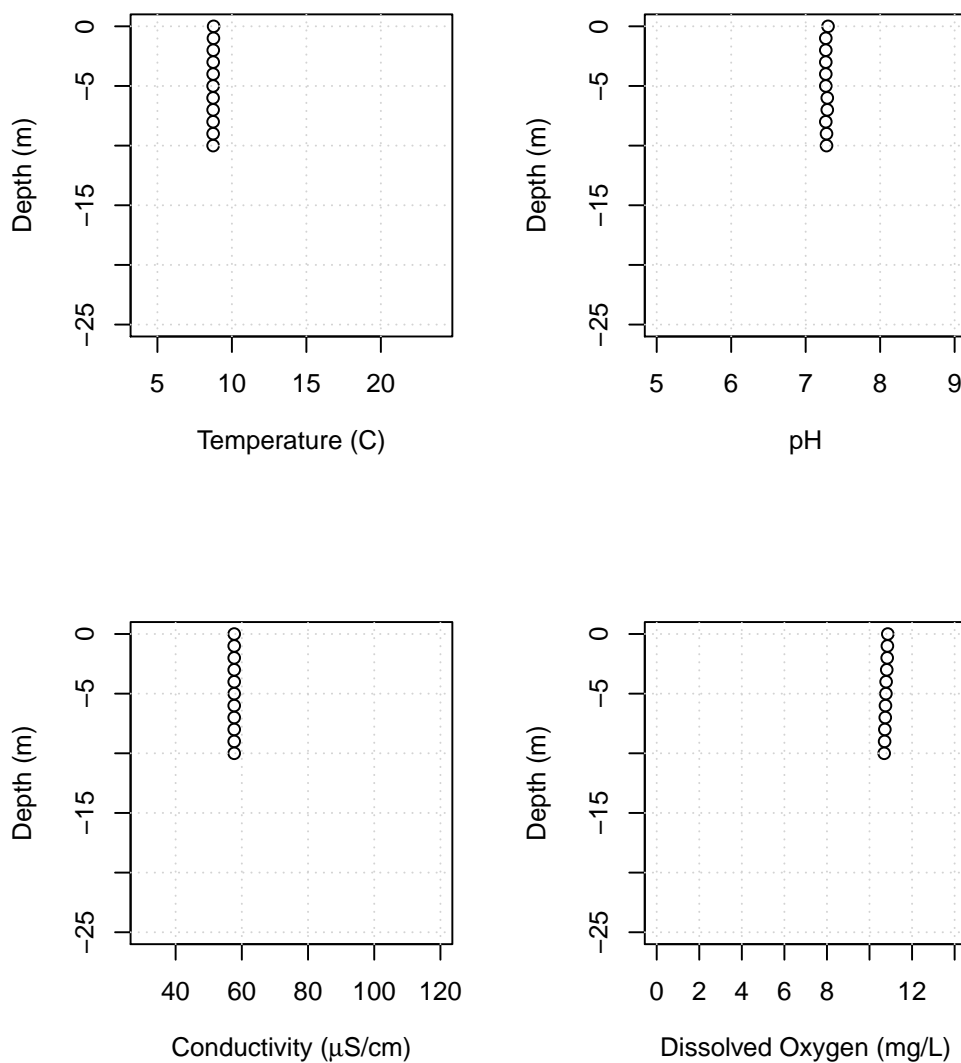
Figure B13: Lake Whatcom water column profiles showing temperature, pH, conductivity, and dissolved oxygen for the Intake, December 9, 2020.
