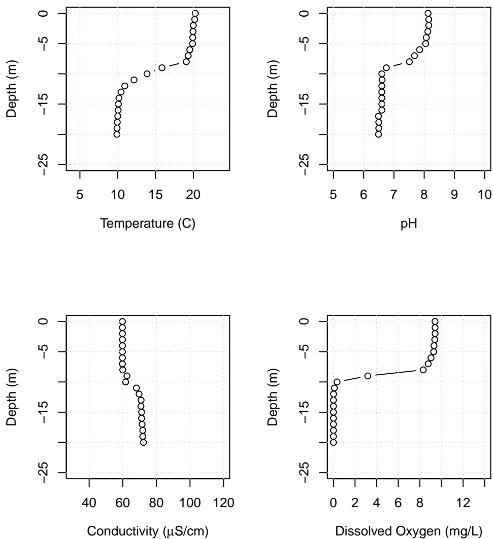
Figure B46: Lake Whatcom water column profiles showing temperature, pH, conductivity, and dissolved oxygen for Site 1, September 9, 2021.
