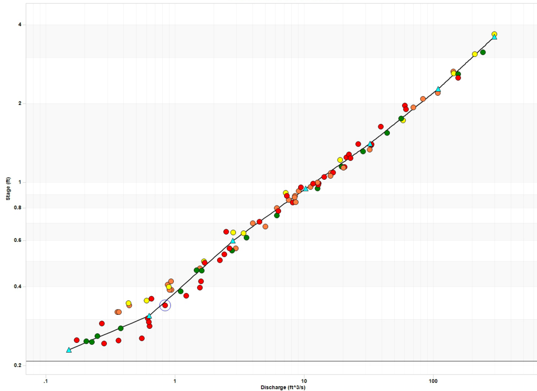
Figure 4.3: Aquarius rating curve for Austin Creek. The triangles (▲) show the fitted rating curve for WY2021. The circles show data collected in WY2021 (●), WY2020 (●), WY2019 (●). The red circles (●) show data collected prior to WY2019 that were used for the rating curve because they help define the high end of the rating curve.
