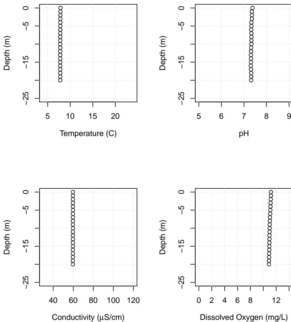
Figure B11: Lake Whatcom water column profiles showing temperature, pH, conductivity, and dissolved oxygen for Site 1, December 9, 2020.
