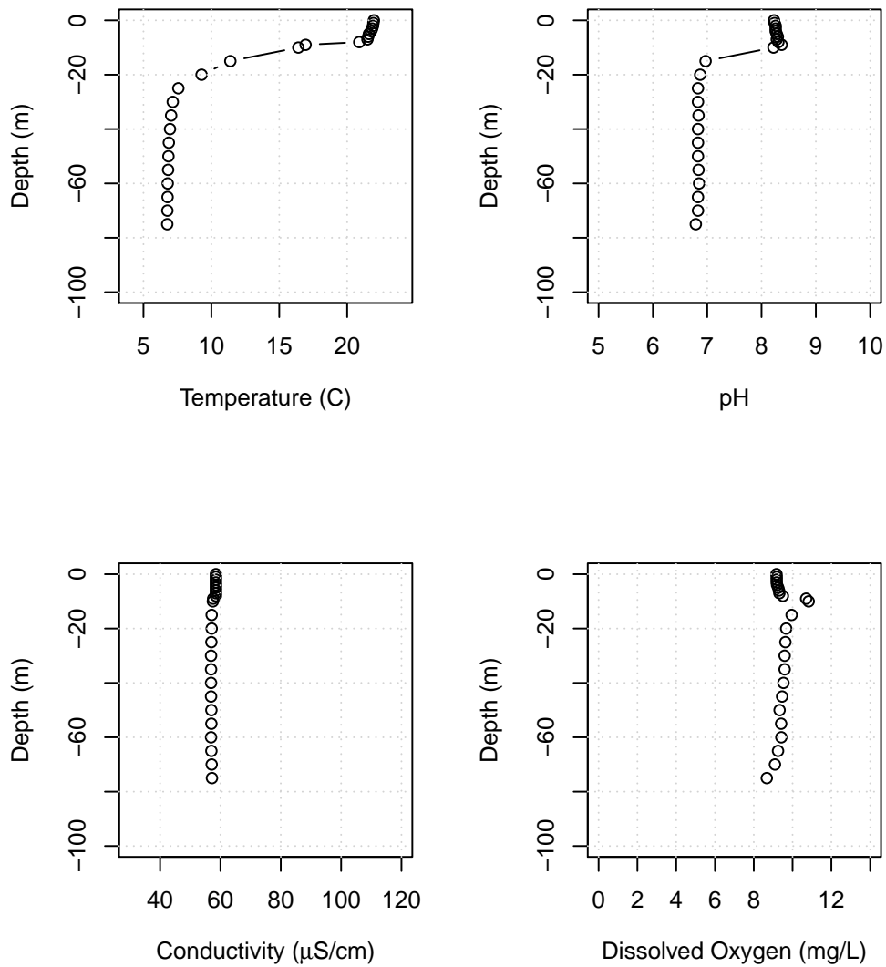
Figure B39: Lake Whatcom water column profiles showing temperature, pH, conductivity, and dissolved oxygen for Site 3, July 8, 2021.
