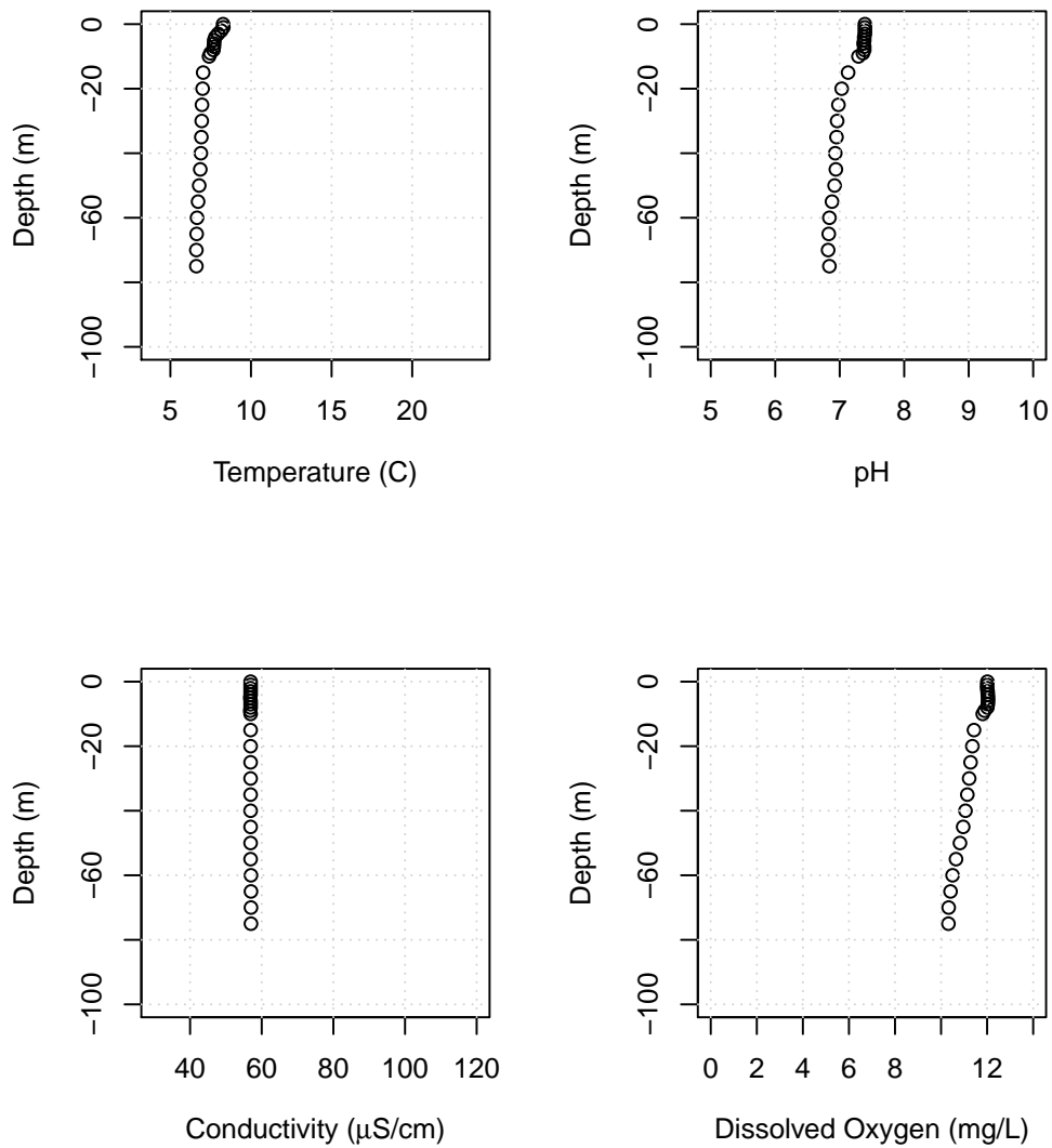
Figure B24: Lake Whatcom water column profiles showing temperature, pH, conductivity, and dissolved oxygen for Site 3, April 6, 2021.
