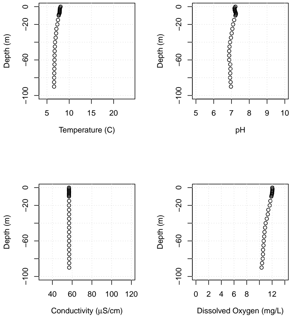
Figure B25: Lake Whatcom water column profiles showing temperature, pH, conductivity, and dissolved oxygen for Site 4, April 6, 2021.
