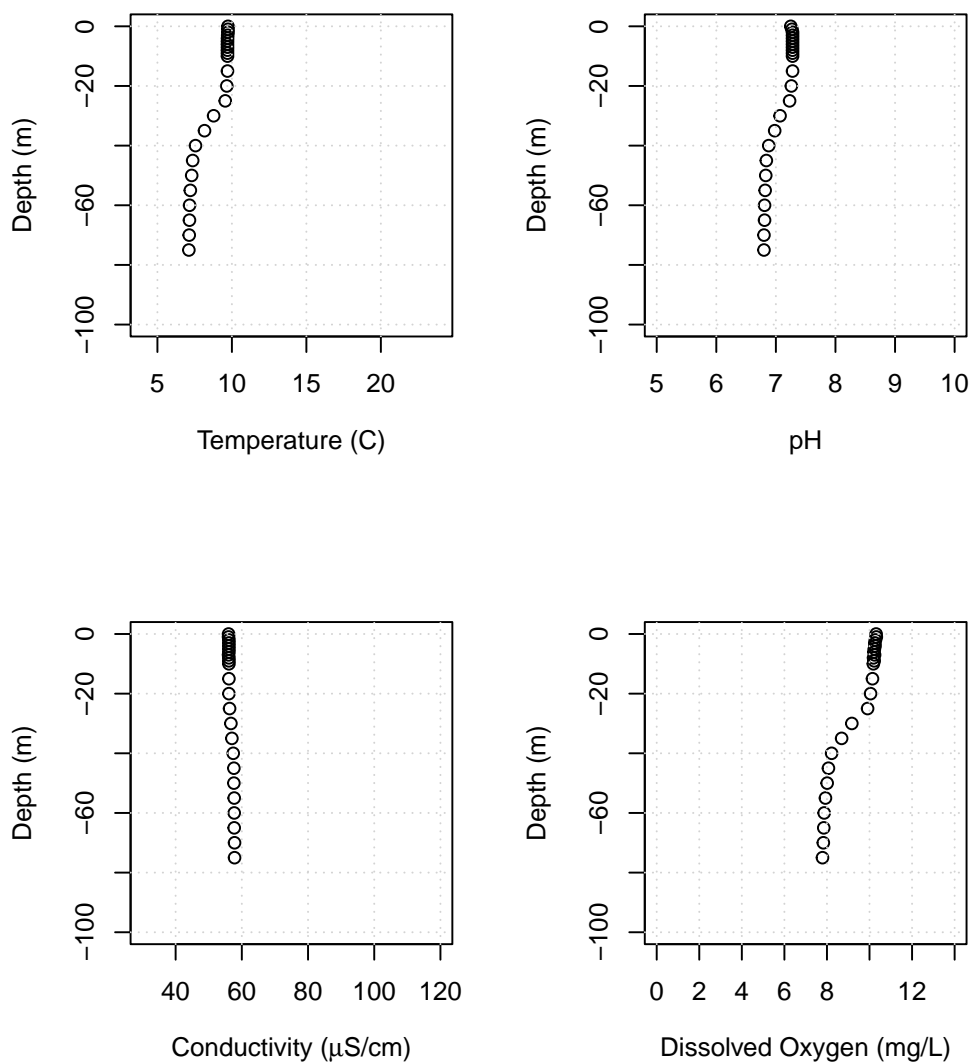
Figure B64: Lake Whatcom water column profiles showing temperature, pH, conductivity, and dissolved oxygen for Site 3, December 2, 2021.
