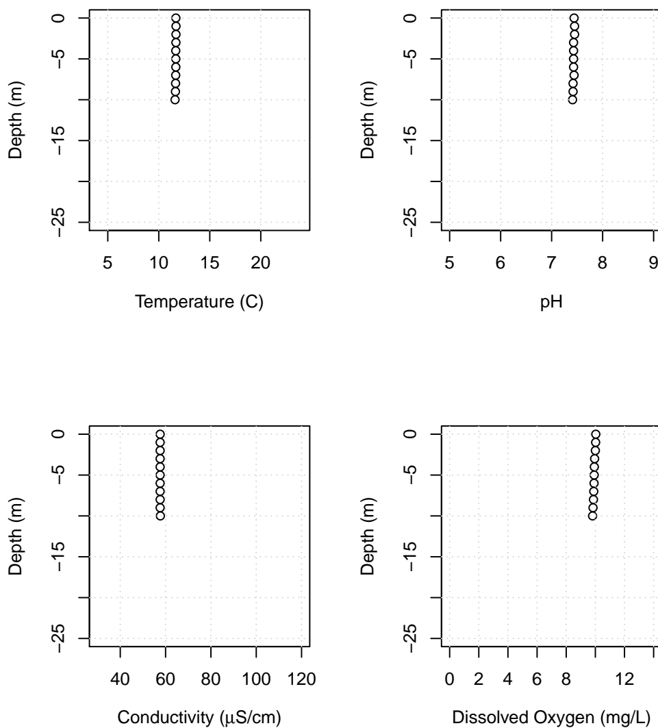
Figure B8: Lake Whatcom water column profiles showing temperature, pH, conductivity, and dissolved oxygen for the Intake, November 9, 2020.
