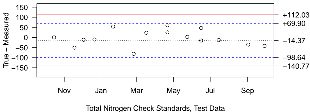
Figure C17: Nitrogen (total) high-range check standards for the Lake Whatcom monitoring program. Upper/lower acceptance limits ( \pm 2 std. dev. from mean pair difference) and upper/lower warning limits ( \pm 3 std. dev. from mean pair difference) were calculated based on the preceding two years of check standard data.
