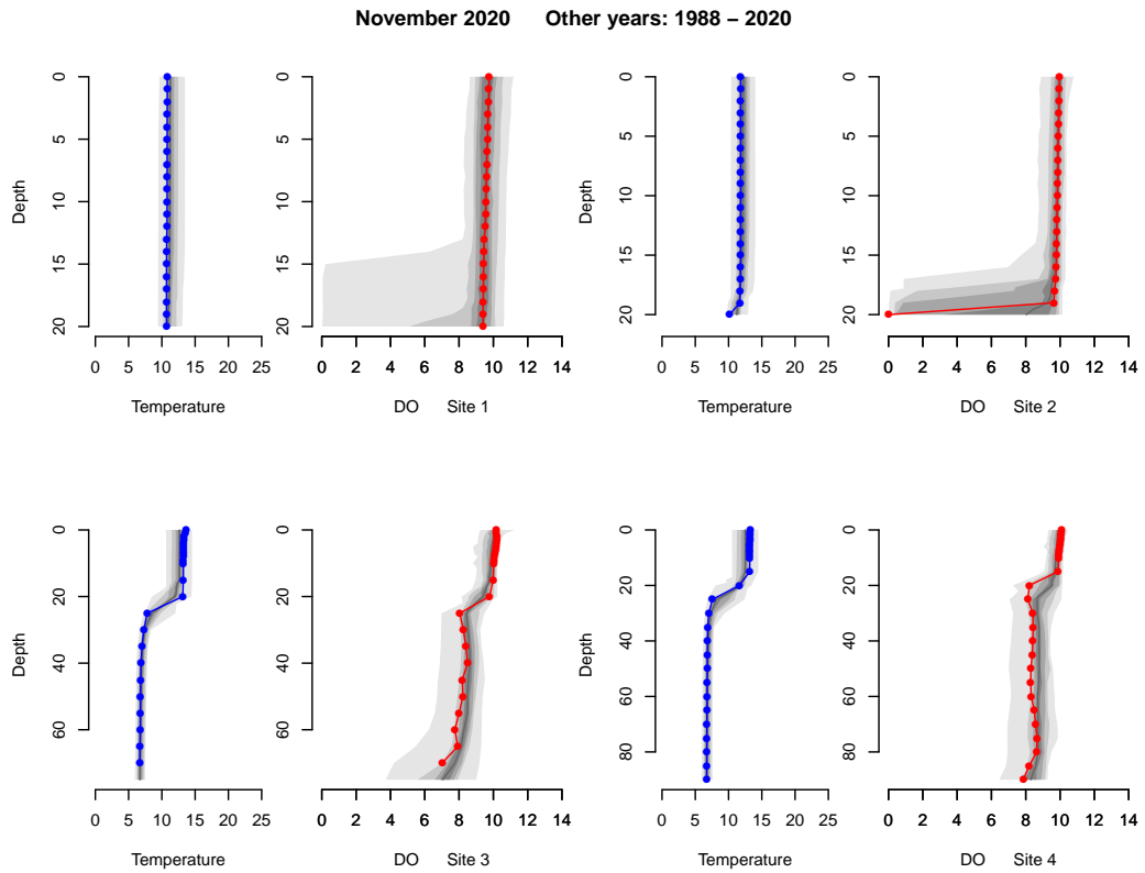
Figure 2.2: November 2020 temperature (-●-) and dissolved oxygen (-●-) profiles compared to historic ranges. The gradation in shading shows the approximate frequency of the 1988–2020 data.
