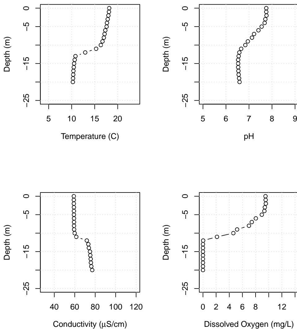
Figure B1: Lake Whatcom water column profiles showing temperature, pH, conductivity, and dissolved oxygen for Site 1, October 7, 2020.
