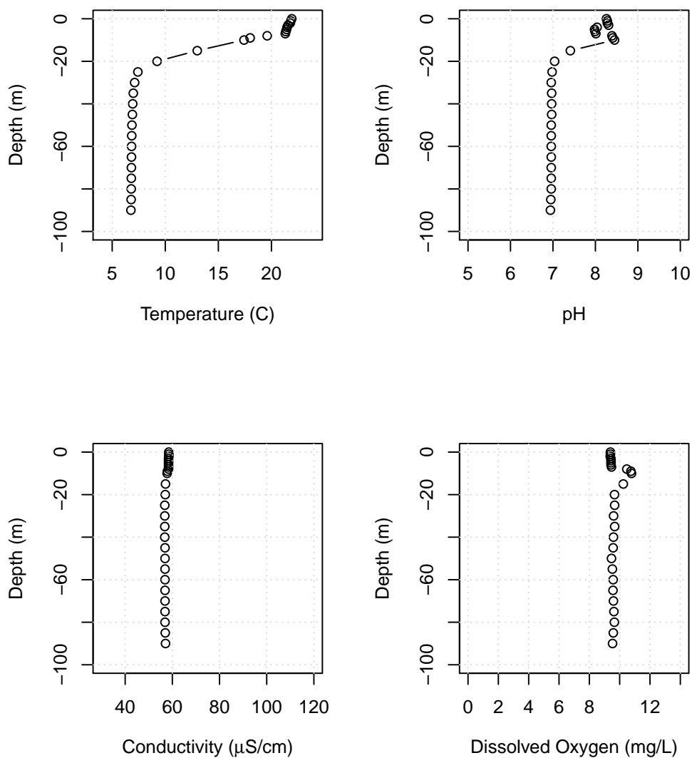
Figure B40: Lake Whatcom water column profiles showing temperature, pH, conductivity, and dissolved oxygen for Site 4, July 6, 2021.
