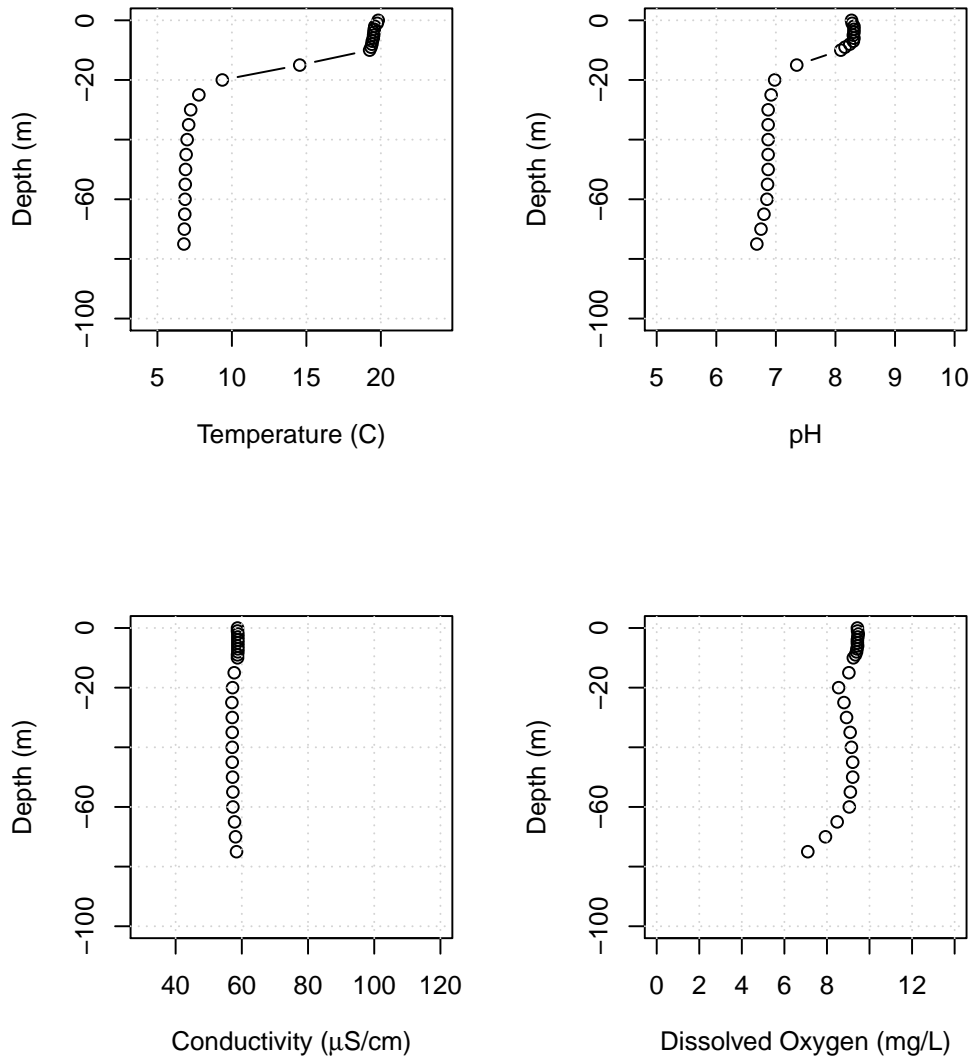
Figure B49: Lake Whatcom water column profiles showing temperature, pH, conductivity, and dissolved oxygen for Site 3, September 7, 2021.
