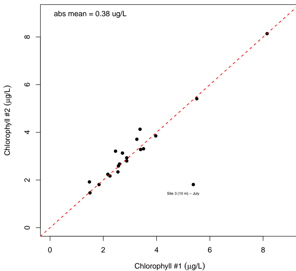
Figure C33: Chlorophyll field duplicates for the 2020/2021 Lake Whatcom monitoring program (lake samples). Diagonal reference line shows 1:1 relationship. The outlier identified likely represents slight differences in sample depth of the field duplicate near the steep thermocline.
