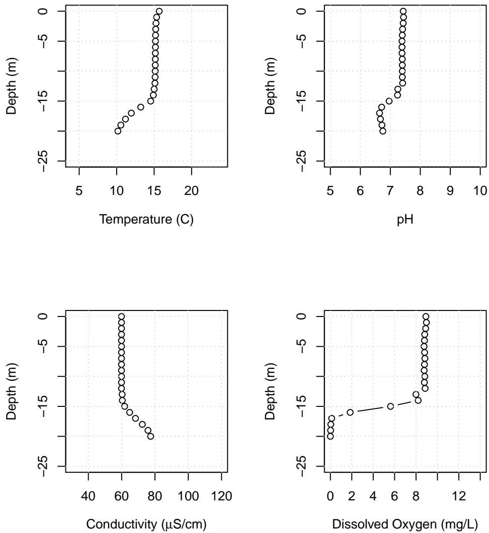
Figure B51: Lake Whatcom water column profiles showing temperature, pH, conductivity, and dissolved oxygen for Site 1, October 7, 2021.
