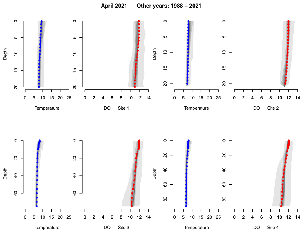
Figure 2.5: April 2021 temperature (-●-) and dissolved oxygen (-●-) profiles compared to historic ranges. The gradation in shading shows the approximate frequency of the 1988–2021 data.
