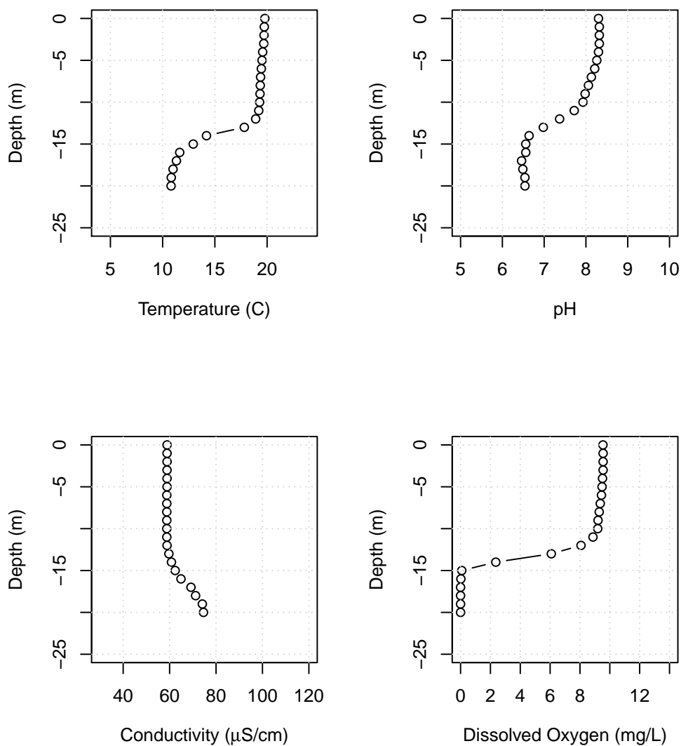
Figure B47: Lake Whatcom water column profiles showing temperature, pH, conductivity, and dissolved oxygen for Site 2, September 9, 2021.
