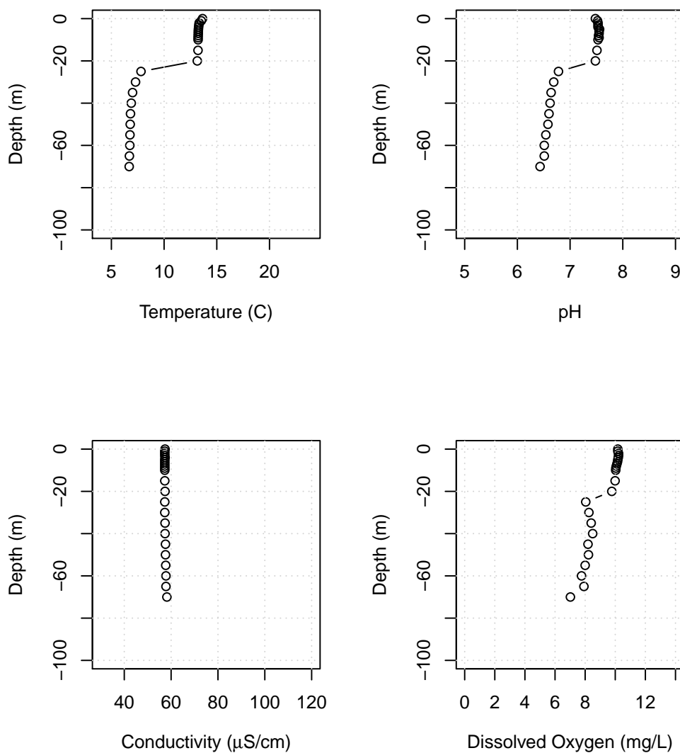
Figure B9: Lake Whatcom water column profiles showing temperature, pH, conductivity, and dissolved oxygen for Site 3, November 2, 2020.
