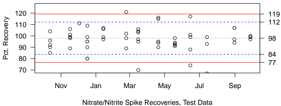
Figure C12: Nitrogen (nitrate/nitrite) spike recoveries for the Lake Whatcom monitoring program. Upper/lower acceptance limits ( \pm 2 std. dev. from mean pair difference) and upper/lower warning limits ( \pm 3 std. dev. from mean pair difference) were calculated based on the preceding two years of spike data.
