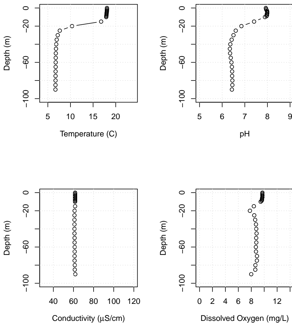
Figure B5: Lake Whatcom water column profiles showing temperature, pH, conductivity, and dissolved oxygen for Site 4, October 5, 2020.
