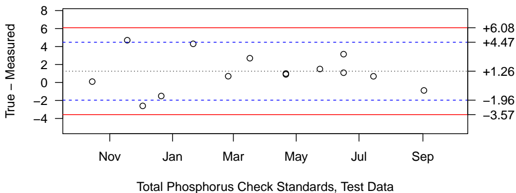
Figure C26: Phosphorus (total) high-range check standards for the Lake Whatcom monitoring program. Upper/lower acceptance limits ( \pm 2 std. dev. from mean pair difference) and upper/lower warning limits ( \pm 3 std. dev. from mean pair difference) were calculated based on the preceding two years of check standard data.
