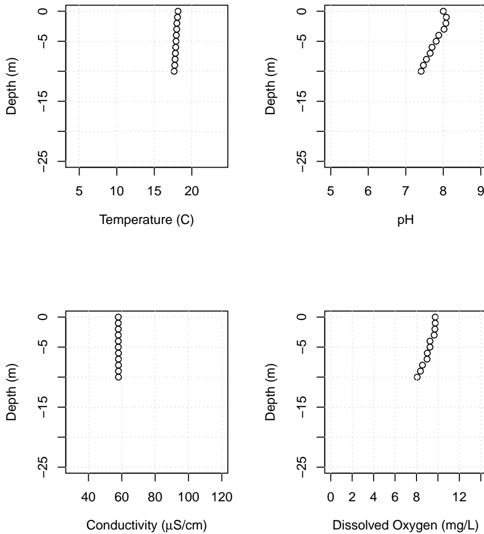
Figure B3: Lake Whatcom water column profiles showing temperature, pH, conductivity, and dissolved oxygen for the Intake, October 7, 2020.
