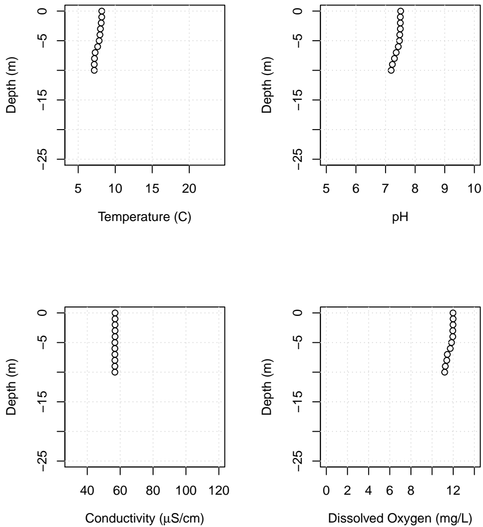
Figure B23: Lake Whatcom water column profiles showing temperature, pH, conductivity, and dissolved oxygen for the Intake, April 8, 2021.
