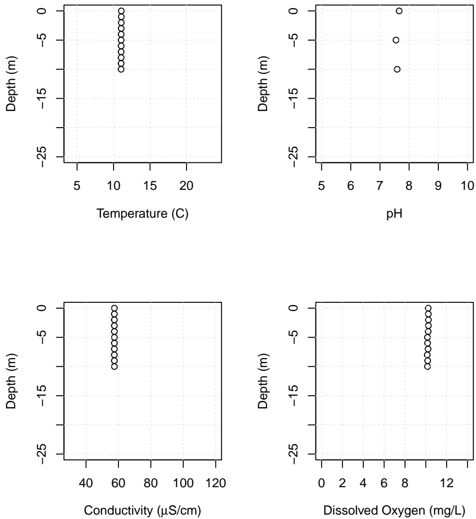
Figure B58: Lake Whatcom water column profiles showing temperature, pH, conductivity, and dissolved oxygen for the Intake, November 9, 2021.
