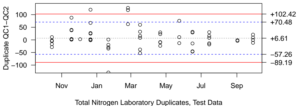
Figure C15: Nitrogen (total) laboratory duplicates for the Lake Whatcom monitoring program. Upper/lower acceptance limits ( \pm 2 std. dev. from mean pair difference) and upper/lower warning limits ( \pm 3 std. dev. from mean pair difference) were calculated based on the preceding two years of lab duplicate data.
