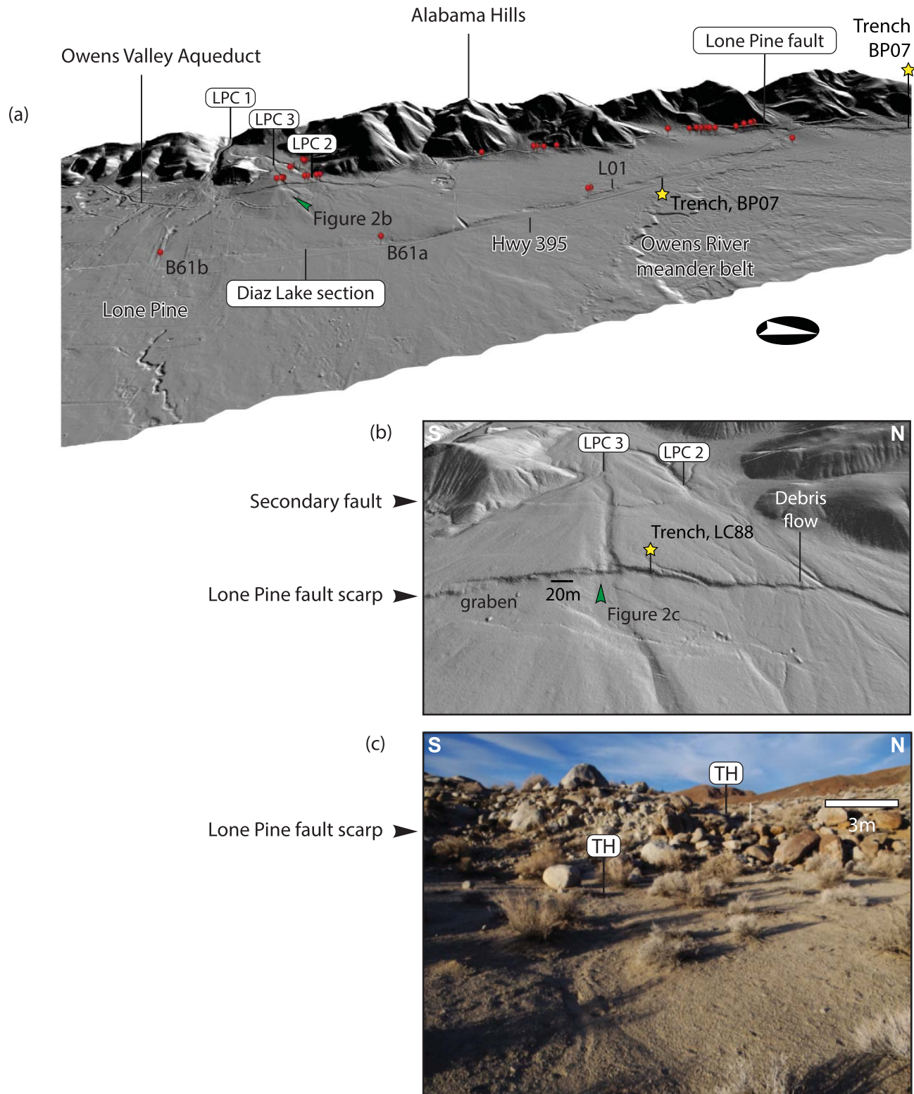
Figure 2. Oblique view of hillshade image derived from EarthScope lidar data. (a) View towards the northwest of the Alabama Hills and the southern Owens Valley fault zone, including the Diaz Lake section (east) and the Lone Pine fault (west). Offset features (red markers) include new measurements and sites described in Bateman [1961] (B61), Lubetkin and Clark [1988] (LC88), and Bacon and Pezzopane [2007] (yellow stars, BP07). LPC1, LPC2, and LPC3—Lone Pine Creek 1, 2, and 3. (b) Hillshade image of the faulted Lone Pine fan (Lone Pine, CA) showing right-oblique separation of debris-flow channels and fan axes [ Lubetkin and Clark , 1988; Beanland and Clark , 1994]. (c) View to the west of the offset thalweg (TH) of southern Lone Pine Creek (LPC3) first identified by W. D. Johnson in Hobbs [1910].
