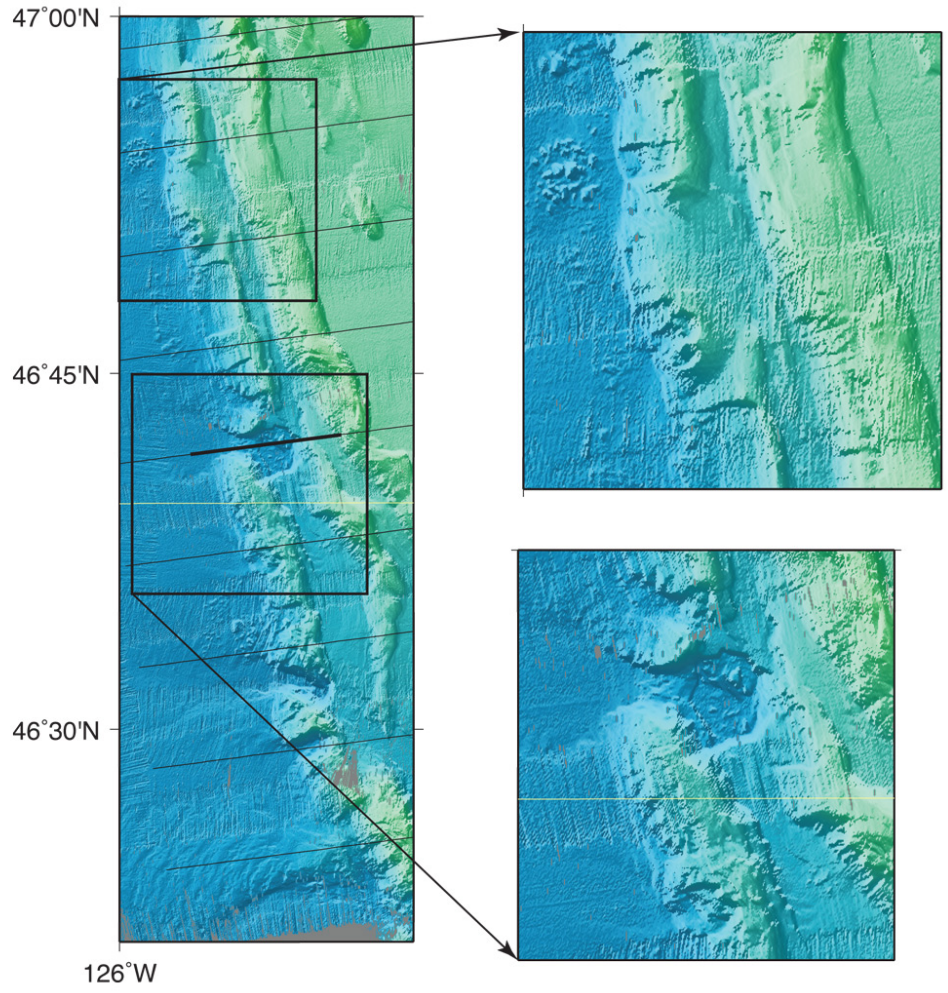
Figure S2. Multibeam bathymetry over the deformation front in the COAST survey area. Seismic lines (1-9) are shown as thin lines. Zooms of collapse features are shown top right and bottom right.
