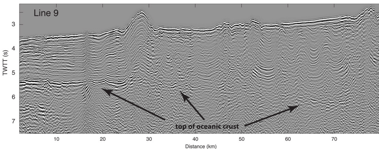
Figure S1. Time migrated section showing the deformation front and accretionary prism on Line 9, at the south end of the COAST survey. Note the reflections from the top of oceanic crust, and the uniformly folded sediments in the prism from 55–75 km. The vertical feature near 16 km is a processing artifact, resulting from a short shut-down of the airguns due to a marine mammal sighting.
