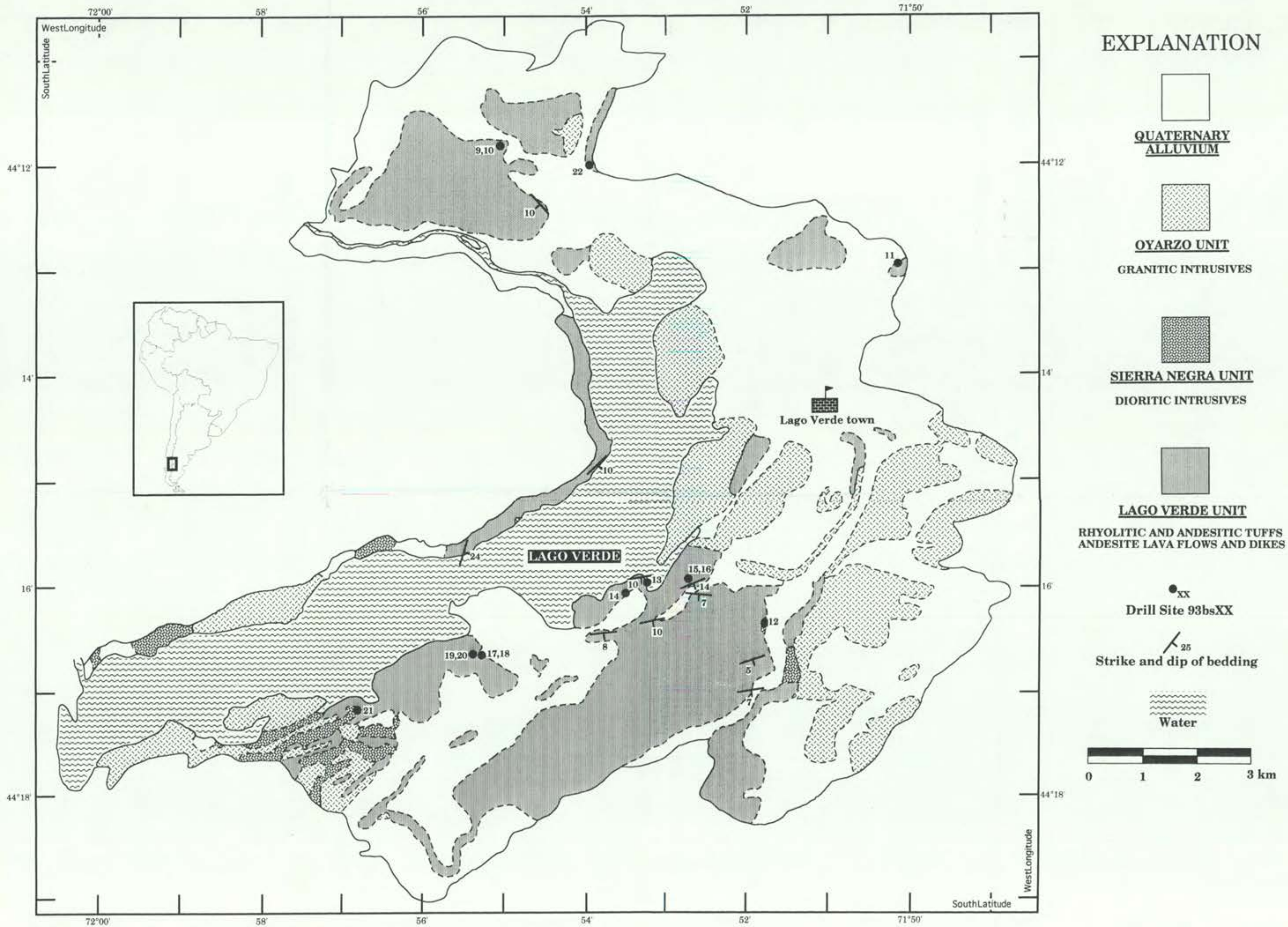
Figure 2.3 Geological map of the Lago Verde field area showing rock units, structural data, and location of paleomagnetic sample sites.
