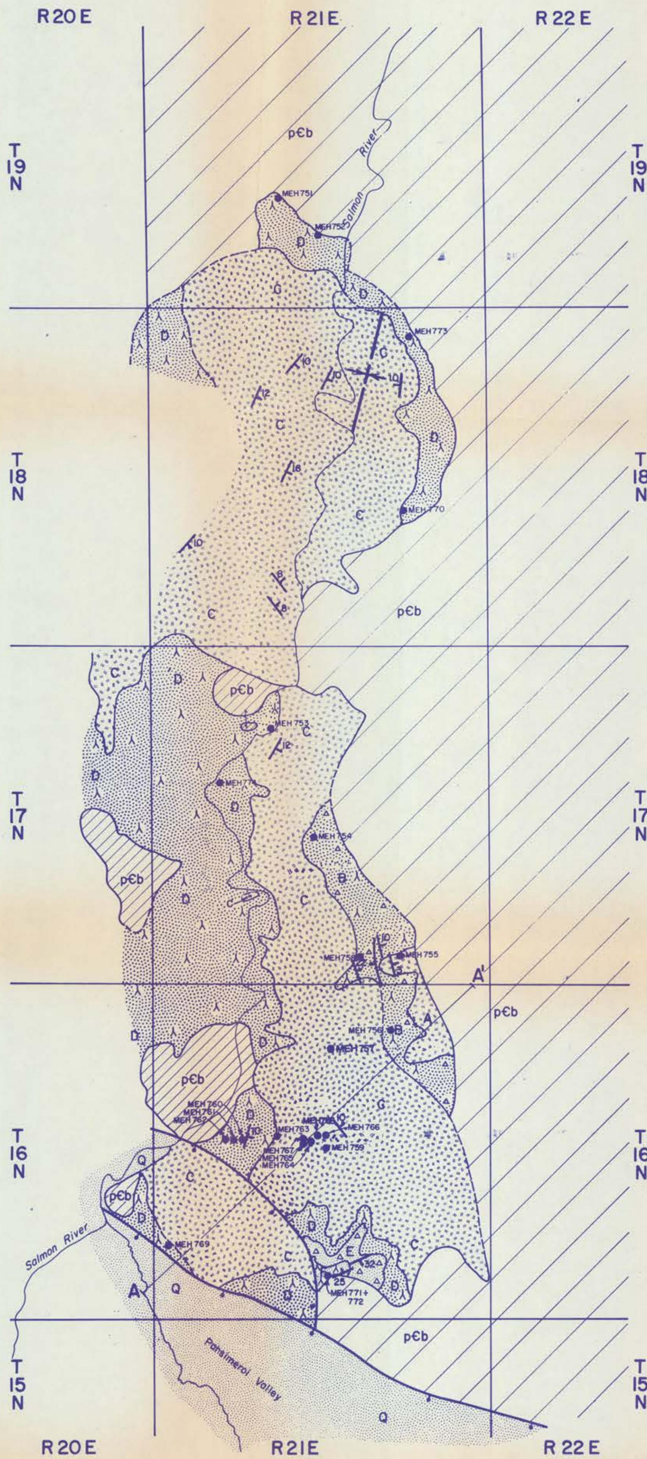
FIGURE 15. GEOLOGIC MAP AND CROSS-SECTION OF SALMON RIVER VALLEY AND PAHSIMEROI RIVER VALLEY, NORTH OF MAY (AREA III).
