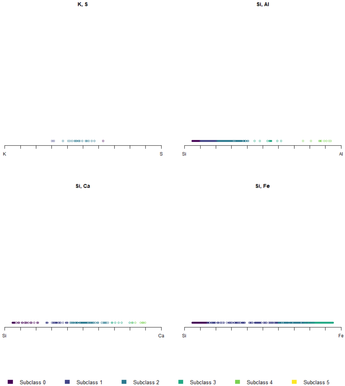
Figure S1. Particle class and subclass composition. Particle classes are displayed above each figure. Each point represents a particle, arranged by composition and colored by subclass. The source classes and occurrences of common subclasses ( n > 10 ) are listed in Appendix B.
