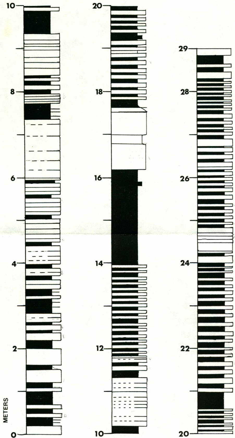
Plate 4. Partial stratigraphic section of the Hoko River Formation, Elwah River Rappel section.
