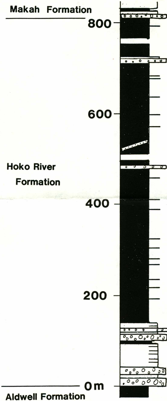
Plate 5. Stratigraphic section of the Hoko River Formation at Morse Creek. De Chant, 1989
