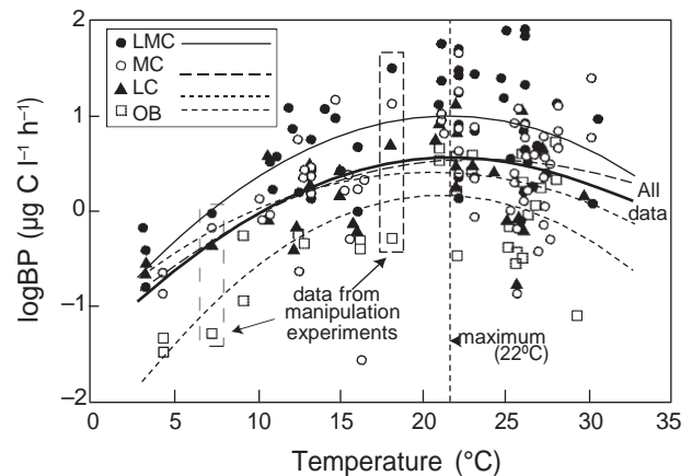
Fig. 4. Relationship between bacterioplankton production (BP) and temperature in each of the estuarine sub-systems of Monie Bay (i.e. LMC: Little Monie Creek; MC: Monie Creek; LC: Little Creek; OB: open bay). The inflection point of the second order polynomial describing the temperature response of the entire dataset (i.e. 22^\circ\text{C} ) is indicated by the vertical dotted line. Data from temperature manipulation experiments are indicated by enclosures
