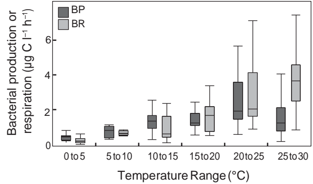
Fig. 3. Box and whisker plots of median bacterial production (BP) and respiration (BR) at discrete temperature ranges throughout the year. Quartiles represented are 10, 25, 75, and 90%
