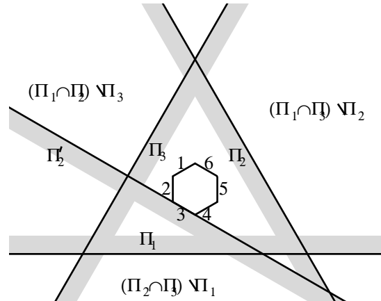
Fig. 3 Half-planes \Pi_1, \Pi_2, \Pi_3 and \Pi'_2 (of type 3) in proof of Lemma 15. Minimal region shown (hexagon) is surrounded by half-planes of types 1–6.
